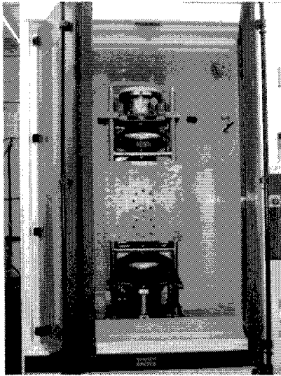
Figure 2. The closed chemistry, BCP, cabinet is used to acid etch the inner surface of the cavity at a controlled etch rate and temperature.
