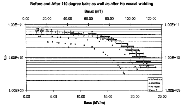
Figure 6. The plot of Q_0 vs E_{acc} for three tests on the 5 cell cavity. The blue circles are before the 110 degree bake, the red triangles are after the 110 degree bake and the red squares are with the He vessel attached.
