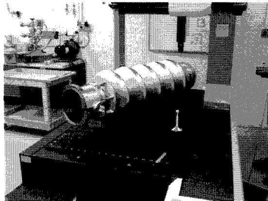
Figure 1. Dimensional Analysis on the CMM machine, the cavity needed to be placed on an angle due to its size.
