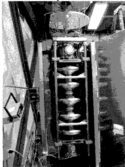
Figure 4. The low temperature bake-out box used for the 5 cell cavity 110 degree bake.
