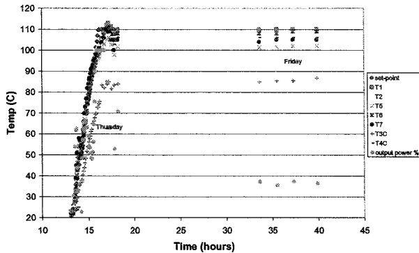
Figure 5. A plot of the thermocouple readout during the low temperature cavity bake. All thermocouples placed inside the box were within 5 degrees of one another.
