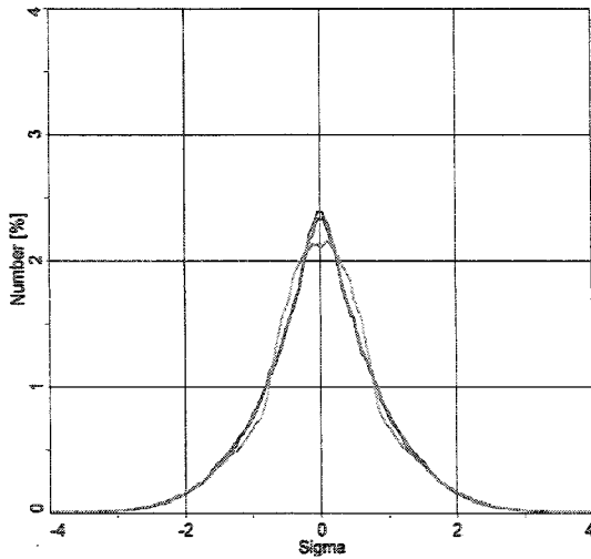
Figure 2: Horizontal (red), vertical (blue) and longitudinal (green) ion beam profiles after 5 minutes of cooling based on velocity distribution shown in Fig. 1.
