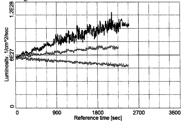
Figure 4: Initial luminosities. Black – using electron distribution at the start of the cooling section. Red (based on the local model) and blue (based on global parameters) using distribution at the end of the cooling section.
