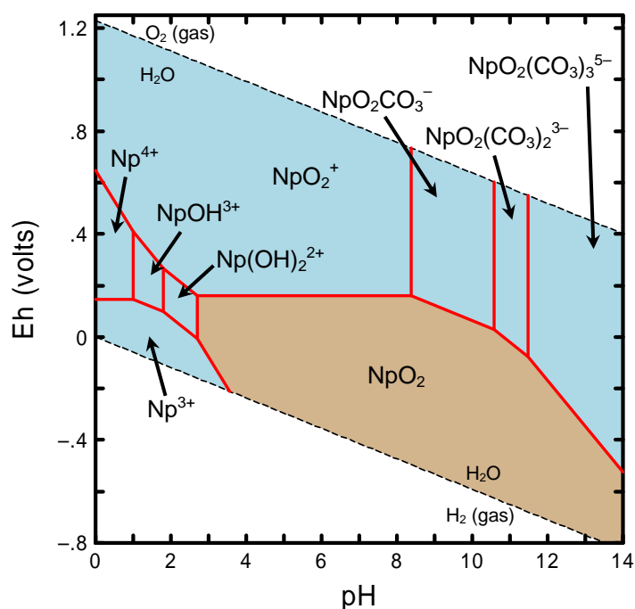
Figure A.7. Diagram Showing Eh-pH Region (Tan Colored) that Calculates to be Oversaturated with Respect to the Solubility of Neptunium Solids. (Diagram was calculated at a total activity of 1 \times 10^{-16} M dissolved neptunium at 25°C.)
