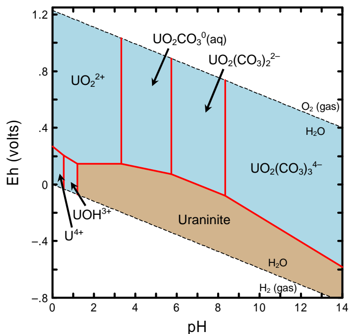
Figure A.18. Diagram Showing Eh-pH Region (tan colored) that Calculates to be Oversaturated with Respect to the Solubility of Uraninite (UO 2 ) (Diagram was calculated at a total activity of 1 \times 10^{-9} M dissolved uranium at 25°C.)
