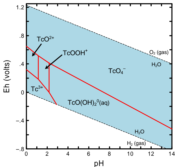
Figure A.15. Eh-pH Diagram Showing Dominant Aqueous Species of Technetium. (Diagram was calculated at a total activity of 1 \times 10^{-7.5} M dissolved technetium at 25°C.)
