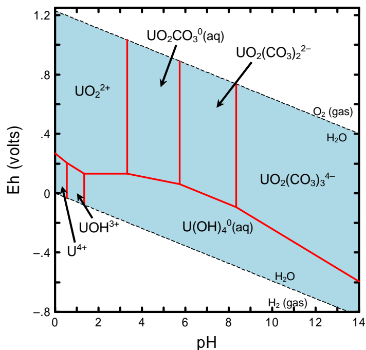
Figure A.17. Eh-pH Diagram Showing Dominant Aqueous Species of Uranium (Diagram was calculated at a total activity of 1 \times 10^{-8} M dissolved uranium at 25^\circ\text{C} .)
