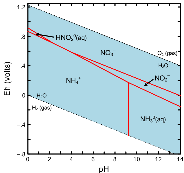
Figure A.8. Eh-pH Diagram Showing Dominant Aqueous Species of Nitrogen. (Diagram was calculated at a total activity of 1 \times 10^{-2} M dissolved nitrogen at 25°C.)
