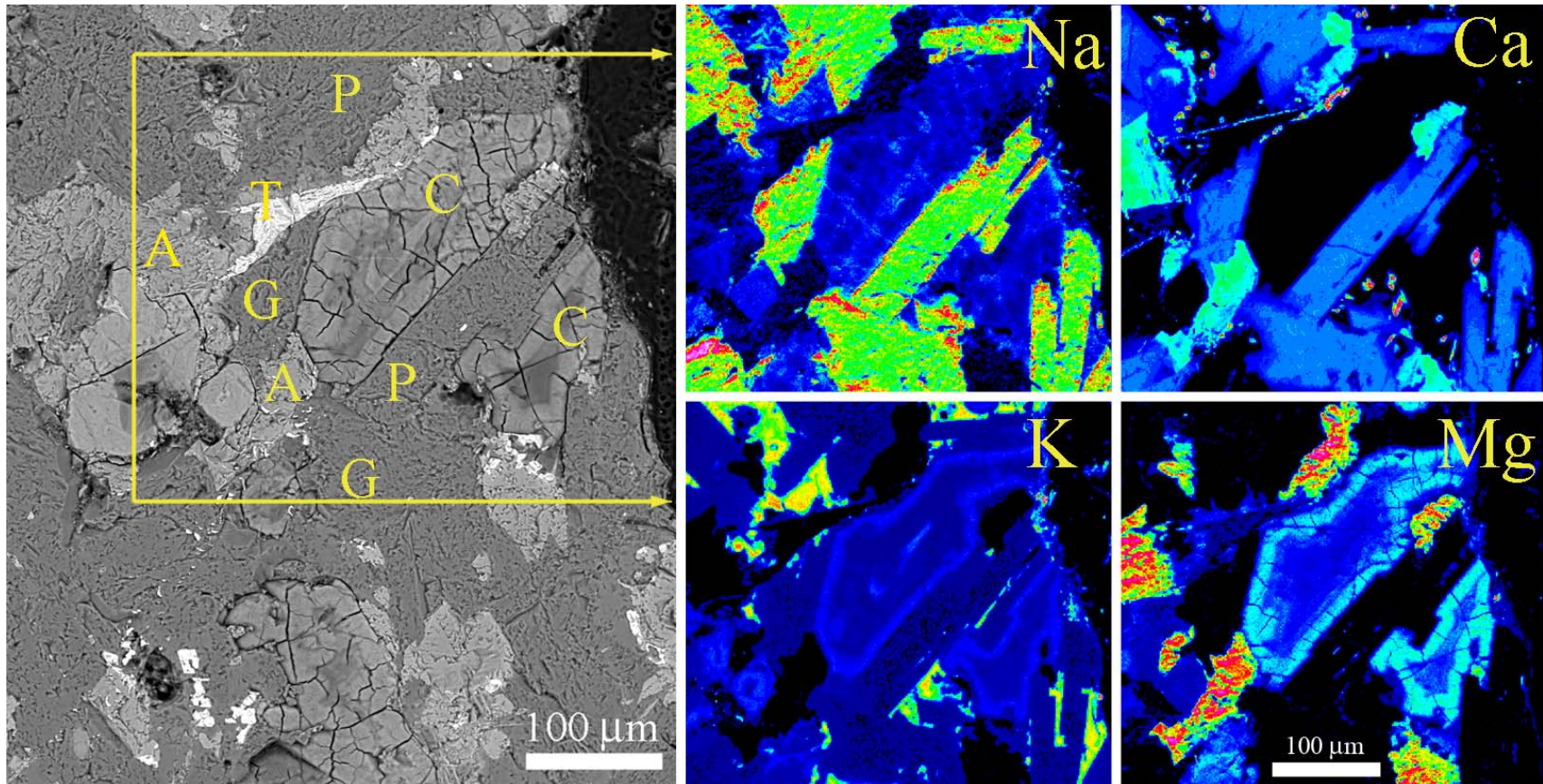
Figure 6.6. Scanning Electron Microscope Backscattered Electron Image (left) and Maps of Relative Elemental Abundances (colorized images at right) for Sodium (Na), Calcium (Ca), Potassium (K), and Magnesium (Mg) for ^{90}\text{Sr} -Containing Area of Smectite Inclusions Indicated by White Arrow in Figure 3.5. Elemental abundances are shown in false color where blue indicates regions of lowest abundance and red indicates highest abundance in a rainbow progression. All are secondary phyllosilicate domains (saponites-C) showing the characteristic Mg-zonation (Source: McKinley et al. 2006).
