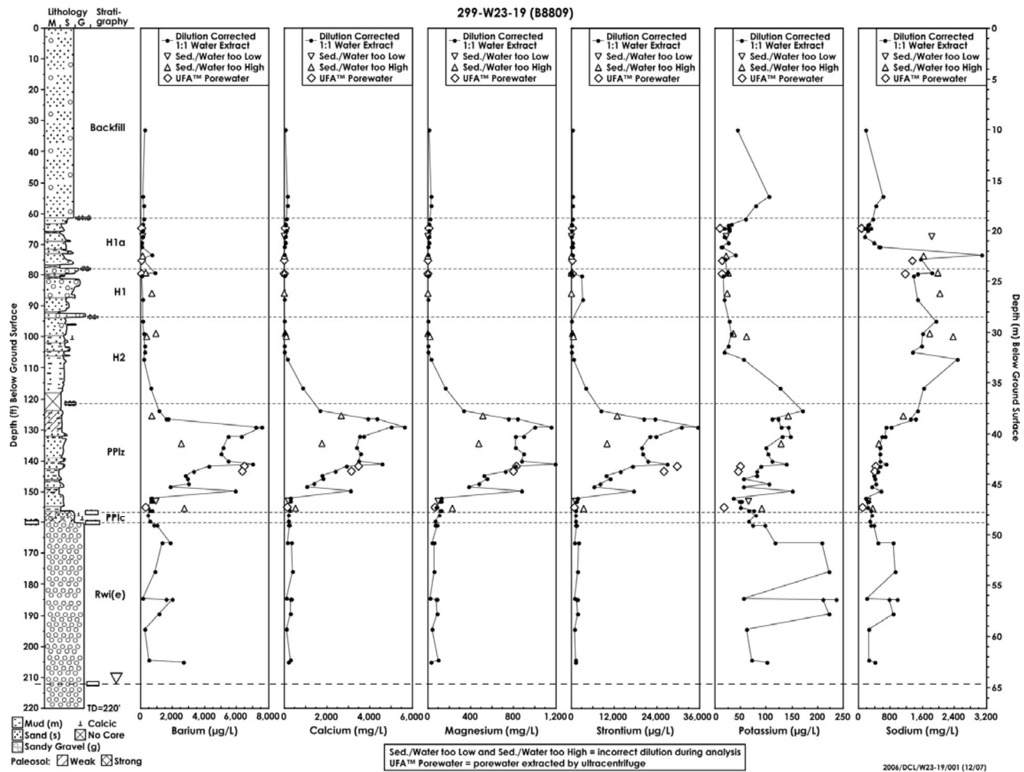
Figure 6.4. Depth Distribution of Water-Extractable Ions in Sediment Beneath Leaked Single-Shell Tank SX-115. Note the tank waste front at 150 ft (45.8 m) below ground surface. Tank SX-115 released waste of intermediate composition (Source: Serne et al. 2002a)
