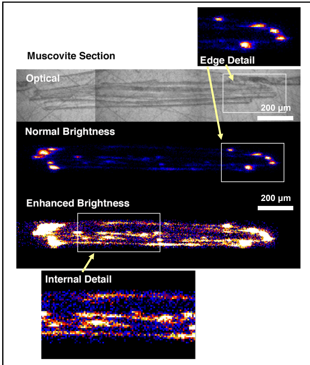
Figure 6.7. Distribution of Cesium Within a Flake (shown on edge) of the Mineral Muscovite from a Sediment Sample Collected Beneath the WMA S-SX as Measured by Synchrotron X-Ray Fluorescence. Cesium is strongly localized at selected regions on the crystallite edge. Cesium abundance is shown in false color where highest concentrations of cesium are indicated by the brightest areas (Source: Liu et al. 2003a).
