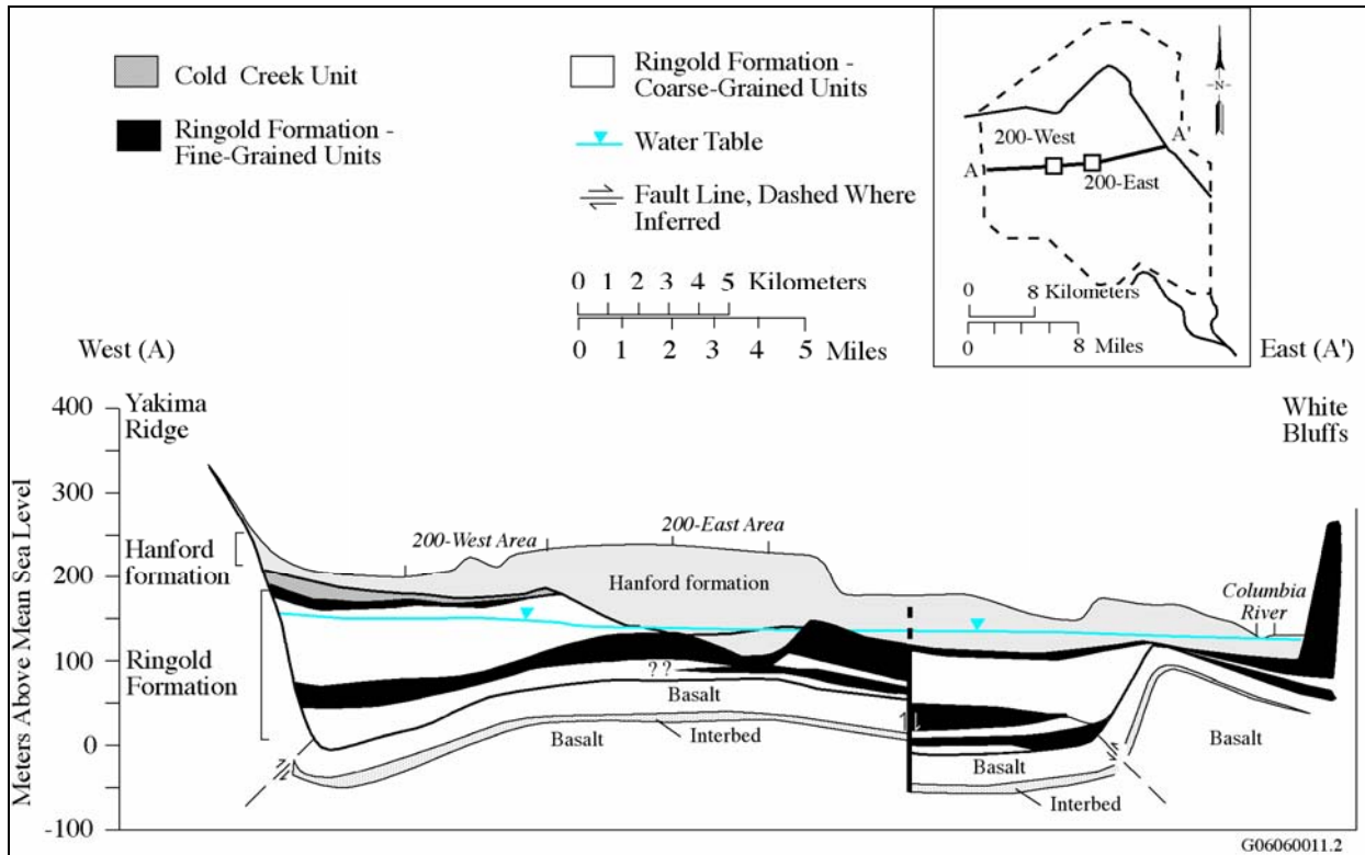
Figure 3.3. Generalized Cross Section Through the Hanford Site (Source: Reidel and Chamness 2007)
