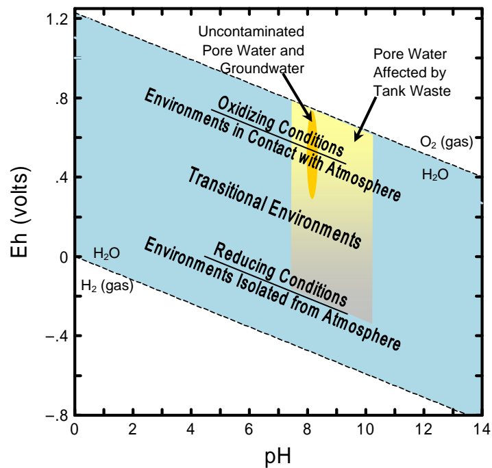
Figure 5.1. Approximate Position of Some Natural Environments as a Function of pH and Eh Conditions. (Dark yellow area shows general Eh-pH regions expected for pore water from vadose zone and groundwater from the upper unconfined aquifer not affected by waste release. Light yellow shaded area shows expected Eh-pH region for vadose zone pore water that was influenced by tank waste.)
