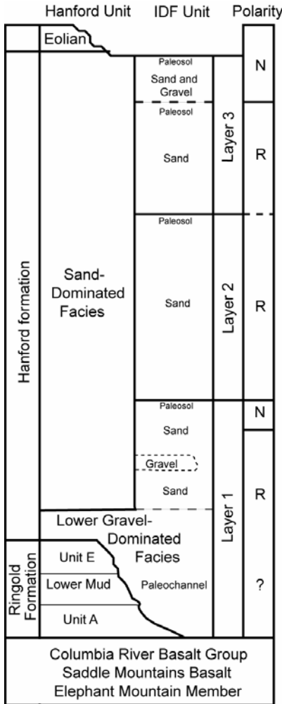
Figure 3.5. Stratigraphy Below the Integrated Disposal Facility (Source: Reidel and Chamness 2007)
