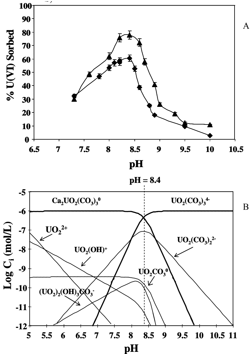
Figure 6.2. A)(top) Adsorption of \mu\text{mol/L} U(VI) on a Calcite-Containing, Deep Vadose Zone Sediment (100 g/L) from Hanford Site's 200 Area Plateau (WMA S-SX), P_{\text{CO}_2} = 10^{-3.5} \blacklozenge = untreated sediment; \blacktriangle = sediment with calcite removed. B)(bottom) Computed Aqueous Speciation of U(VI) in Calcite-Saturated 0.05 mol/L NaNO 3 (Source: Dong et al. 2005)
