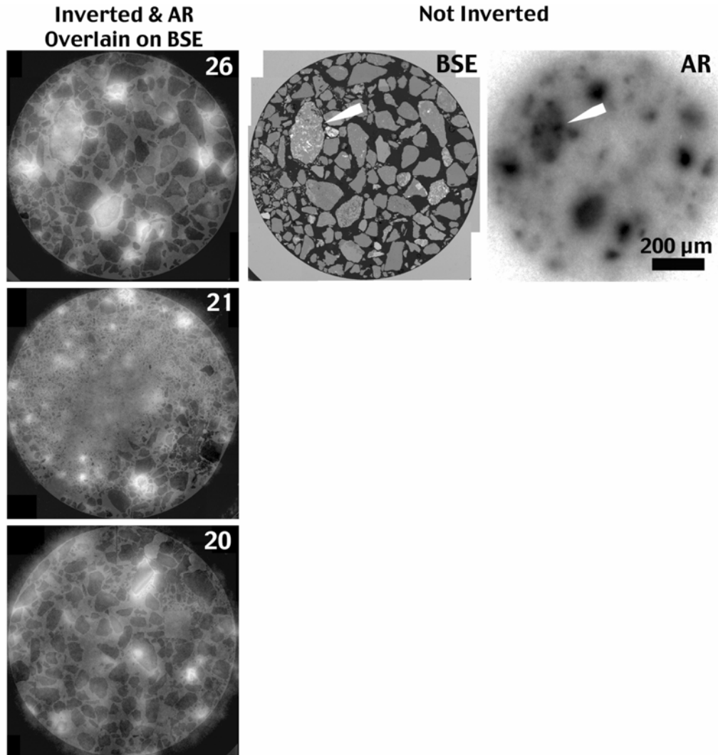
Figure 6.5. Scanning Electron Microscope Backscattered Electron Image (BSE) and Autoradiographs (AR) Showing Distribution of ^{90}\text{Sr} in Contaminated Sediment Samples 20A, 21A, and 26A from Borehole 299-E33-46 near Tank B-110 (Source: McKinley et al. 2007). Lithic fragments containing ^{90}\text{Sr} are white in inverted ARs (samples 20A, 21A, and 26A), or black in ARs not inverted (sample 26A only).
