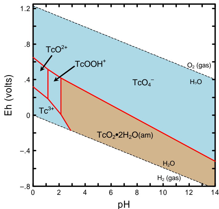
Figure A.16. Diagram Showing Eh-pH Region (Tan Colored) that Calculates to be Oversaturated with Respect to the Solubility of Technetium Solids. (Diagram was calculated at a total activity of 1 \times 10^{-7.5} M dissolved technetium at 25°C.)
