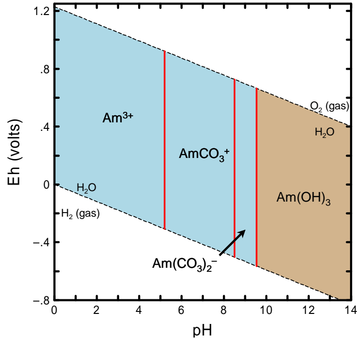
Figure A.2. Diagram Showing Eh-pH Region (tan colored) that Calculates to be Oversaturated with Respect to the Solubility of \text{Am}(\text{OH})_3 . (Diagram was calculated at a total activity of 1 \times 10^{-8} M dissolved americium at 25^\circ\text{C} .)
