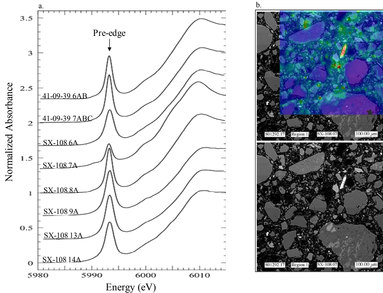
Figure 6.9. Field Samples from Beneath Tank SX-108. (a) XANES Spectra of Chromium-Contaminated Sediment from SX-108 Borehole C3082 where the Height of the Pre-Edge Feature is Proportional to the Cr(VI) Content (Source: Zachara et al. 2004). (b) Synchrotron X-ray Fluorescence Map (top right) of SX-108 Sediment 7A, Overlain on a SEM BSE micrograph. Grains colored green to red indicates high-chromium concentrations.
