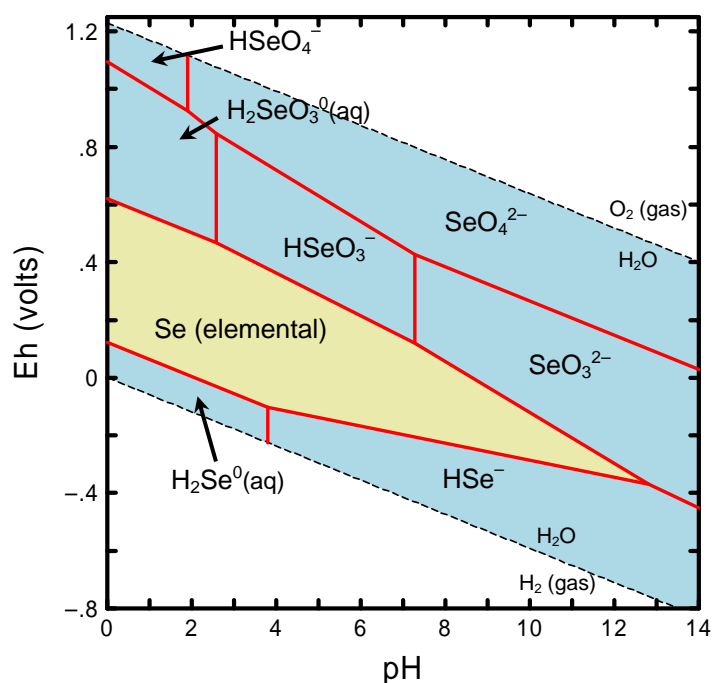
Figure A.12. Diagram Showing Eh-pH Region (tan colored) that Calculates to be Oversaturated with Respect to the Solubility of Elemental Selenium. (Diagram was calculated at a total activity of 1 \times 10^{-8} M dissolved selenium at 25^\circ\text{C} .)
