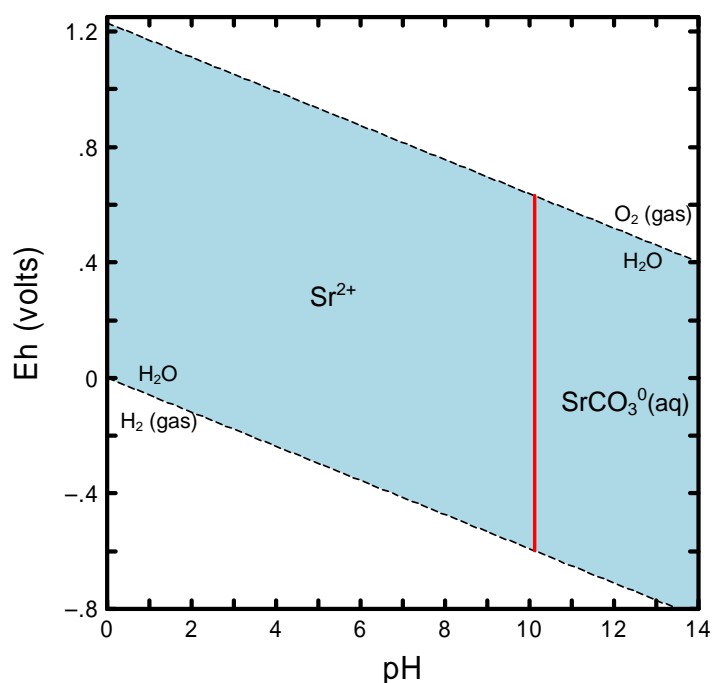
Figure A.13. Eh-pH Diagram Showing Dominant Aqueous Species of Strontium. (Diagram was calculated at a total activity of 1 \times 10^{-8} M dissolved strontium at 25°C.)
