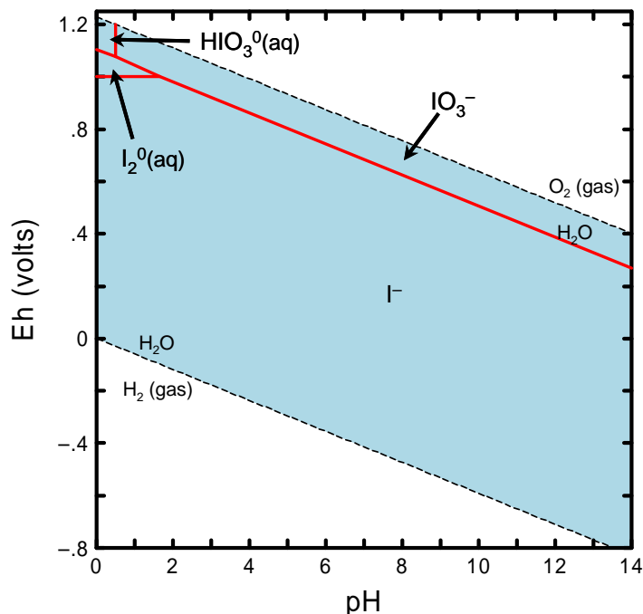
Figure A.5. Eh-pH Diagram Showing Dominant Aqueous Species of Iodine. (Diagram was calculated at a total activity of 1 \times 10^{-8} M dissolved iodine at 25°C.)
