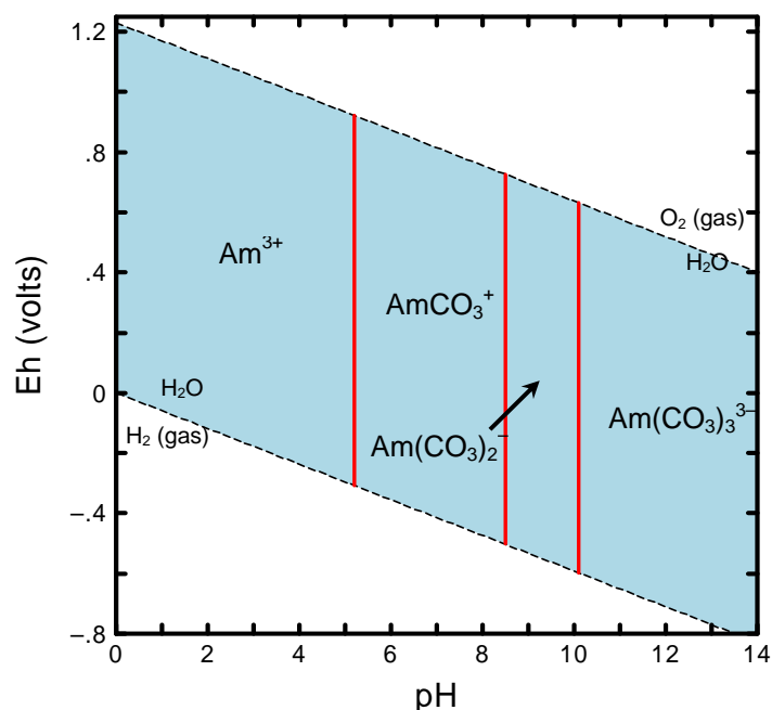
Figure A.1. Eh-pH Diagram Showing Dominant Aqueous Species of Americium. (Diagram was calculated at a total activity of 1 \times 10^{-8} M dissolved americium at 25^\circ\text{C} .)
