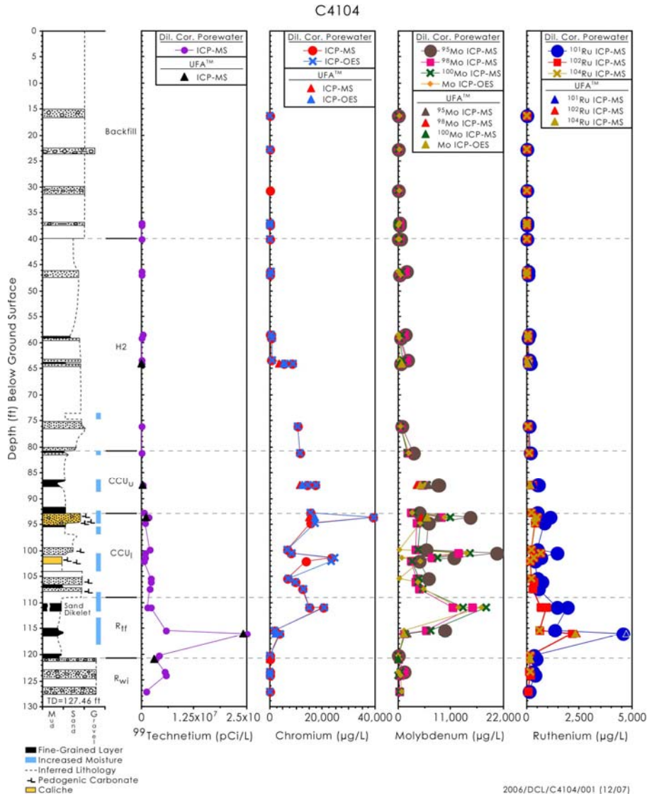
Figure 6.3. Derived and Actual Pore Water Concentrations of Mobile Metals in Borehole C4104 Collected Near T-106. The leading edge of the tank waste plume is defined by the peak in ^{99}\text{Tc} concentration (Source: Serne et al. 2004b.)
