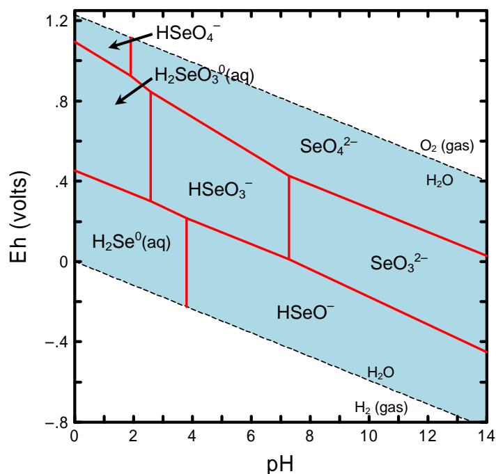
Figure A.11. Eh-pH Diagram Showing Dominant Aqueous Species of Selenium. (Diagram was calculated at a total activity of 1 \times 10^{-8} M dissolved selenium at 25^\circ\text{C} .)
