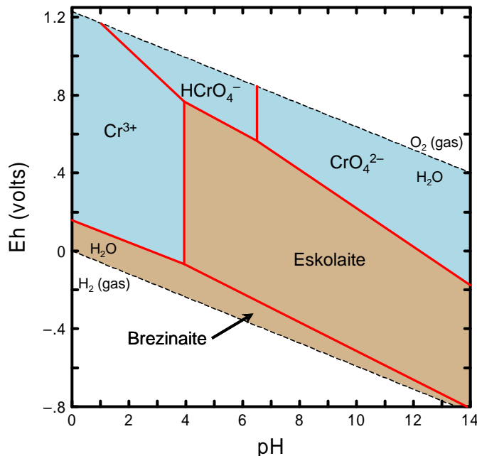
Figure A.4. Stability Diagram Showing Eh-pH Region (tan) that Calculates as Oversaturated with Respect to the Solubility of Cr(III) Solids. (Diagram was calculated at total activity of 1 \times 10^{-8} M dissolved chromium at 25^\circ\text{C} .)
