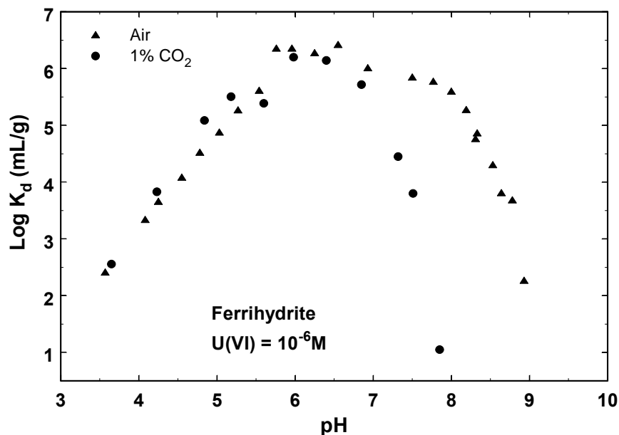
Figure 6.1. Adsorption of 1 \mu\text{mol/L} U(VI) on 1 mmol/L of Ferrihydrite, One of the Most Important Subsurface Sorbents of Uranium (Source: Davis et al. 2004)
