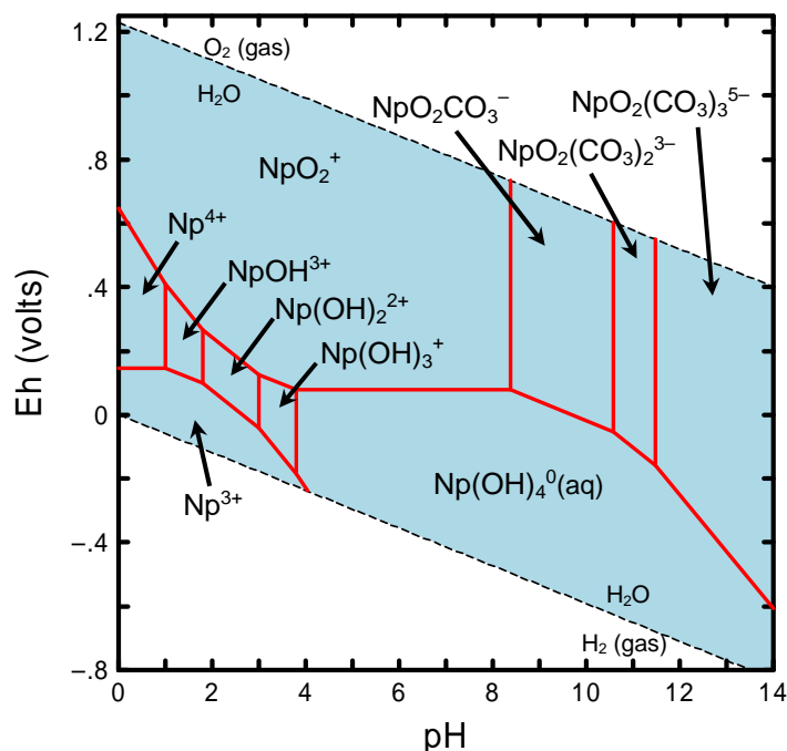
Figure A.6. Eh-pH Diagram Showing Dominant Aqueous Species of Neptunium. (Diagram was calculated at a total activity 1 \times 10^{-8} M dissolved neptunium at 25^\circ\text{C} .)
