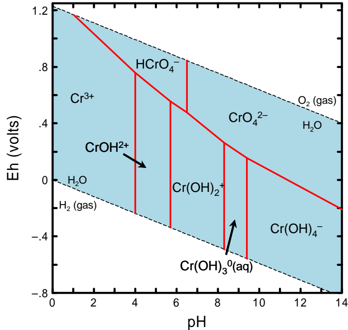
Figure A.3. Eh-pH Diagram Showing Dominant Aqueous Species of Chromium. (Diagram was calculated at a total activity of 1 \times 10^{-8} M dissolved chromium at 25°C.)
