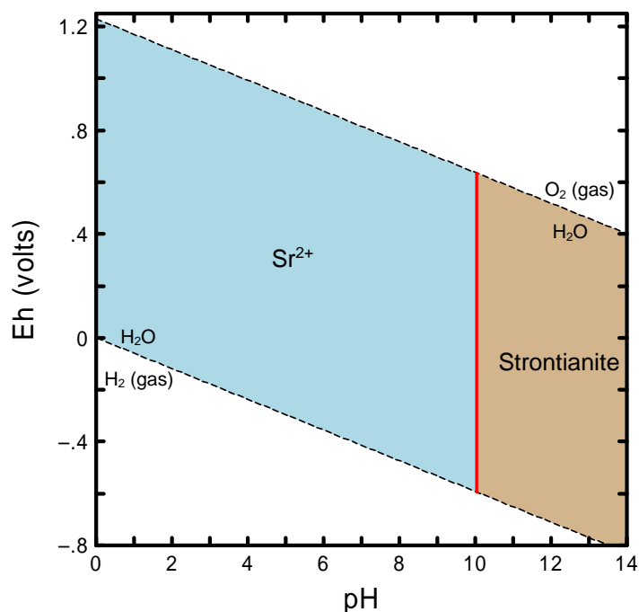
Figure A.14. Diagram Showing Eh-pH Region (tan colored) that Calculates to be Oversaturated with Respect to the Solubility of Strontianite ( \text{SrCO}_3 ). (Diagram was calculated at a total activity of 1 \times 10^{-7.7} M dissolved strontium at 25^\circ\text{C} .)
