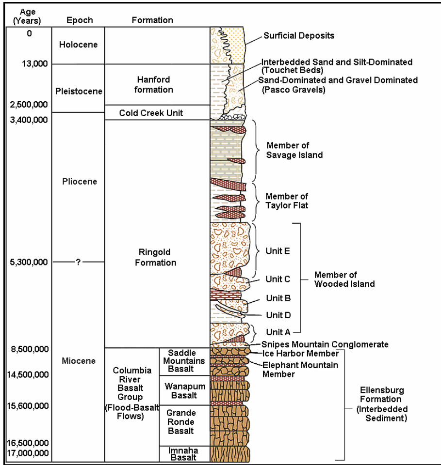
Figure 3.2. Generalized Stratigraphy of the Sediments (Hanford formation, Cold Creek Unit, and Ringold Formation) and Flood-Basalt Flows of the Pasco Basin and Vicinity (Source: Reidel and Chamness 2007)
