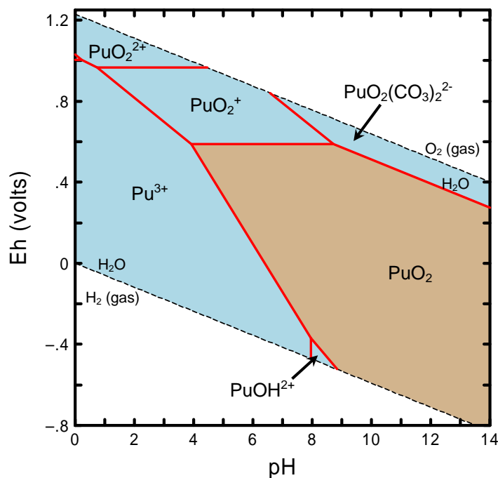
Figure A.10. Diagram Showing Eh-pH Region (tan colored) that Calculates to be Oversaturated with Respect to the Solubility of \text{PuO}_2 . (Diagram was calculated at a total activity of 1 \times 10^{-16} M dissolved plutonium at 25^\circ\text{C} .)
