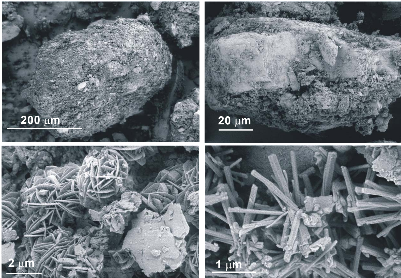
Figure 6.8. Scanning Electron Micrographs of Secondary Feldspathic Precipitates Resulting from the Reaction of \text{Na}^+/\text{NO}_3^-/\text{OH}^- Tank Waste Stimulant with Hanford Sediment. The dissolution of primary aluminosilicates and reprecipitation of various secondary phases neutralizes the high pH of tank waste (Source: Qafoku et al. 2003).
