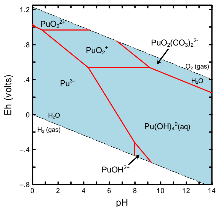
Figure A.9. Eh-pH Diagram Showing Dominant Aqueous Species of Plutonium. (Diagram was calculated at a total activity of 1 \times 10^{-8} M dissolved plutonium at 25^\circ\text{C} .)
