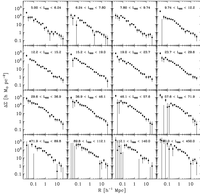
FIG. 10.— Same as Figure 7 but in 16 bins of L_{200} , the total i-band luminosity of ( > 0.4L_* ) galaxies within r_{200}^{gals} .
