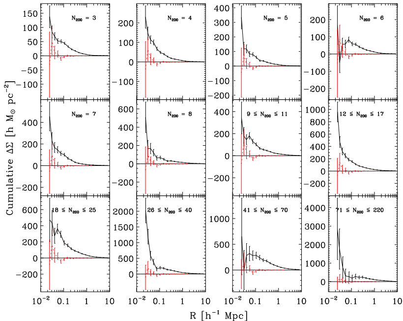
FIG. 13.— Mean estimated contamination of \Delta\Sigma from intrinsic alignments in each of the N_{200} bins, estimated as described in the text. These are cumulative curves so adjacent bins are correlated. In each panel, the intrinsic shear is the red curve and the cluster measurement is the black curve. Note the vertical scale varies between plots.
