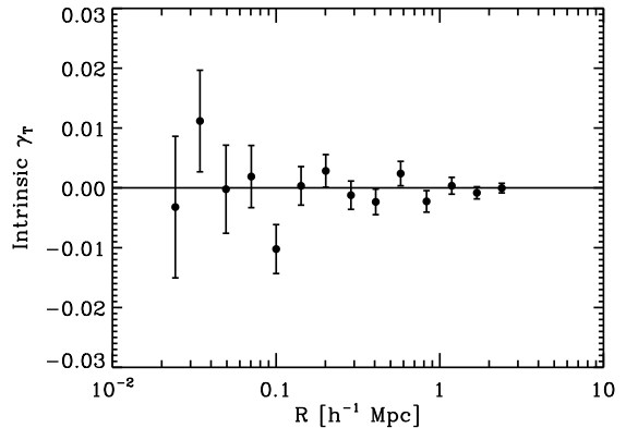
FIG. 12.— Estimate of intrinsic tangential alignments for the spectroscopic cluster sample of (Berlind et al. 2006). The shear tracer population was drawn from the SDSS main spectroscopic sample and chosen to have velocity within \pm 2000 km/s of the cluster. Thus any signal is not due to lensing, but rather intrinsic correlations between galaxy shapes and the tangential direction relative to the lens center. Such an effect would bias the lensing profiles. No net effect was detected.
