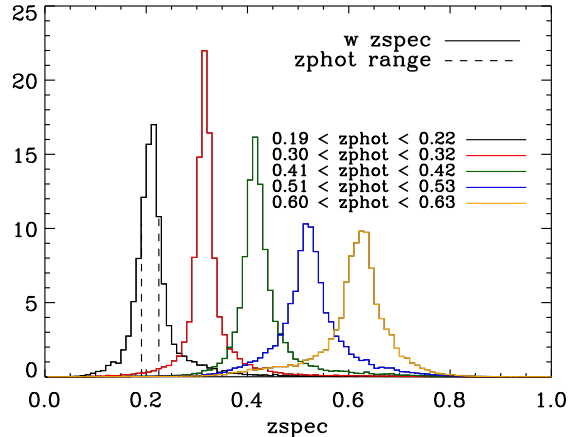
FIG. 3.— Weighted distribution of spectroscopic redshifts in a few bins of photometric redshifts. We chose weights such that the weighted distributions of each of the five SDSS bandpasses match that of the photometric sample in the given bin. The error bars come from bootstrap re-sampling the spectroscopic validation set.
