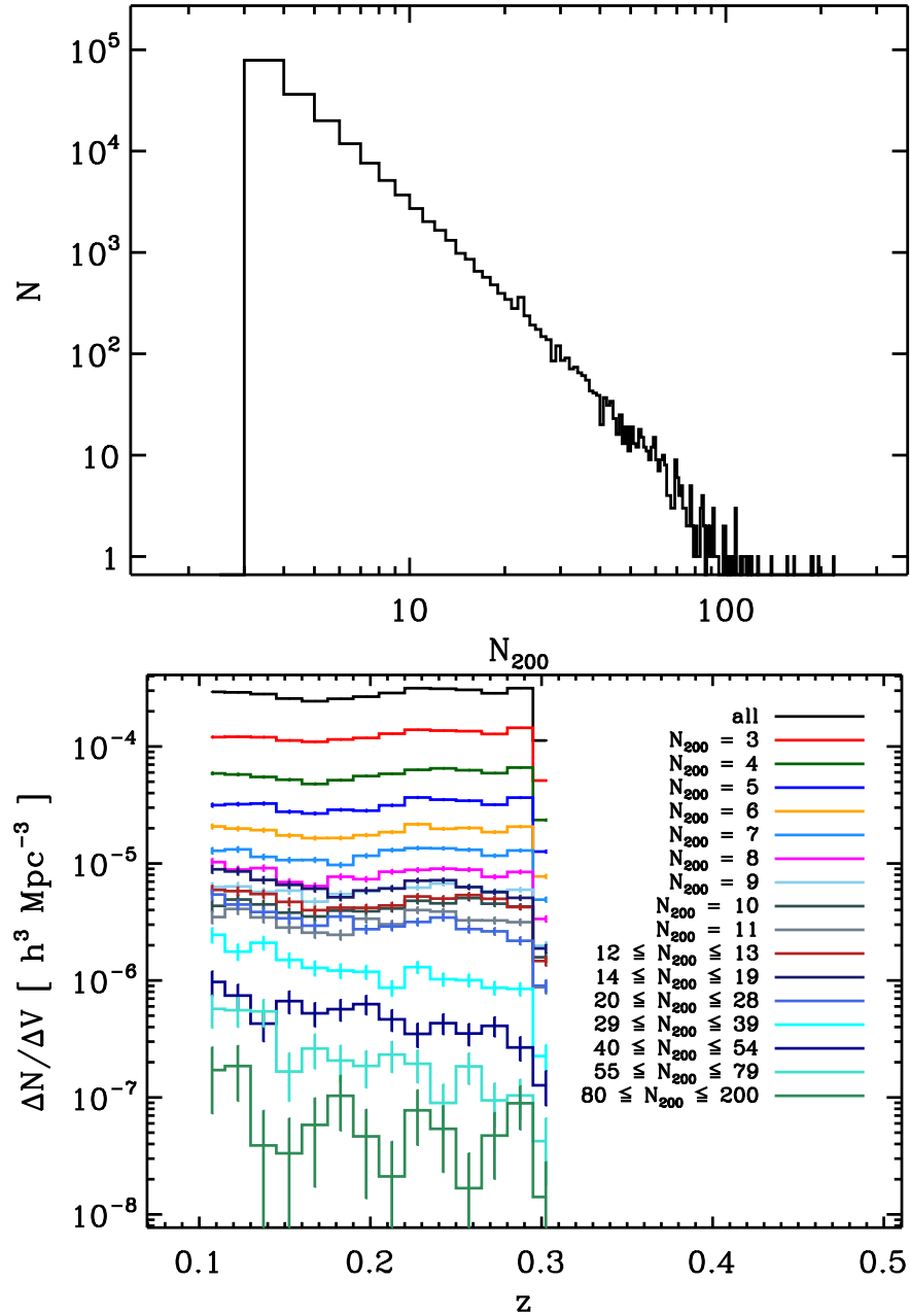
FIG. 4.— Top panel: Histogram of N_{200} , the number of red galaxies brighter than 0.4L_* within r_{200}^{gals} , for the cluster sample. Bottom panel: Number density as a function of redshift for differential bins of N_{200} .
