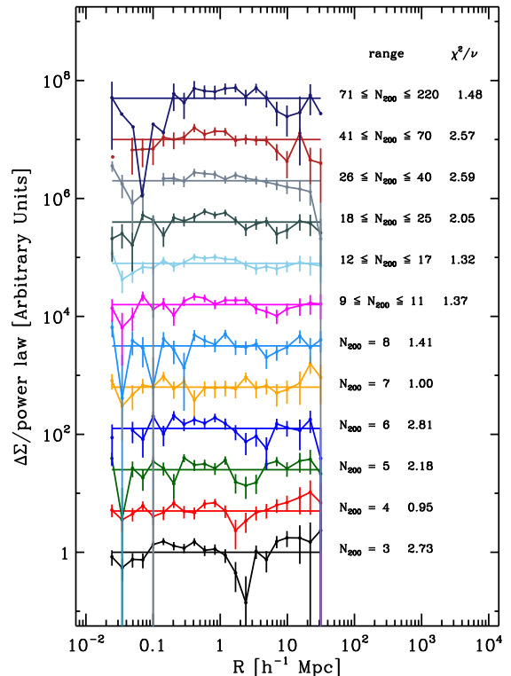
FIG. 8.— Power law fits in each N_{200} bin. For each bin, the best fitting power law (see Table 1) has been divided out and the signal scaled arbitrarily to separate the profiles visually. For clarity, the error bars for points with S/N < 1 have been suppressed for the top two bins. Each curve is labeled by its richness range and reduced \chi^2 for the power law fit. The profiles are not generally good fits to a power law and demonstrate systematic deviations as a function of scale.
