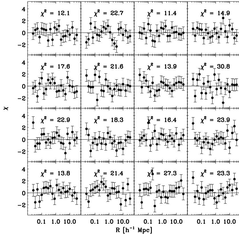
FIG. 11.— Bins of luminosity as in Figure 10 with each L_{200} bin split at the median redshift of 0.25. The data points are the difference between high redshift and low redshift splits divided by the error (added quadratically). The distribution of \chi^2 between the 16 bins is consistent with that expected from random scatter with 21 degrees of freedom.
