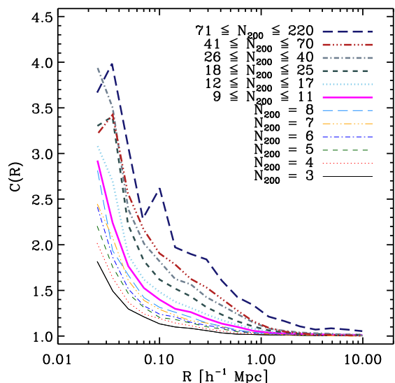
FIG. 6.— Correction factor for the clustering of source galaxies with the clusters in bins of N_{200} . The multiplicative factor C(R) is calculated and applied for all profiles shown herein.
