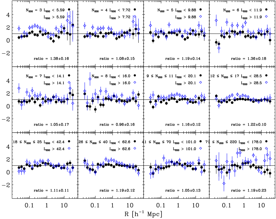
FIG. 9.— The same 12 N_{200} bins from figure 7 with each bin split into two by L_{200} . The L_{200} split is at the 2/3 quantile. The upper quantile is represented by the diamond symbols, the lower by the filled circles. The best fitting power-law for each N_{200} bin before splitting is divided out. The mean ratio of the splits is shown in the legend. There is a further correlation with luminosity within each N_{200} bin.
