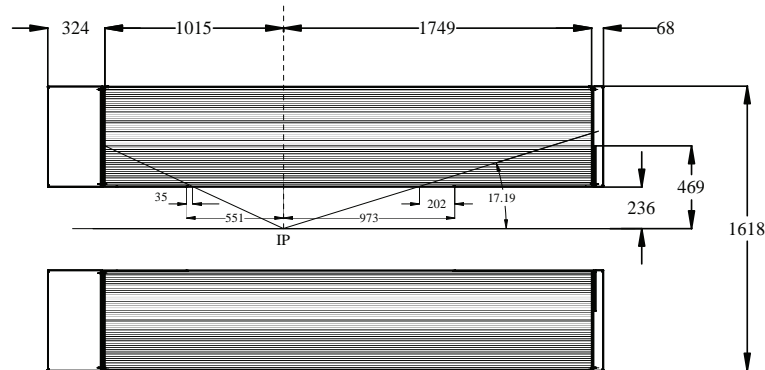
Figure 3.4: Side view of the BaBar drift chamber. The dimensions are in mm.
