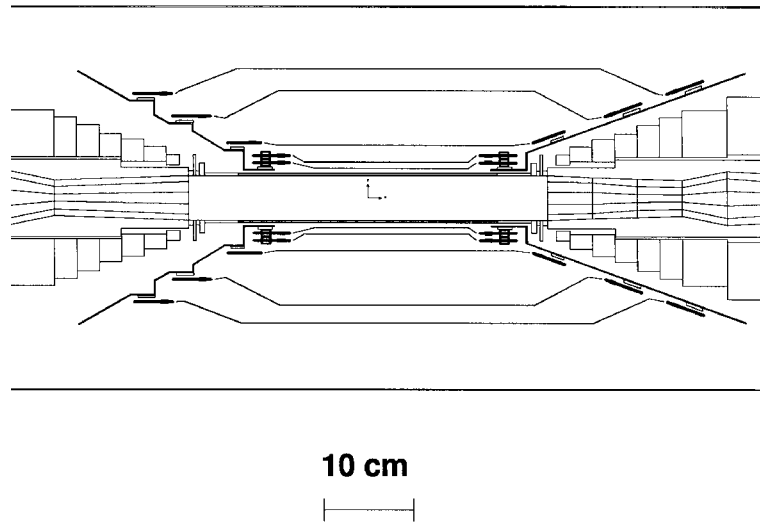
Figure 3.2: Detail of the inner part of the apparatus, showing the cross-sectional view of the silicon vertex tracker in a plane containing the beam axis.
