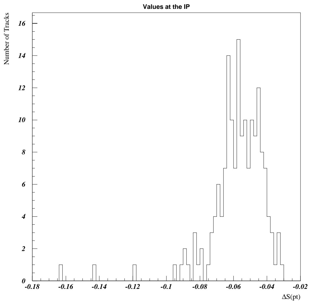
Figure 7.6: Muon \Delta S(p_t) distribution for 0.5 \leq p \leq 0.6 GeV/c
