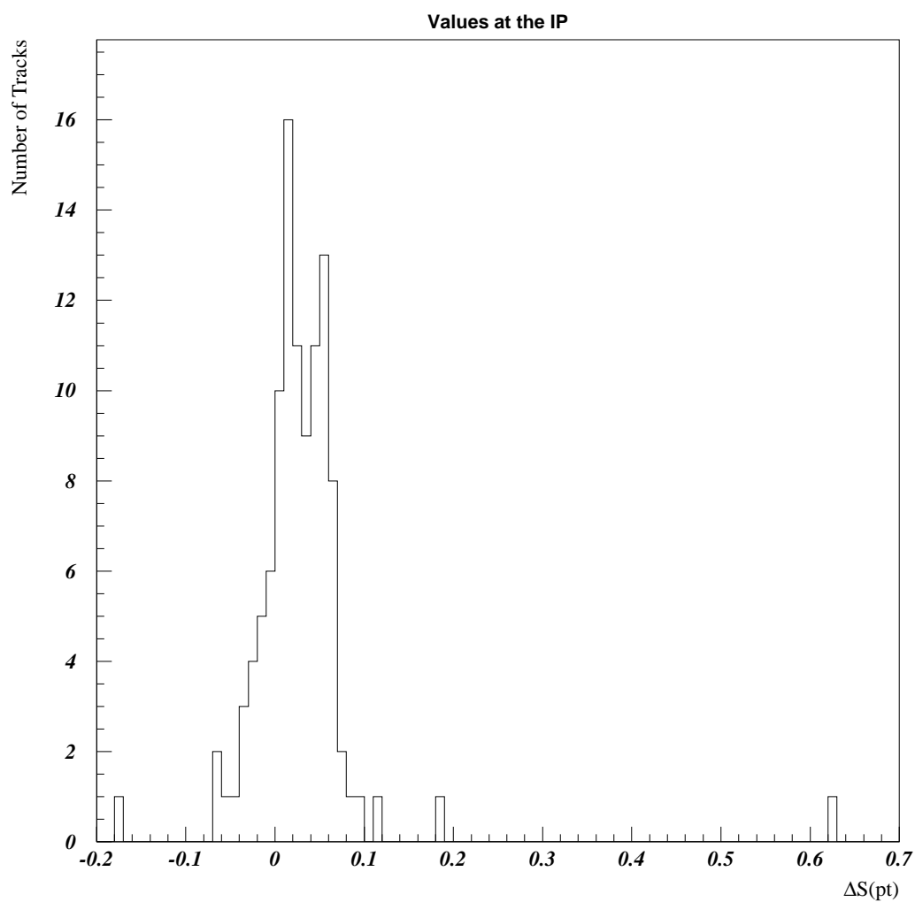
Figure 7.12: Proton \Delta S(p_t) distribution for 3.1 \leq p \leq 3.2 GeV/c
