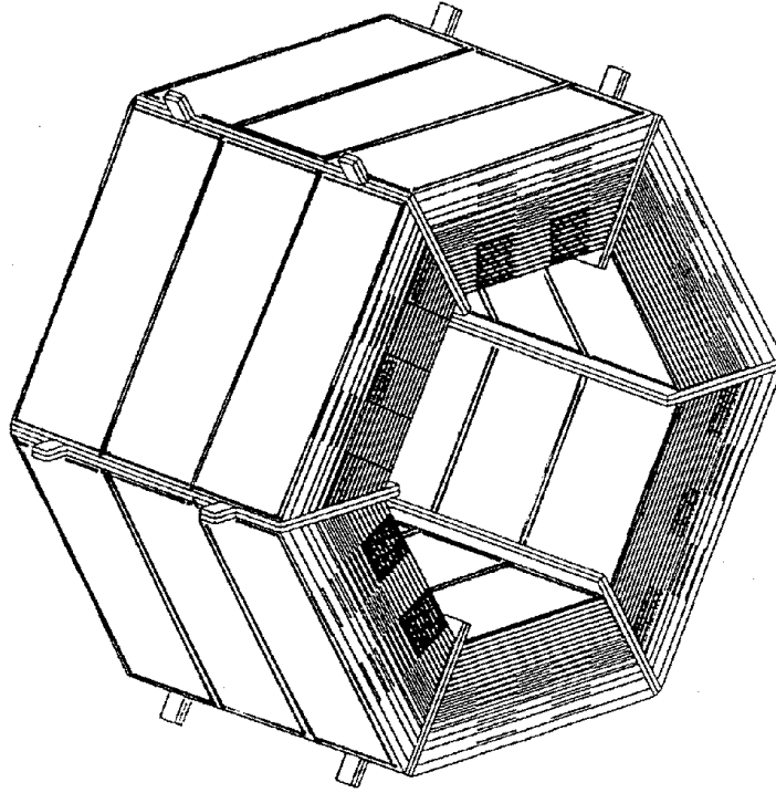
Figure 3.8: The IFR Barrel: layout of the RPC Modules.
