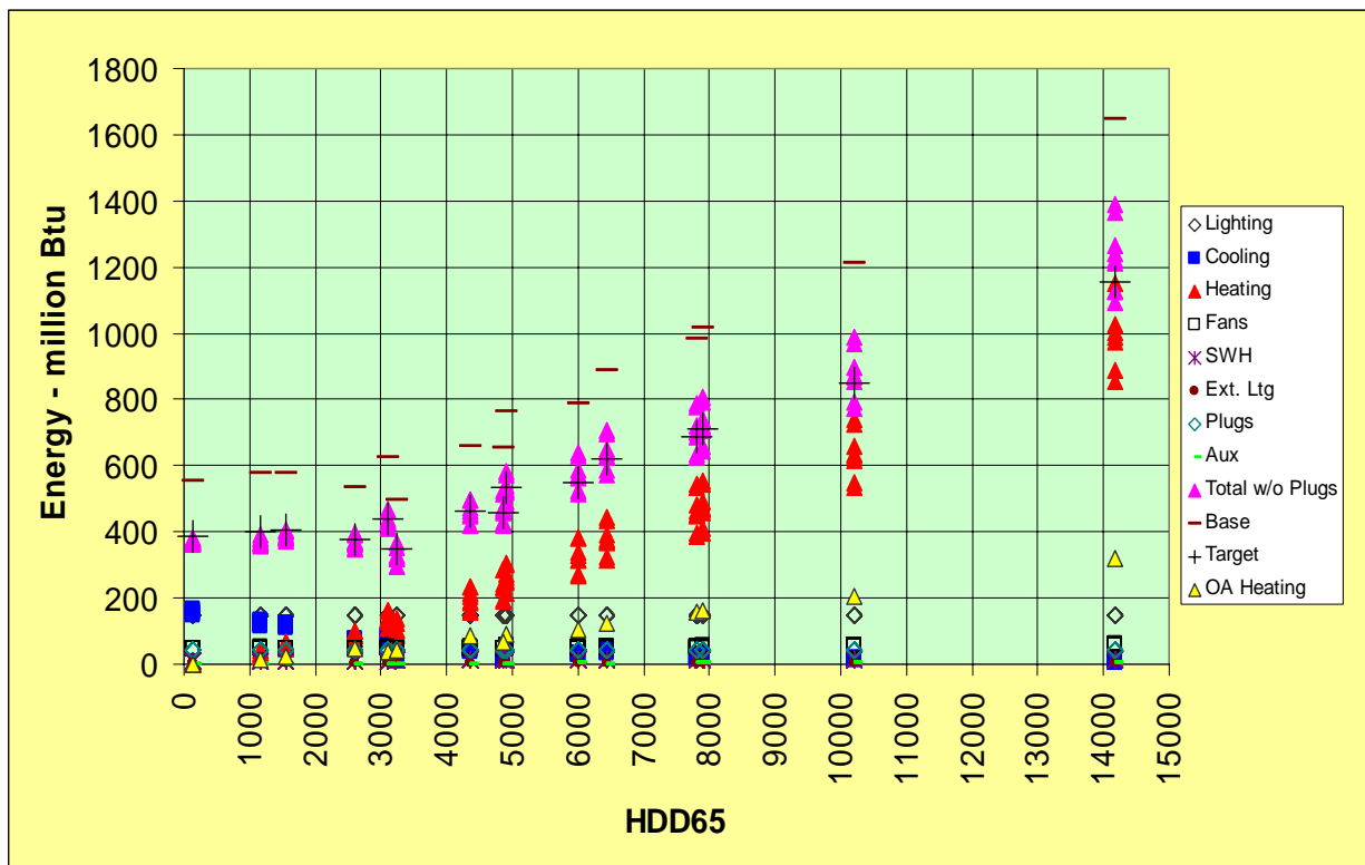
Figure 9-1 7,500-ft 2 Strip Mall Energy Use
