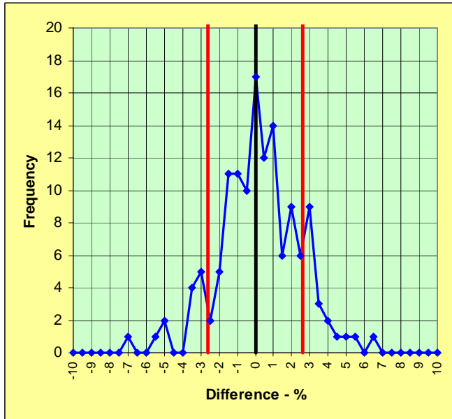
Figure 9-2 Distribution of Total Energy Difference, Regression – DOE-2 (%) Standard Deviation = 2.62
