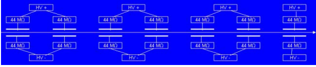
Figure 3: Electrostatic separator high voltage circuit.
