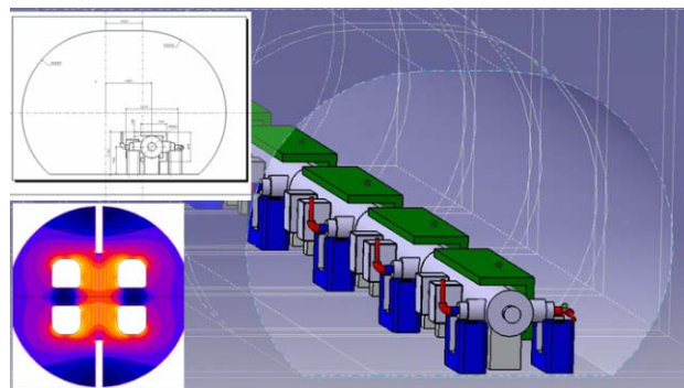
Figure 2: Layout of electrostatic separators with split electrodes in the enlarged tunnel. The compensating dipole envelopes the separator.
