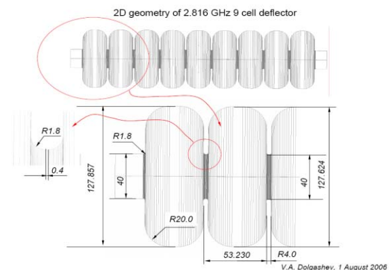
Figure 2: A 2.816-GHz 9-cell deflecting cavity.
