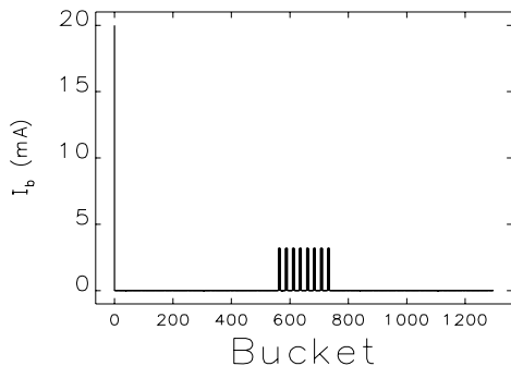
Figure 7: Hybrid-fill pattern 1+7*8 used in the APS storage ring.
