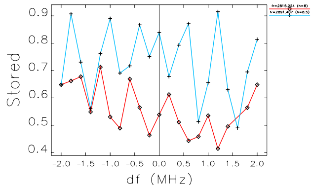
Figure 9: Fraction of current stored in the ring as a function of detuning of the deflecting cavity. The central frequency of the cavity considered is either h=8 (red curve) or h=8.5 (blue curve).
