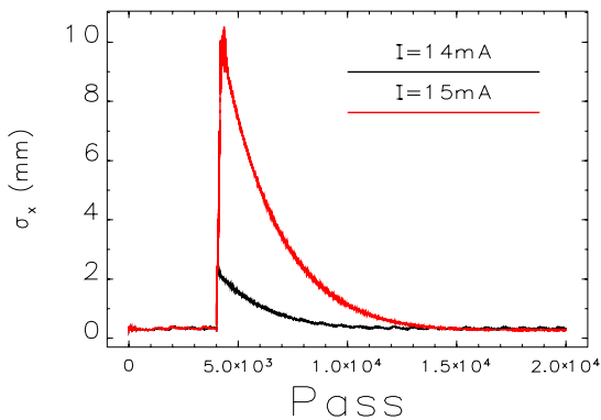
Figure 4: The evolution horizontal beam size after a 3-mm horizontal kick at pass 4000 shows the beam size blows up when the current is above 14 mA.
