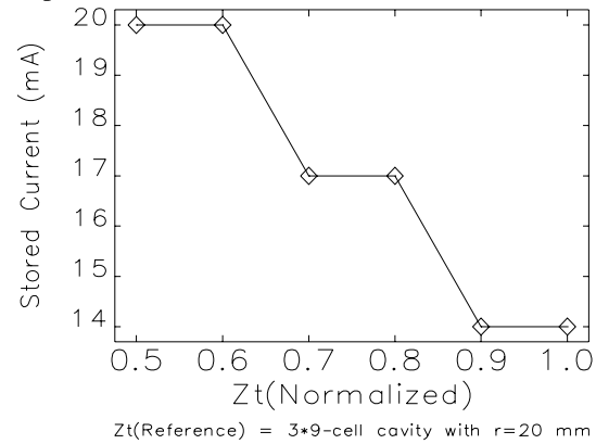
Figure 5: Single-bunch current in the storage ring as a function of deflecting cavity impedance
