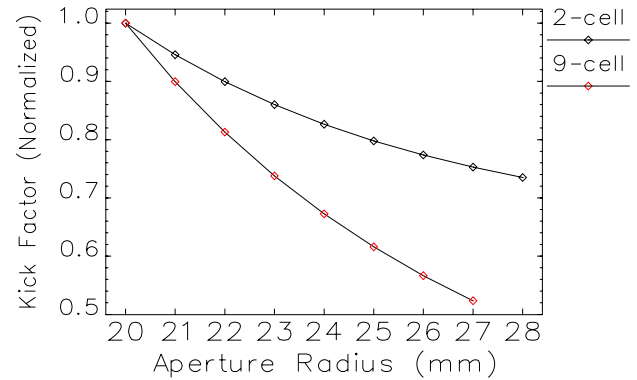
Figure 6: Transverse kick factor variation as function of aperture radius.
