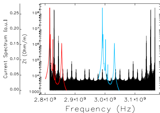
Figure 8: Beam spectrum and HOM impedance at h=8 and h=8.5 .
