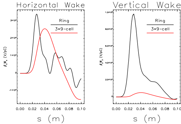
Figure 3: Comparison of a total wake potential of the ring and three 9-cell cavities: horizontal wake \beta_x W_x (left) and \beta_y W_y (right).
