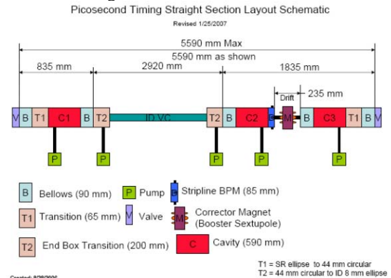
Figure 1: Short x-ray pulse straight section.
