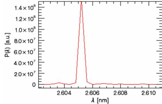
Figure 7: Radiation Spectrum of the fifth harmonic for a possible seeded scheme at 2.3 GeV.
