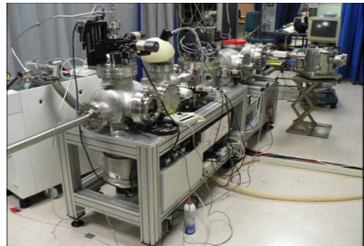
Figure 4: Harmonic Gas generation chamber
