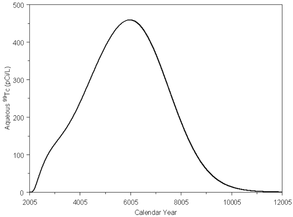
Figure 5.36. Calculated Distributions for 99 Tc at a Hypothetical Receptor well Under a Recharge Rate of 0.5 mm/yr Based on STOMP Simulations
