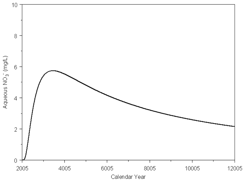
Figure 5.41. Calculated Distributions for NO 3 - at a Hypothetical Receptor well Under a Recharge Rate of 0.0 mm/yr Based on STOMP Simulations
