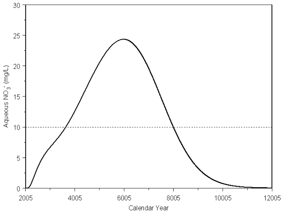
Figure 5.37. Calculated Distributions for NO 3 - at a Hypothetical Receptor well Under a Recharge Rate of 0.5 mm/yr Based on STOMP Simulations. The dotted line is the MCL of 10 mg/L.
