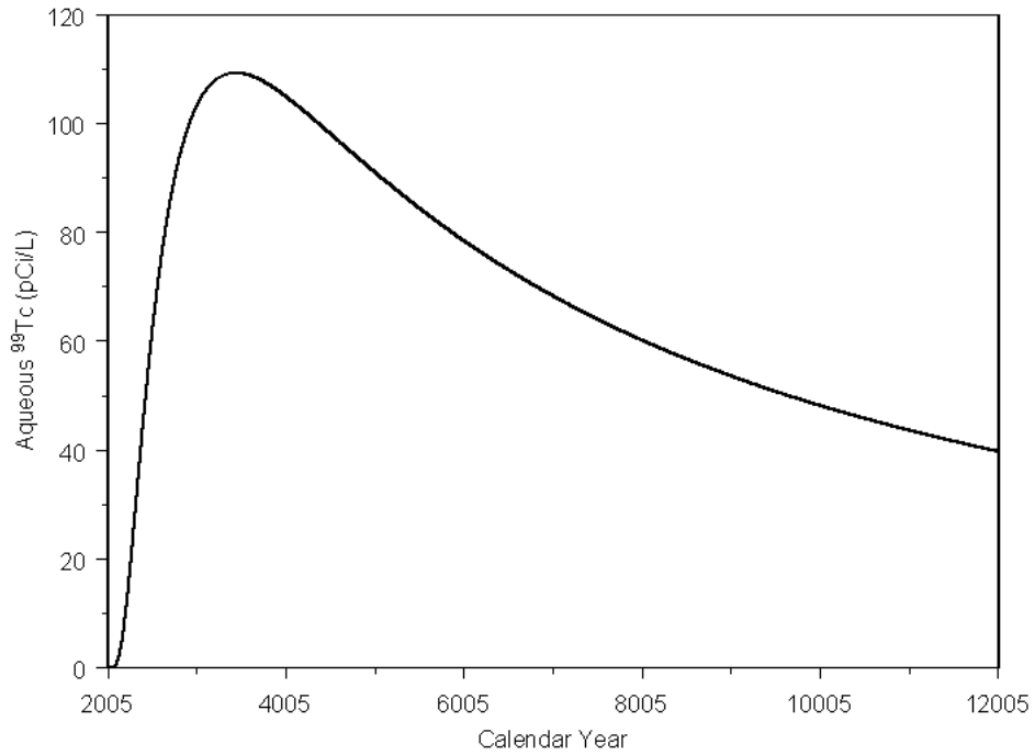
Figure 5.40. Calculated Distributions for 99 Tc at a Hypothetical Receptor well Under a Recharge Rate of 0.0 mm/yr Based on STOMP Simulations
