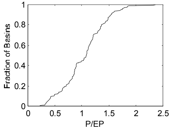
Figure 5 – Distribution of the Ratio of Mean Annual Precipitation to Mean Annual Potential Evaporation in the Arkansas-Red River Basin
