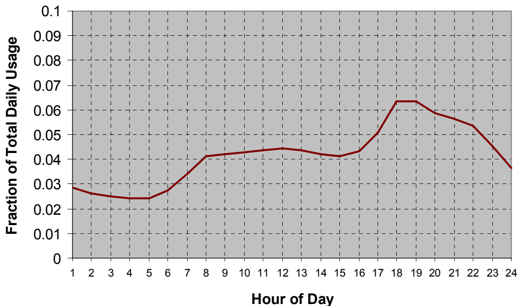
Figure 16. Total combined residential equipment profile (Pratt et al 1989)
