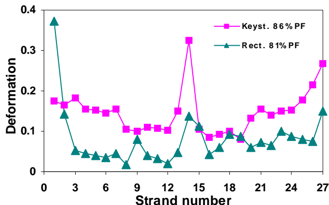
Fig. 5. Strand deformation as a function of position in 27-strand cables.
