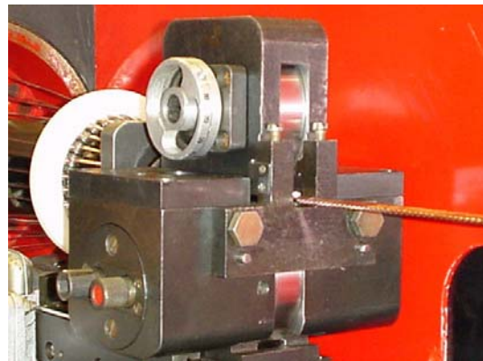
Fig. 3. Rectangular cable forming fixture.
