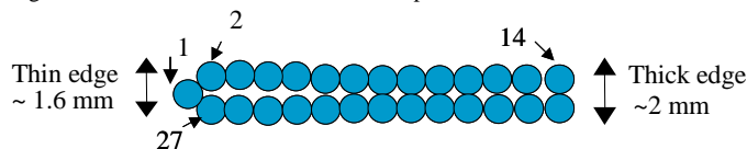
Fig. 6. Scheme of the strand numbering used in a cable.
