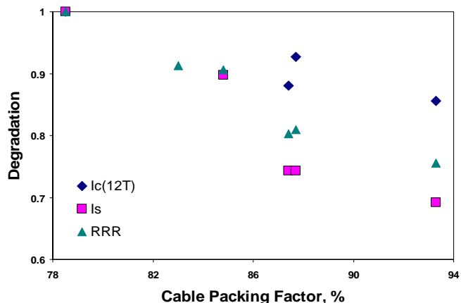
Fig. 9. Cabling degradation at 4.2 K for nominal TQ cable at 12 T and 4.2 K.
