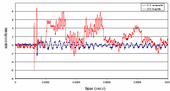
Figure 5: Response to intense beam comparison between graphite and carbon-composite targets
