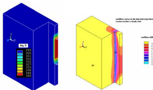
Figure 7: Estimated temperatures and critical stresses in the SNS primary collimator during a full beam intercept
