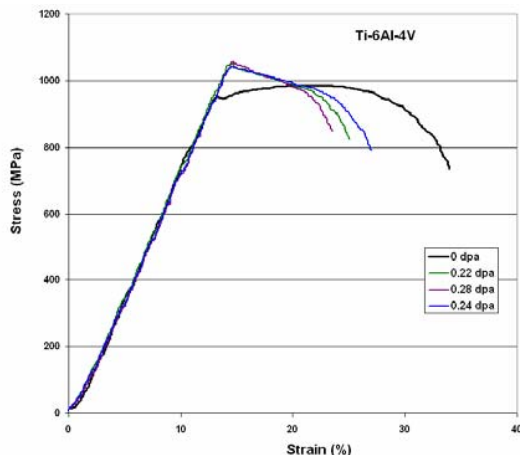
Figure 21: Irradiation effects on stress-strain relation of Ti-6Al-4V
