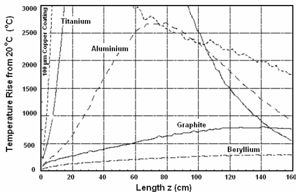
Figure 3: Estimates of temperature in the LHC collimators based on different material choices [Ref. 5]
