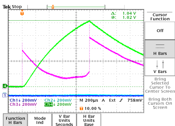
Figure 1: Operation of CCII at nominal 30 MV/m gradient. Green trace is Transmitted power, Magenta trace is Reflected power. Horizontal marker indicates 30 MV/m.
