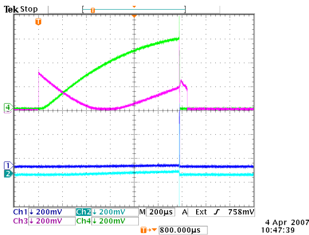
Figure 3: CCII Quench at low (16 MV/m) gradient. Green – transmitted power, Magenta – reflected power, Cyan – rectified Downstream HOM power, Blue – rectified Upstream HOM power
