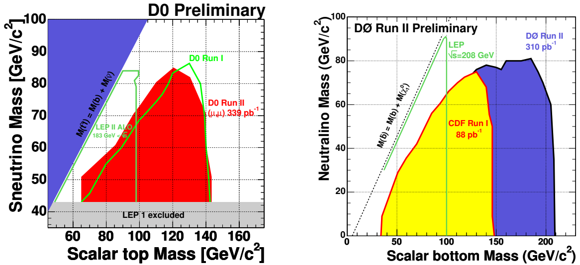
Figure 2: 95% C.L. exclusion regions for the \tilde{t}_1 \rightarrow b\tilde{\nu} (left) and \tilde{b} \rightarrow b\tilde{\chi}_1^0 search (right).
