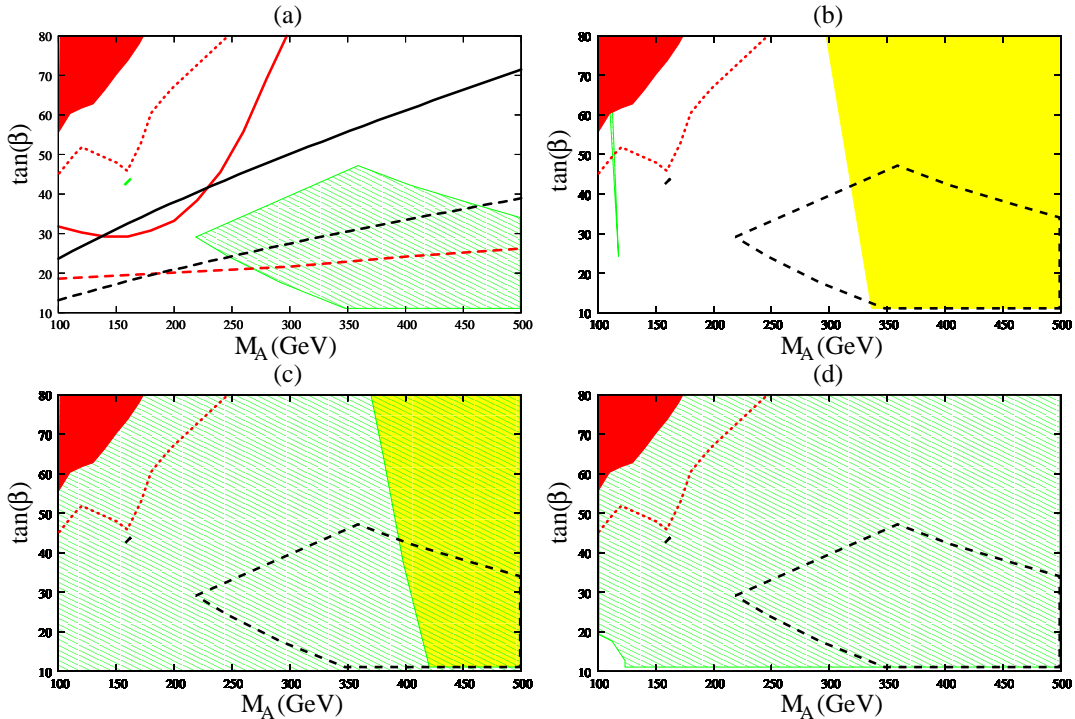
Figure 3: (a)–(d) The lines and the colors correspond to the same quantities as in Fig. (2), where the SUSY parameters are the same except for X_t = 1 TeV.
