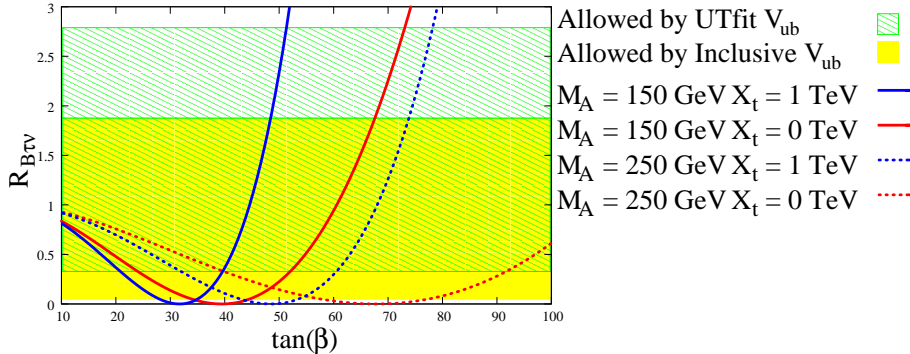
Figure 1: The green(grey) hatched area is the 2\sigma allowed region of the ratio R_{B\tau\nu} if the fitted value of |V_{ub}| is used to calculate the standard model prediction of the B_u \rightarrow \tau\nu decay rate. The yellow(light grey) is corresponding region if the inclusive determination of |V_{ub}| is used instead of the fitted value. The solid (dashed) lines show the variation of R_{B\tau\nu} with respect to \tan\beta for M_A = 150\text{GeV}(250\text{GeV}) , while the red (grey) color and blue (dark grey) color correspond to X_t = 0 and X_t = 1 TeV respectively.
