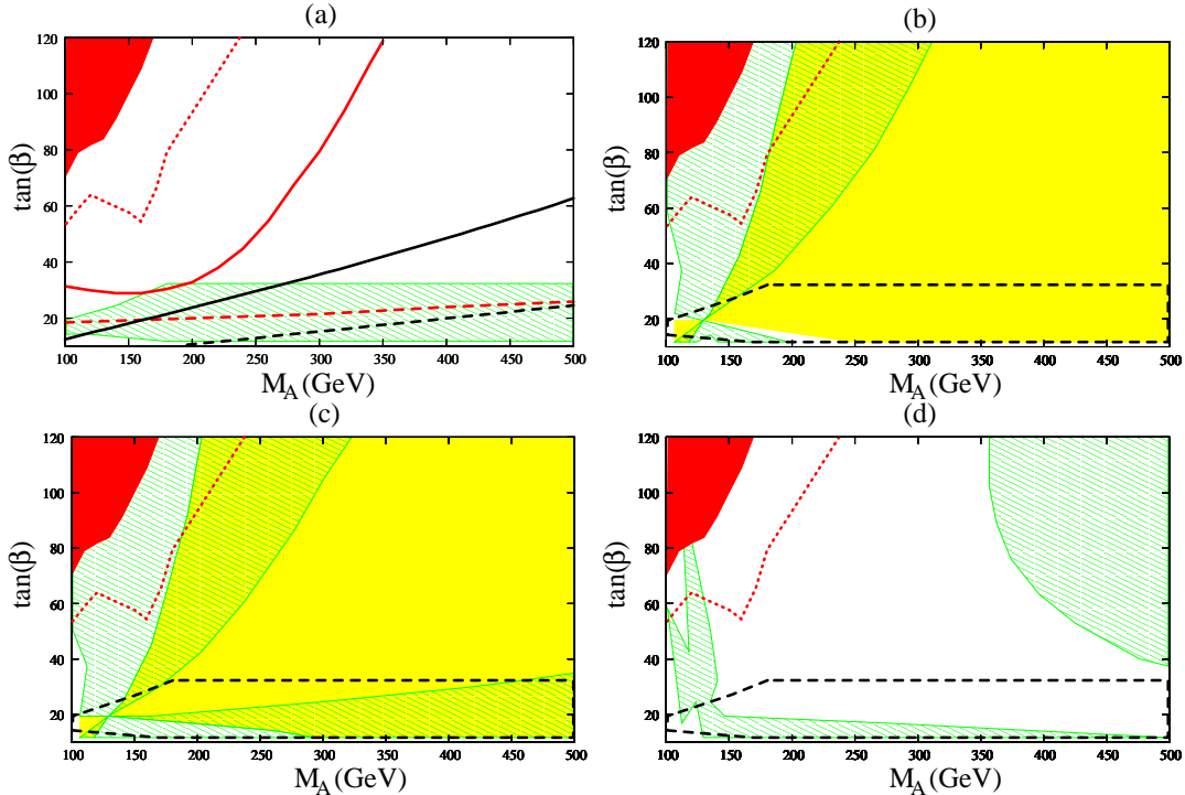
Figure 5: (a)–(d) The lines and the colors correspond to the same quantities as in Fig. (2), where the SUSY parameters are the same except for M_3 = 500 GeV, M_{SUSY} = 800 GeV, X_t = -1.2 TeV and \mu = 2.5 TeV.
