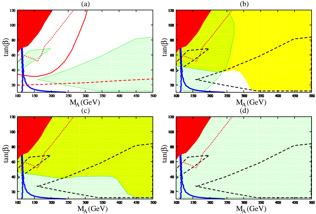
Figure 4: (a)–(d) The lines and the colors correspond to the same quantities as in Fig. (2), where the SUSY parameters are the same except for X_t = 0 GeV, \mu = 1.5 M_{SUSY} and M_{SUSY} = 2 TeV. The region below the blue (black) solid line corresponds to the area excluded by the LEP bound on the SM-like Higgs boson for m_t = 170.9 GeV.
