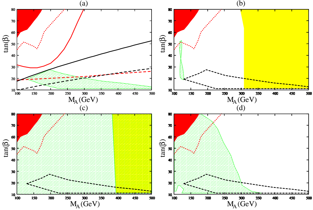
Figure 2: The red (grey) region, in all four figures, is excluded by the CDF experiment's search for non-standard Higgs bosons in the inclusive A \rightarrow \tau^+\tau^- channel at 1 \text{ fb}^{-1} luminosity. The dotted line shows the corresponding D0 excluded region at 1 \text{ fb}^{-1} . (a) The solid and dashed lines represent the future reach for the Tevatron (at 4 \text{ fb}^{-1} ) and LHC (at 10 \text{ fb}^{-1} for B_s \rightarrow \mu^+\mu^- and at 30 \text{ fb}^{-1} for A \rightarrow \tau^+\tau^- ) respectively, where the red (dark gray) lines correspond to the non-standard Higgs search reaches in the H \rightarrow \tau\tau channel while the black lines are the projected \mathcal{BR}(B_s \rightarrow \mu^+\mu^-) bounds for \mu = -100 \text{ GeV} , X_t = 2.4 \text{ TeV} , M_{SUSY} = 1 \text{ TeV} and M_3 = 0.8 \text{ TeV} . The green (gray) hatched regions are those allowed by the present B-physics constraints on the B_u \rightarrow \tau\nu b \rightarrow s\gamma and B_s \rightarrow \mu^+\mu^- branching ratios. (b) and (c) For the same SUSY mass parameters the yellow (light gray) area is the 5\sigma discovery region in the h \rightarrow \gamma\gamma channel, while the green (gray) hatched area is the same for the h \rightarrow \tau\tau channel for the CMS and ATLAS experiments respectively at 30 \text{ fb}^{-1} . (d) Green (gray) hatched region is the 3\sigma evidence region for the SM-like Higgs searches (at 4 \text{ fb}^{-1} ) at the Tevatron. (b)–(d) The areas surrounded by the dashed black curves correspond to the regions allowed by present B-physics constraints.
