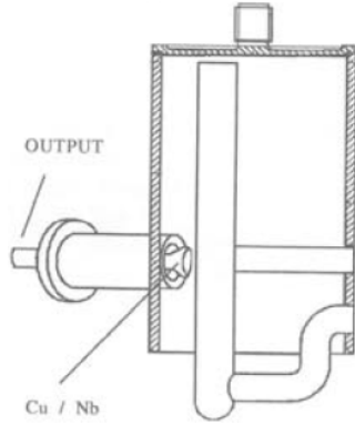
Figure 3: HOM coupler schematic
