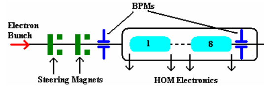
Figure 9. Steering Setup for HOM dipole experiment
