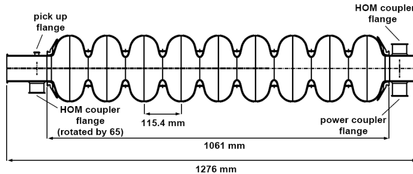
Figure 2: Schematic of a TESLA cavity.
