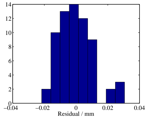
Figure 15: Residual of the x offset prediction using the HOM analysis for cavity #5 in module #5.
