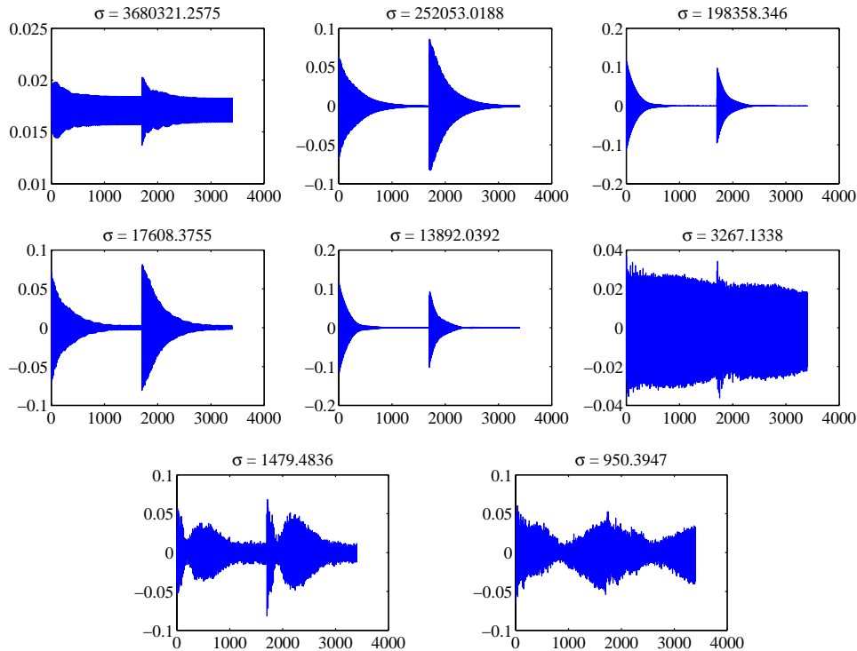
Figure 12: Top eight SVD modes for an example dataset, including their singular values.
