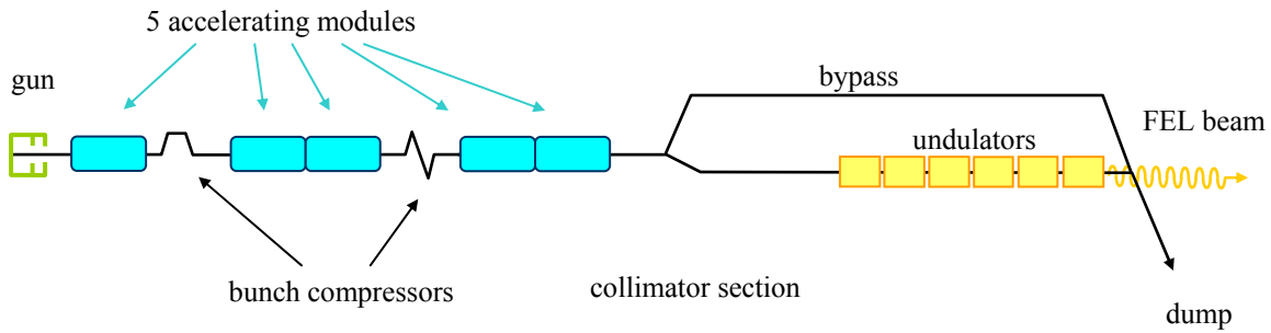
Figure 1: Schematic of the FLASH facility
