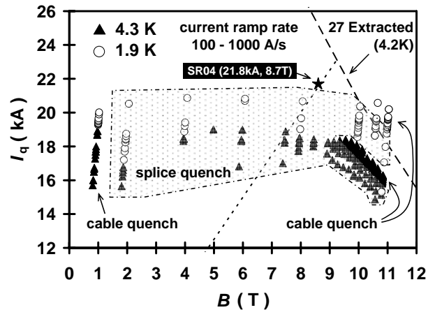
Fig. 9. Quench current values of the cable test at CERN at 1.9 K are shown together with values at 4.3K. Also in this figure, the load line for SR04 magnet and its highest quench value at 3.95 K are shown for comparison.
