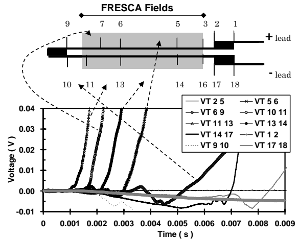
Fig. 7. Quench behaviors and quench velocity determination at 10.8 T at 4.3 K. Ramp rate at 1000 A/s. I q = 15.81 kA. V q = 109 m/s for >1.2 ms.
