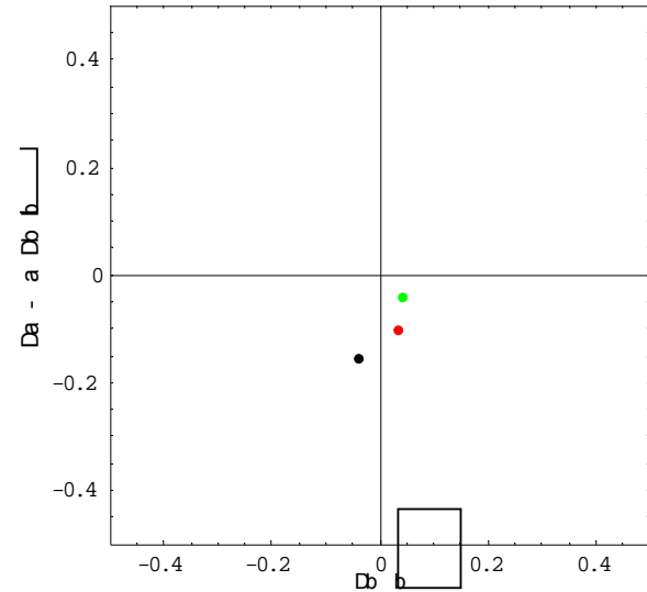
Figure 4. Vertical mismatch for different settings of the Q711 quadrupole. Black is nominal current, red is +10A, green is +20A.
