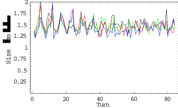
Figure 2. Vertical beam size for the first 85 turns following injection for proton bunches #5 (black), #11 (red), #15 (green) and #19 (blue), taken during the same collider shot. There is clear and consistent evidence of mismatch.
