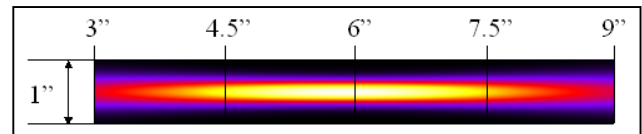
Figure 3: Intensity distribution (arb. units) along planar cut transverse to the axis from the 90-degree deflection point of the mirror for \lambda = 1 mm, E.F.L. = 152.4mm, O.D. = 50.8mm with a Gaussian laser source, RMS radius = 6.35mm reflected into focus.
