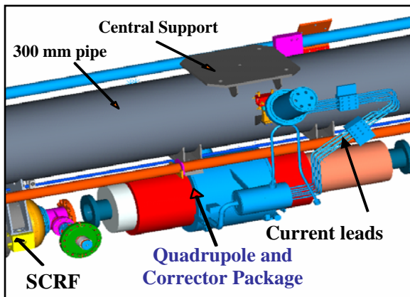
Figure 2: Conceptual layout of a quadrupole-corrector – BPM assembly mounted at the center of a cryomodule.
