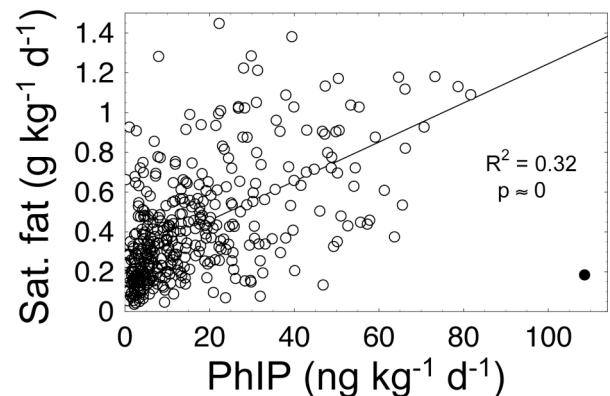
Figure 2. Saturated fat (g/kg-d) intake estimated by FFQ vs. PhIP intake estimated by the LLNL Meat questionnaire for 392 Oakland, CA-area African-American men (open points). Linear regression shown (solid line) indicates a significantly positive association. A single point (closed circle) determined to be an outlier (p < 10 -5 by F test) was excluded from the regression
