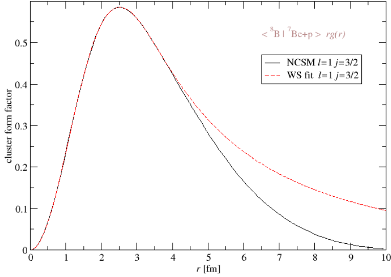
Fig. 4. Computed radial-cluster form factor, rg(r) , for the ground state of {}^7\text{Be} plus proton with the ground state of {}^8\text{B} . The black line represents the NCSM result, while the red line represents a renormalized overlap obtained from a Woods-Saxon potential whose parameters were fit to the compute overlap up to 3.5 fm and constraining the energy to reproduce the experimental separation energy.
