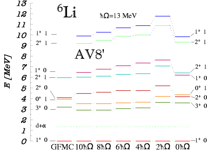
Fig. 1. Comparison of the NCSM and GFMC spectra obtained for the Argonne AV8' potential. The NCSM spectra are shown as a function of the model size denoted by N_{\max}\hbar\Omega .
