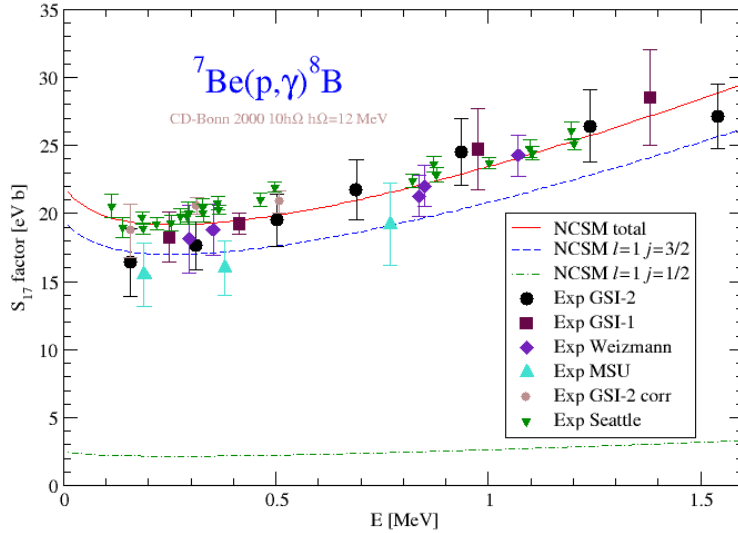
Fig. 5. Preliminary calculation of the {}^7\text{Be}(p,\gamma){}^8\text{B} S-factor using renormalized cluster form factors as shown in Fig. 5. The blue and green dashed lines show the contribution due to the l = 1, j = 3/2 and j = 1/2 states, respectively.
