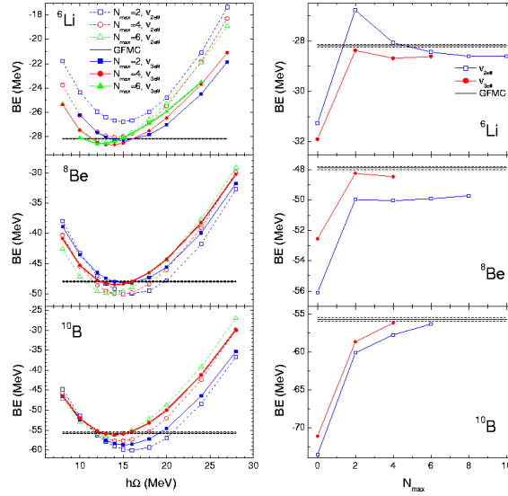
Fig. 2. Calculated ground-state energy of {}^6\text{Li} (upper panel), {}^8\text{Be} (middle panel) and {}^{10}\text{B} (lower panel) using the AV8' NN potential with Coulomb. Results using the two-body effective interaction and the three-body effective interaction in basis spaces up to 6\hbar\Omega in the range of HO frequencies of \hbar\Omega = 8 - 28 MeV are shown and compared to the GFMC results from Ref. [6]. On the rhs, the energies at the HO frequency minima as a function of N_{max} are plotted.
