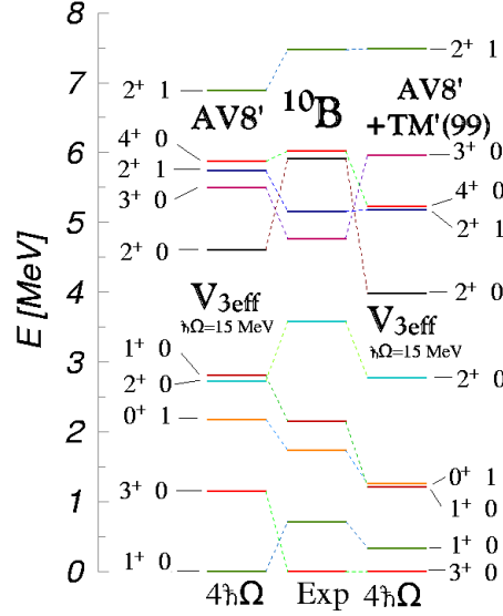
Fig. 3. Comparison of low-lying spectrum of ^{10}\text{B} obtained with the AV8' two-nucleon interaction alone (left side) and with the Tucson-Melbourne three-nucleon force (right side) with experiment.
