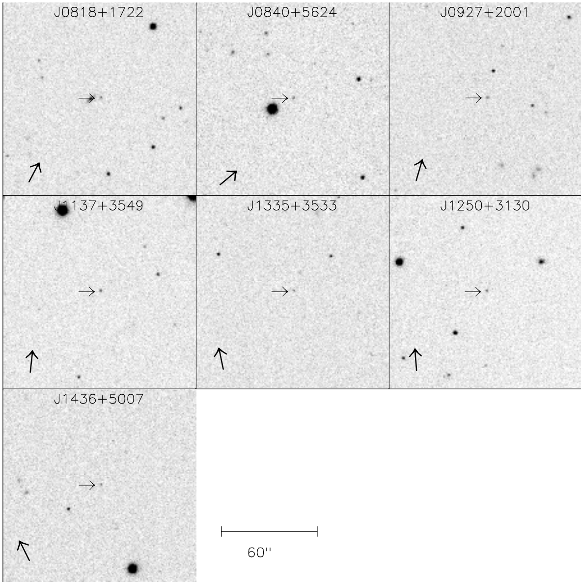
Fig. 1.— SDSS z -band images of the seven new z > 5.7 quasars. Each side of the finding chart is 120'' . The arrow at the lower left indicates the direction of North on the finding chart; East is 90^\circ counterclockwise from North.
