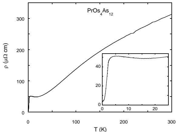
FIG. 5: Electrical resistivity \rho vs T from 2 K to 300 K. The inset shows \rho(T) from 0.06 K to 25 K.
