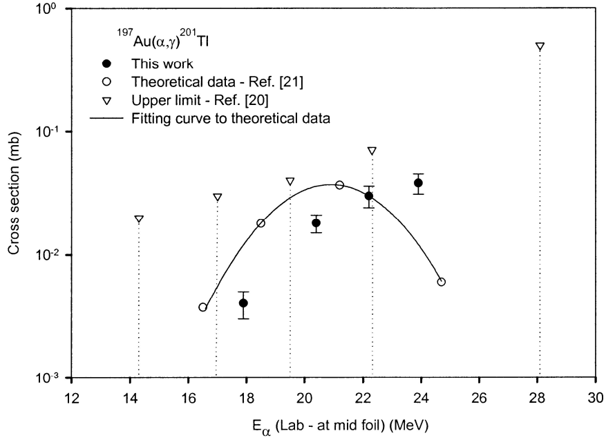
FIG. 2. Cross sections for the ^{197}\text{Au}(\alpha, \gamma)^{201}\text{Tl} reaction.
