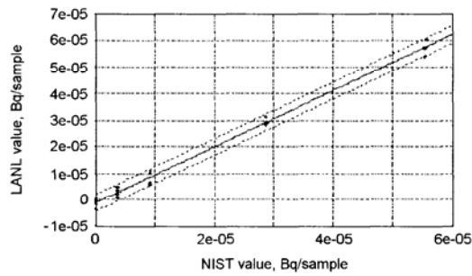
Fig. 2. LANL TIMS 239 Pu results compared to NIST values. Regression analysis: y = a + bx ; a = -9.92e-07 ; b = 1.06 ; 90% prediction interval
