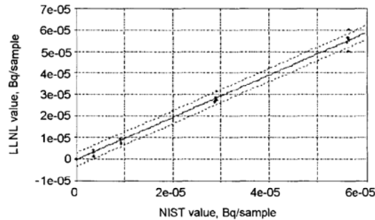
Fig. 3. LLNL AMS 239 Pu results compared to NIST values. Regression analysis: y = a + bx ; a = -2.43e-07 ; b = 0.989 ; 90% prediction interval
