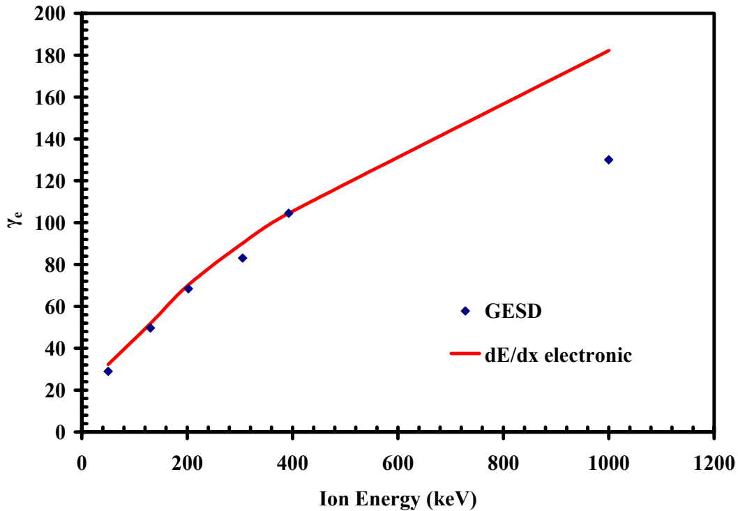
FIG. 5. Electron yield obtained with Gas-Electron Source Diagnostic at 88 degrees compared with the electronic stopping power normalized to the experimental electron yield at 393 keV.
