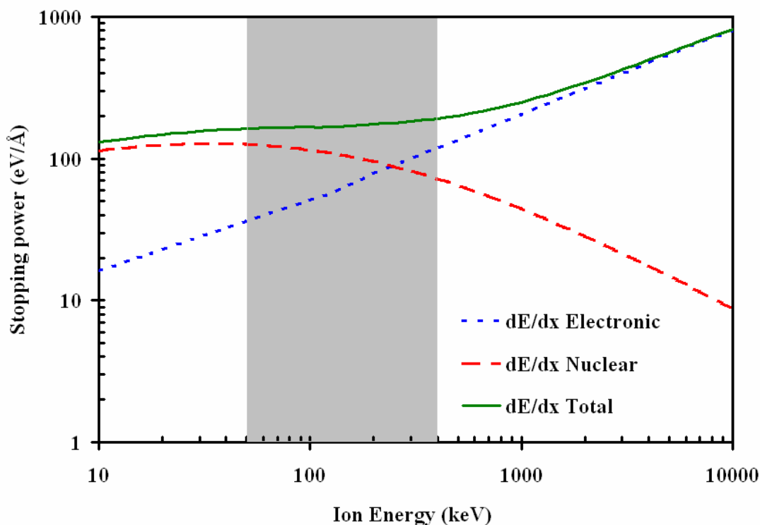
FIG. 1. (Color) Stopping power for K^+ ions hitting stainless steel target, from TRIM 2003 calculations.
