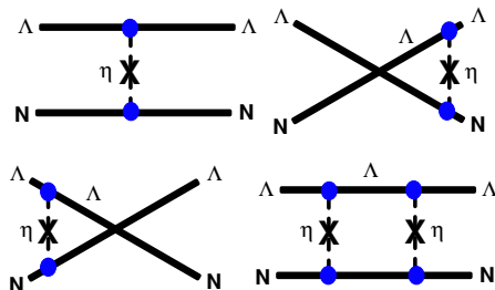
FIG. 2: The LO and NLO contributions to \Lambda N scattering from hairpin-exchange in PQ \chi PT. The shaded blobs are vertices from eq. (12).
