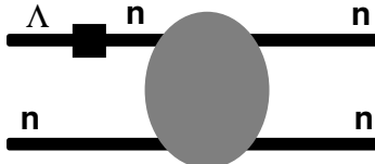
FIG. 6: An example of a contribution to \Lambda n \rightarrow nn .
