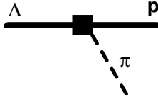
FIG. 3: Tree-level diagram that gives the leading-order contribution to the S -wave amplitudes for the nonleptonic decay \Lambda \rightarrow p\pi^- . The solid square denotes an insertion of the leading-order weak interaction from eq. (19).
