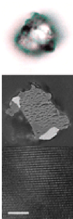
Fig. 4. Three images of the 8- \mu\text{m} terminal particle at end of the >2-mm-long track 27 (Sitara), also shown in Fig. 1 . The top is an optical image showing parent central grain (that is also birefringent) with two attached opaque phases. Other focus depths show additional opaques inside the grain. The middle image is an SEM backscattered electron (BSE) image of the flat surface ("potted butt") of the particle mounted in acrylic after several dozen 70-nm slices had been removed with a diamond microtome. The image brightness is proportional to mean atomic weight and this, along with x-ray spectral measurements, shows that the particle is a solid rock composed of at least four phases. The two bright regions are sulfides; one is pyrrhotite \text{Fe}_{1-x}\text{S} , and the other is pentlandite, a Ni-rich sulfide. The central gray region marked by aligned "chatter pits" from the diamond knife is enstatite. The smooth gray regions are an undetermined crystalline Mg silicate that contains Na, Al, and Ca at abundances of several percent. The bottom image shows the enstatite grain observed in a microtome section at near atomic-scale resolution at near atomic-scale resolution. Scale bar, 5 nm). [View Larger Version of this Image (63K GIF file)]
