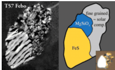
Fig. 2. The 8- \mu\text{m} terminal particle of T57 (Febo), a bifurcated track >1.4 mm long. The left image is a high-angle annular darkfield (HAADF) image of a 70-nm-thick microtome section of the particle. The images combined with x-ray spectral analysis show that the particle has three major components. The sulfide pyrrhotite on the left, a 3- \mu\text{m} enstatite grain in the upper middle, and fine-grained porous aggregate material with approximately chondritic elemental composition (Mg, Al, Si, S, Ca, Cr, Mn, Fe, Ni \sim solar ratios) dominates the right half of the image. The particle's smooth exterior contour is probably due to abrasion during passage through aerogel, although the particle contains only trace amounts, at most, of adhering aerogel. The survival of fine-grained chondritic composition material as a major part of a terminal particle is unusual, and its survival may have been aided by shielding; it may have been in the lee of the large sulfide. The small inset image shows a reflected-light view of the "potted butt," the sample that remains after removing microtome sections.
