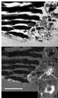
Fig. 5. Energy-filtered TEM images of the lower region of the T57 (Febo) slice shown in Fig. 2 (scale bar, 1 \mu\text{m} ). The top image is a zero-loss image made with electrons that did not lose energy during passage through the sample, and the lower image displays the carbon distribution. The carbon image was made with the standard three-window method that combines images taken in energy passbands above and below the 285-eV carbon edge. The sulfide on the left is carbon free, but regions of carbon are seen both as submicron components in the fine-grained chondritic component on the right and as partial rims on the sulfide grain. Isotopic measurements made at Johnson Space Center have shown considerable ^{15}\text{N} enrichment in the carbon-rich region shown in the expanded window.
