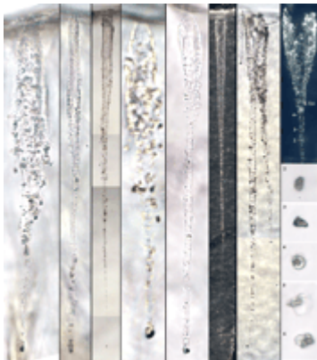
Fig. 1. Optical images of deceleration tracks of eight comet particles in aerogel that entered at the top and terminated at the base. Left to right, the track names and their lengths are T59 (0.35 mm), T58 Noni (0.29 mm), T61 (1.6 mm), T72 Gea (0.12 mm), T71 Surya (0.22 mm), T38 Tara (3.2 mm), T27 Sitara ( >2 mm), and T25 Inti (2 mm). The thinner tracks suffered very little fragmentation that leads to substantial production of side tracks. The break in the T38 track is due to sample preparation, and the upper bulb of T25 widened a bit when it was intentionally flattened. All of the other tracks have their original shapes. The squares below T25 (Inti) are magnified images of five of the major 5- to 12- \mu m particles. The tip of the track containing the 20- \mu m terminal particle was removed before the track image was taken. The terminal particle as well as many of the other fragments are isotopically and mineralogically linked CAIs, exotic refractory components in primitive meteorites that may have formed very close
