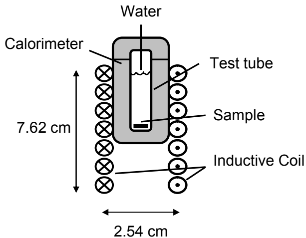
Fig 4. Calorimeter test setup with inductive coil specifications.
