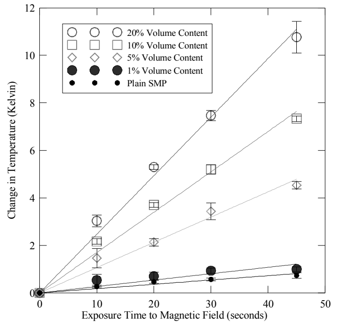
Fig 5. Heating curves of SMP loaded with 43.6 \mu\text{m} C2050 particles at varying volume contents with error bars at \pm one standard deviation. The slope of each curve was used to calculate the power dissipation.
