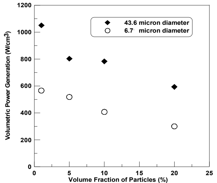
Fig 8. Volumetric Power Dissipation of magnetic particles vs. Volume Fraction of Particles, 12.2 MHz and 545 A/m.
