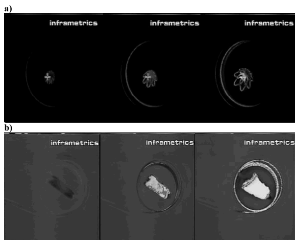
Fig 6. a) Actuation of SMP flower shaped device with 10% volume fraction of 43.6 \mu\text{m} particle diameter C2050 magnetic material (12.2 MHz at 400 A/m applied magnetic field). b) Actuation of SMP foam with 10% volume fraction of 43.6 \mu\text{m} particle diameter C2050 magnetic material (12.2 MHz at 400 A/m applied magnetic field).
