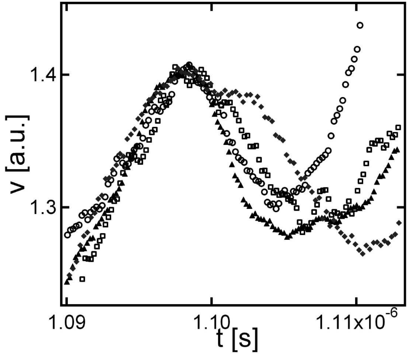
FIG. 3: Velocity relaxation regimes for all experiments, shifted and scaled to a common maximum.
