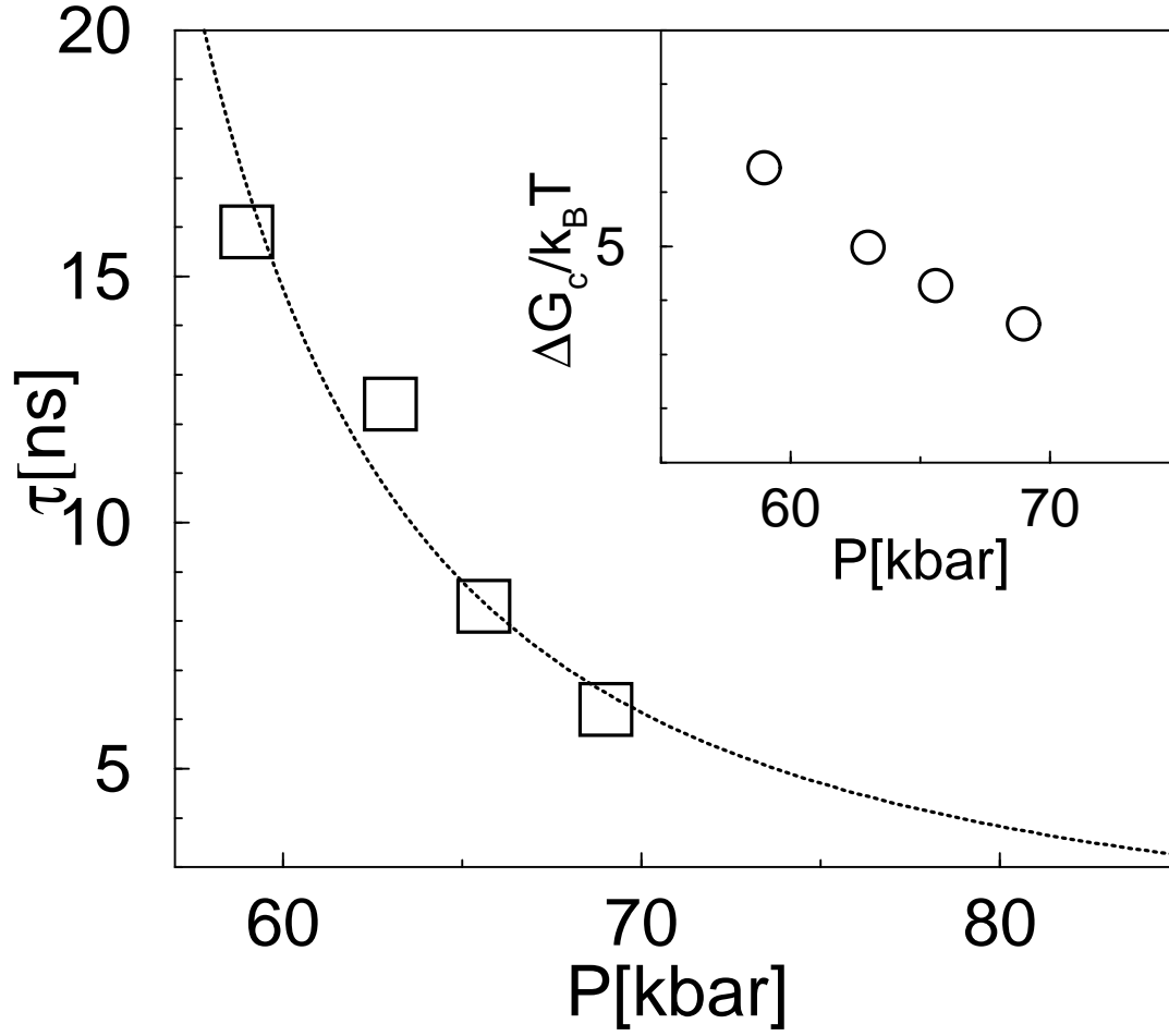
FIG. 4: Characteristic kinetic time scales as a function of pressure (see text). Inset - estimated nucleation barrier as a function of pressure.
