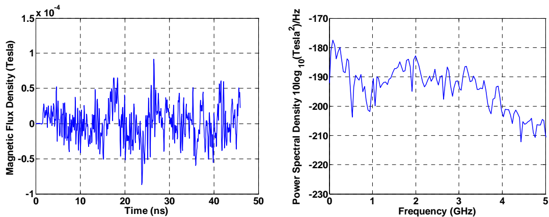
Figure 3: Time sequence of a simulation of the magnetic field due to a bunch of electrons propagating away from the laser target.
