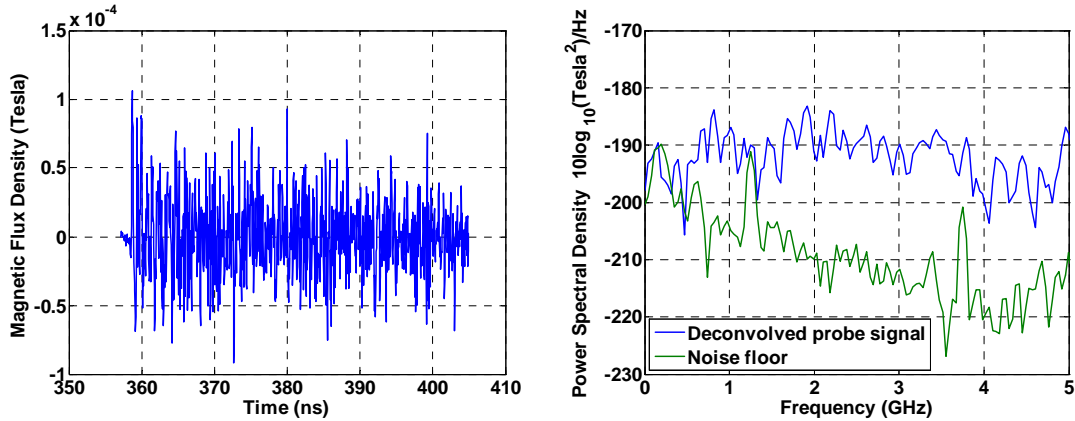
Figure 1: High-frequency B-dot probe signal and power spectral density estimate after deconvolution of probe transfer function.
