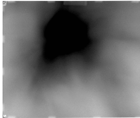
Figure 2: Spatial distribution of a high-energy beam of electrons, observed using an image plate.
