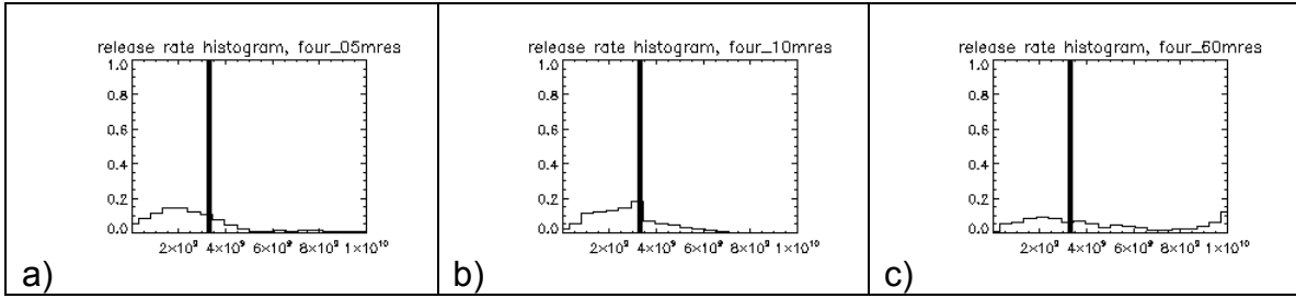
Figure 12: Histogram for release rate for simulation with sensors with a) 5-minute, b) 10-minute, and c) 60-minute time resolution
