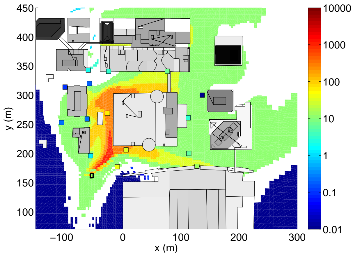
Fig. 15. Composite plume showing 90% confidence intervals for concentration levels for flow in OKC during IOP 3. Observed concentrations are also shown as small colored squares. The threshold is set at 10 ppb.
