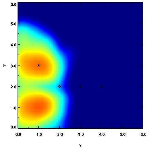
Figure 4: Bimodal posterior probability distribution of the source location for a synthetic data case using concentrations from a linear array of three sensor (black diamonds). The source location is indicated by the black dot at the coordinates (1.0, 3.0). Red color contours represent high probability density and blue color contours represent low probability density.
