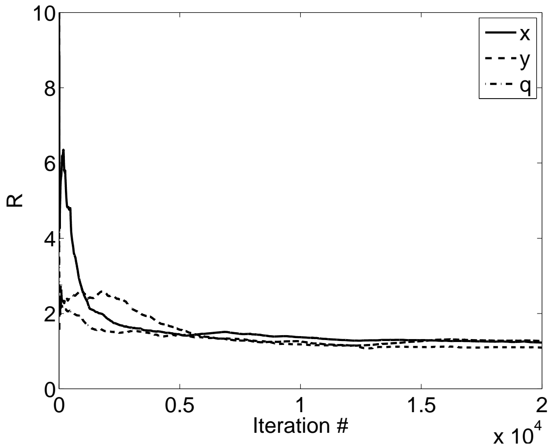
Fig. 5. Convergence rates for horizontal position (x, y) and source strength q for flow around an isolated building.
