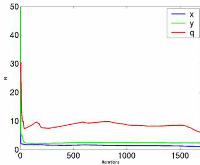
Figure 12: Convergence of x and y location, and slower conversion of strength q for the Oklahoma City example.
