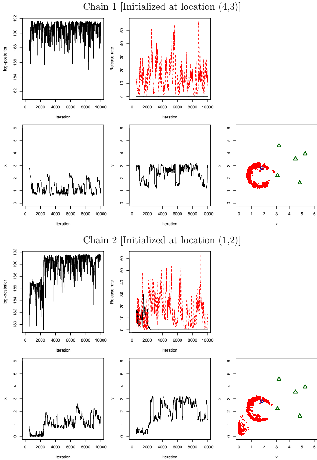
Figure 4: MCMC summary for two chains. Shown is the trace of the log-posterior distribution (up to an unknown additive constant), the trace of the release rate parameters, the trace of the x and y components of the source location, and finally a plot of the sampled source locations along with the location of the sensors and the true location of the source.
