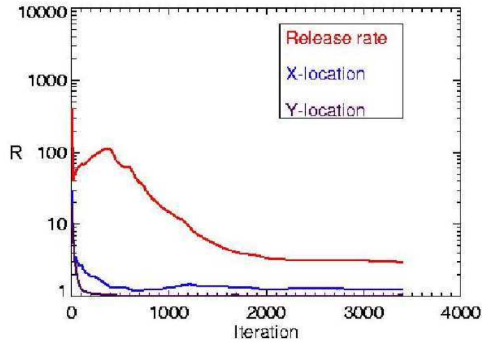
Figure 15: Statistical convergence measure, R , of stochastic procedure as a function of the number of iterations.
