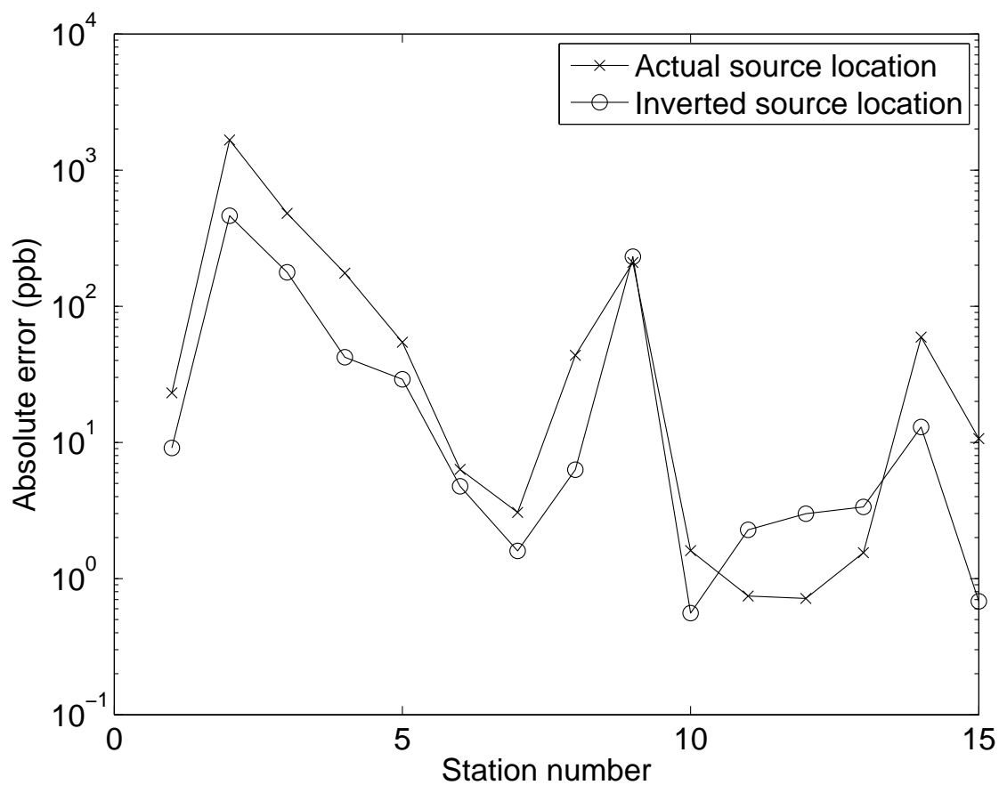
Fig. 14. Absolute error of FEM3MP predictions compared to observed concentrations at the 15 sensor locations for actual and inverted source locations.
