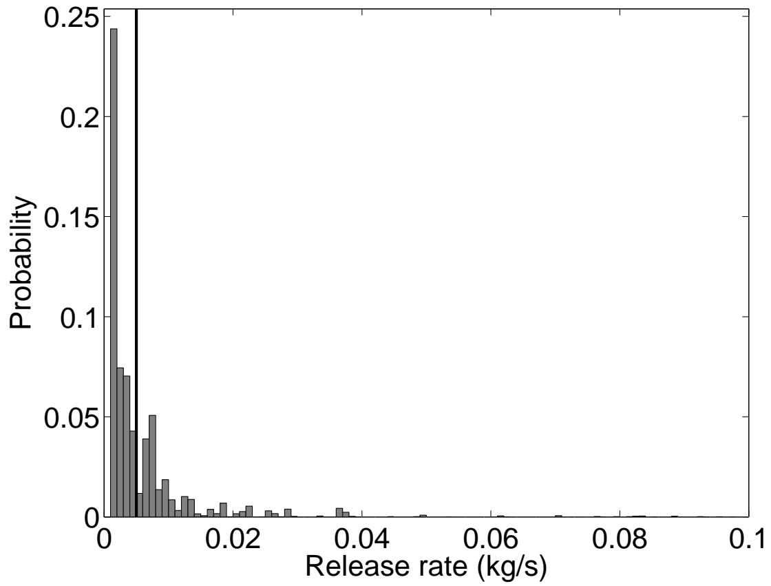
Fig. 10. Histogram of source strengths for flow in OKC during IOP 3. Solid vertical line shows magnitude of actual release rate.
