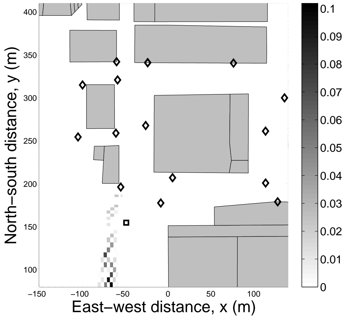
Fig. 9. Probability distribution of source location for flow in OKC during IOP 3. Only sub-domain indicated by dashed line in Fig. 8 is shown. Actual source location is shown by black square. Buildings are shaded in gray.
