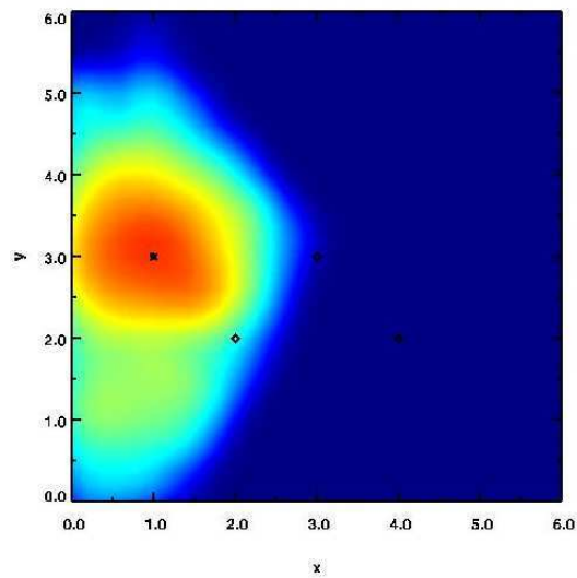
Figure 6: Posterior probability distribution of the source location for a synthetic data case using concentrations from a triangular sensor array. Red color contours represent high probability density and blue color contours represent low probability density.
