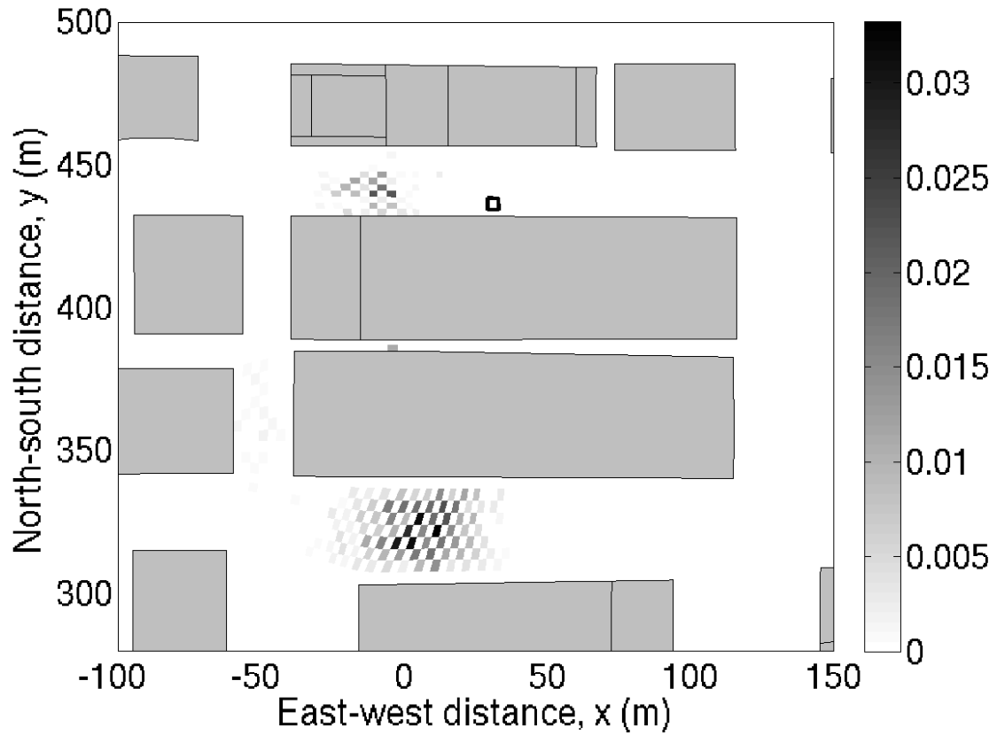
Fig. 18. Conditional probability distribution of source location for flow in OKC during IOP9 with source strength values within 50% of true value.
