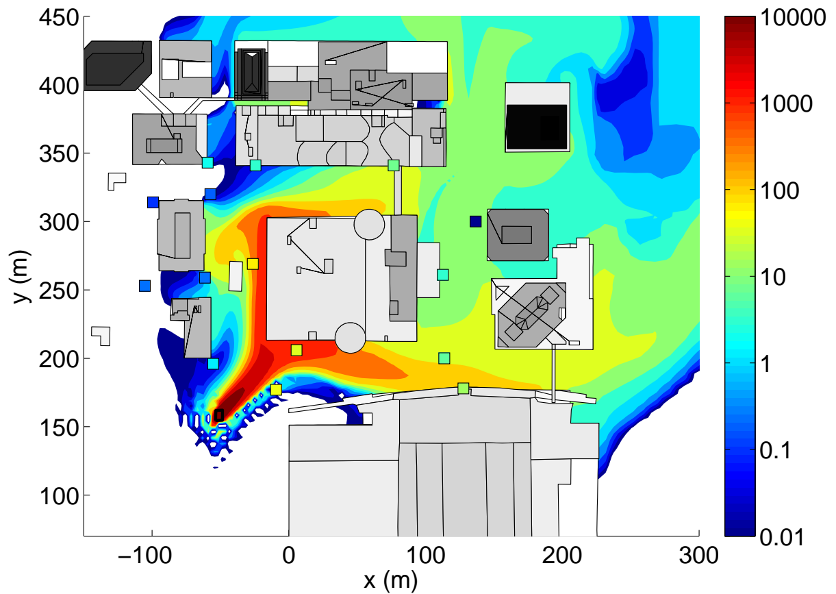
Fig. 12. Concentration plume predicted by FEM3MP with actual source location (small black square) and release rate for OKC IOP 3 compared to averaged concentration measurements (small squares colored by concentration value).
