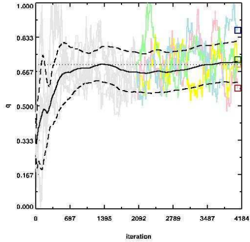
Figure 3: Source release rates for a synthetic case based on concentrations from a four-sensor square array using four Markov chains. Dotted line - actual release rate; solid line - mean of reconstructed release rates from four Markov chains; colored lines - release rates corresponding to each Markov chains; dashed lines - \pm one standard deviation from the mean value (solid line).
