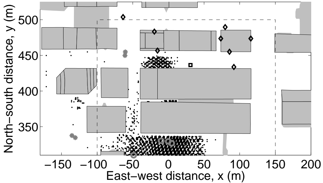
Fig. 16. Black dots show locations sampled by the four Markov chain used for source inversion for flow in Oklahoma City during IOP9. Black diamonds indicate sensor locations. Black stars show the random starting points of the Markov chains. Small black square shows true source location. Buildings that are treated explicitly are outlined in black in addition to shading; others are treated as virtual buildings. Dashed line shows zoomed-in region near the source used for later figures.
