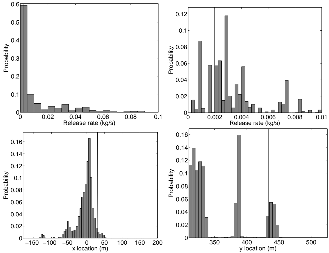
Fig. 19. Histogram of source strengths and x , y positions for flow in OKC during IOP 9. Vertical solid lines denote release rates and location coordinates of actual source.
