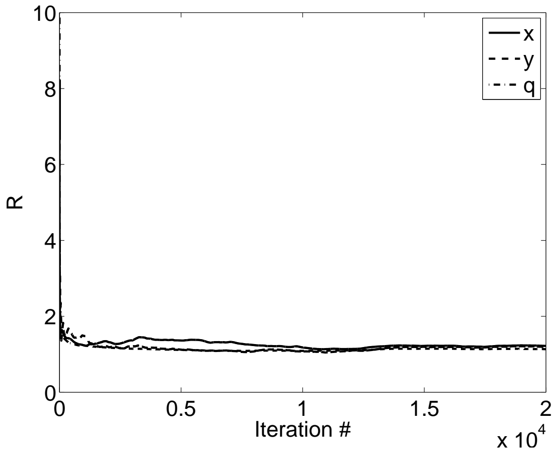
Fig. 11. Convergence rates for horizontal position ( x, y ) and source strength ( q ) for flow in OKC during IOP 3.
