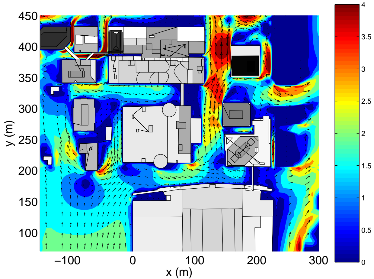
Fig. 7. Surface wind vectors (every third point shown in each direction) and contours of velocity magnitude (m/s) predicted by FEM3MP for flow in the central business district of Oklahoma City during IOP 3 of the Joint URBAN 2003 field experiment. Buildings are indicated with various shades of gray.
