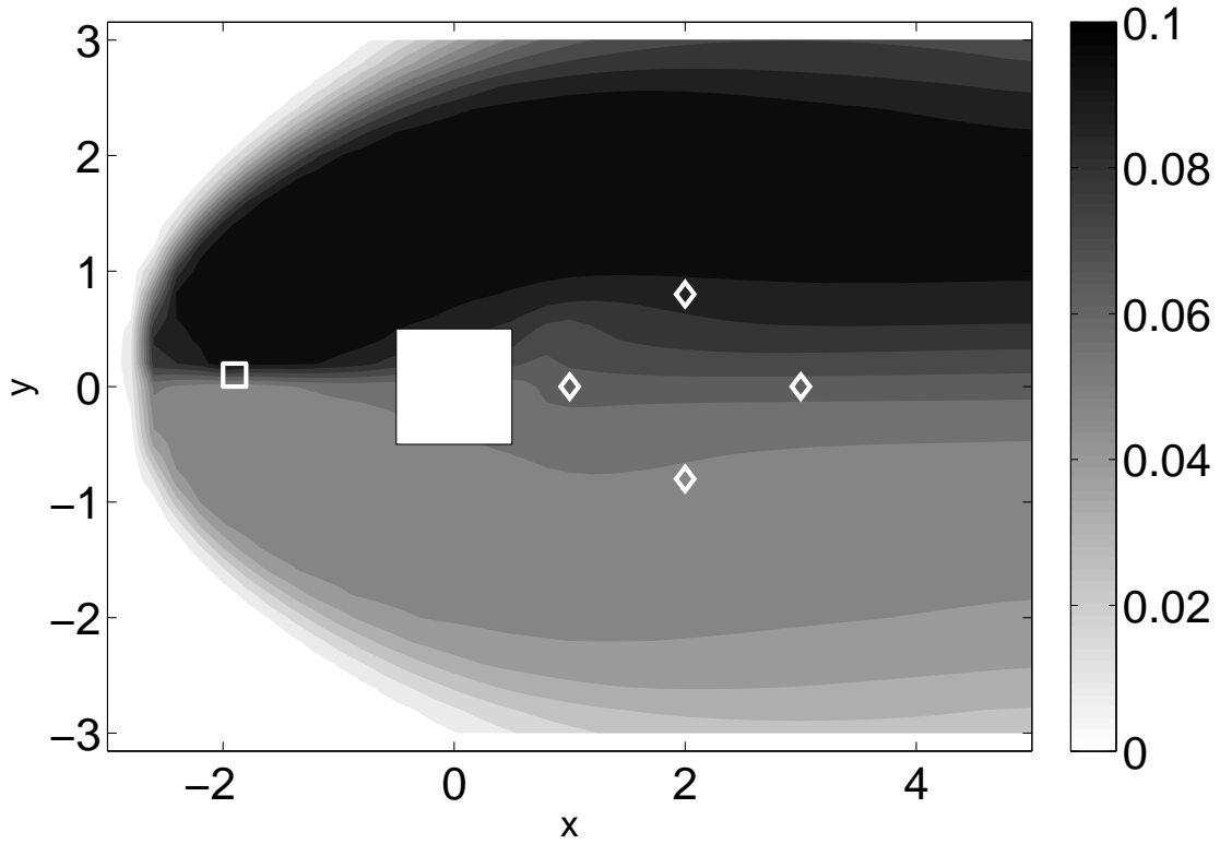
Fig. 1. Horizontal concentration contours at the first vertical level generated by forward simulation with FEM3MP for flow around an isolated building (white box). Four sensors are placed in the lee of the building (white diamonds). The source location is indicated by the white square.
