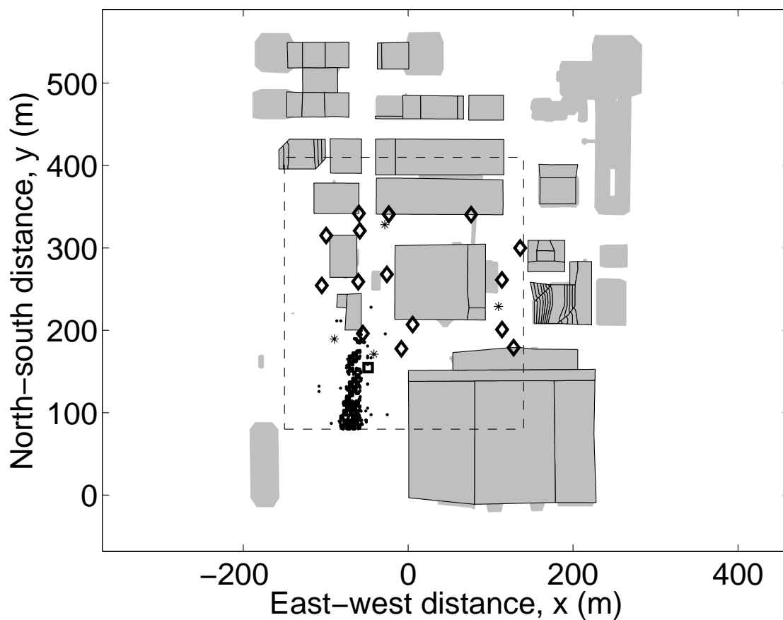
Fig. 8. Black dots show locations sampled by the four Markov chain used for source inversion for flow in Oklahoma City during IOP3. Black diamonds indicate sensor locations. Black stars show the random starting points of the Markov chains. Small black square shows true source location. Buildings that are treated explicitly are outlined in black in addition to shading; others are treated as virtual buildings. Dashed line shows zoomed-in region near the source used for later figures.
