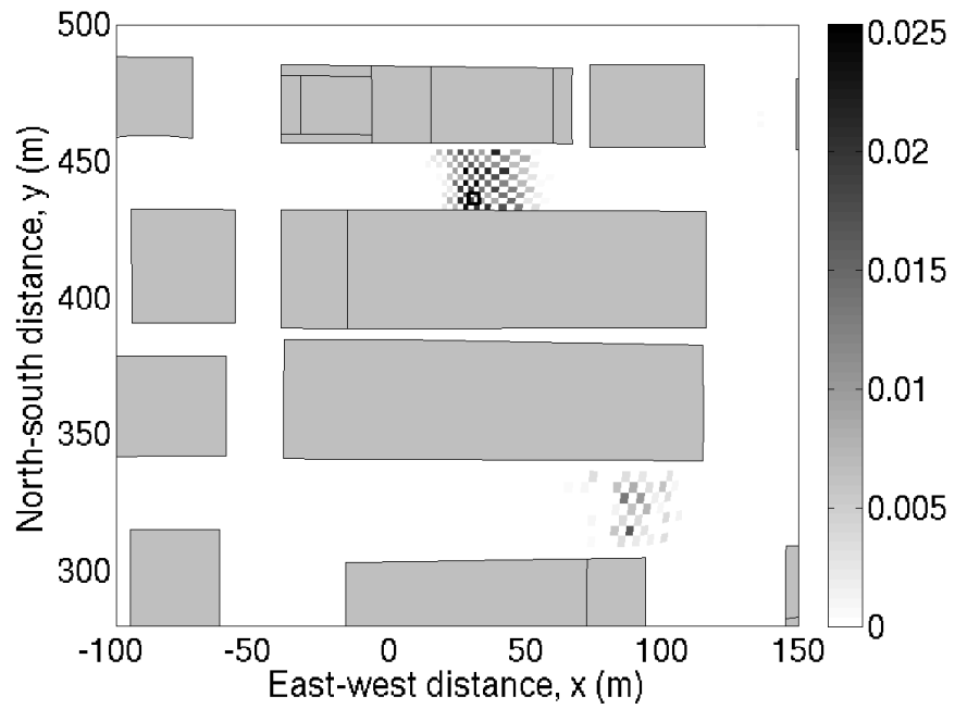
Fig. 21. Probability distribution of source location for flow in OKC during IOP 9 using synthetic sensor data generated from a forward simulation at the actual source location. As in Fig. 17.
