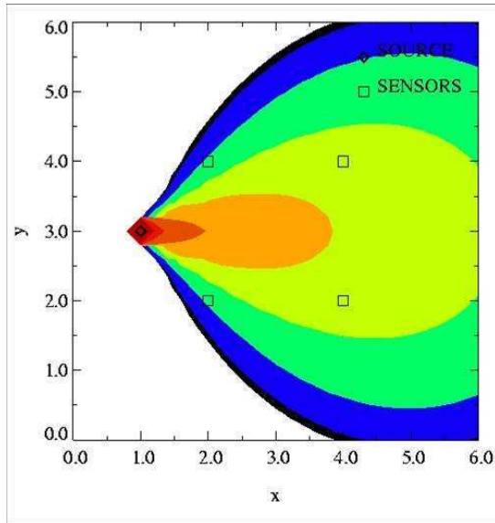
Figure 1: Plume generated with the INPUFF code and used to create synthetic sensor data. Red color contours represent higher concentration levels and blue colors reflect low concentrations.
