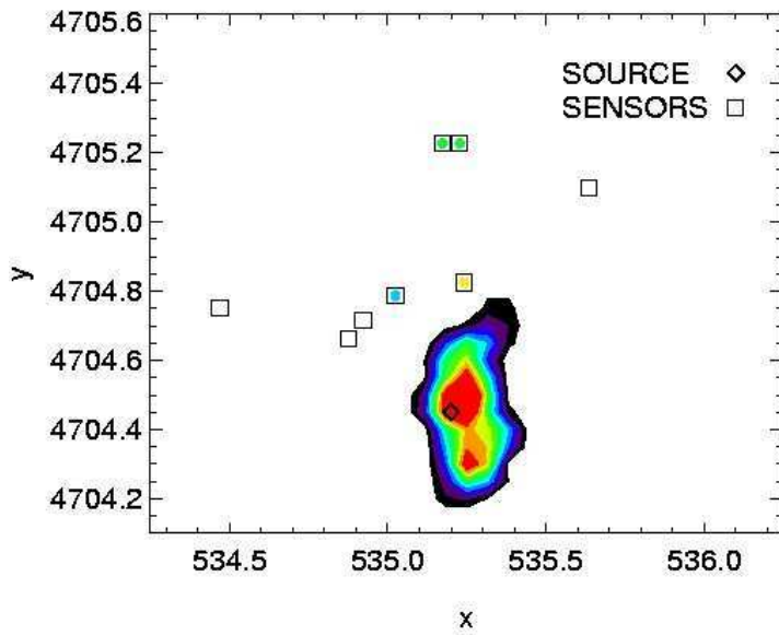
Figure 9: Conditional probability of the source location conditioned on the actual release rate for the Prairie Grass release 5. Axes and symbols are as in Figure 7. Instead of including all accepted locations, the probability contours only depict the locations from accepted proposals with source strengths close to the actual value. Warmer colors indicate higher probability; the real source location lies within the 90th percentile confidence interval.
