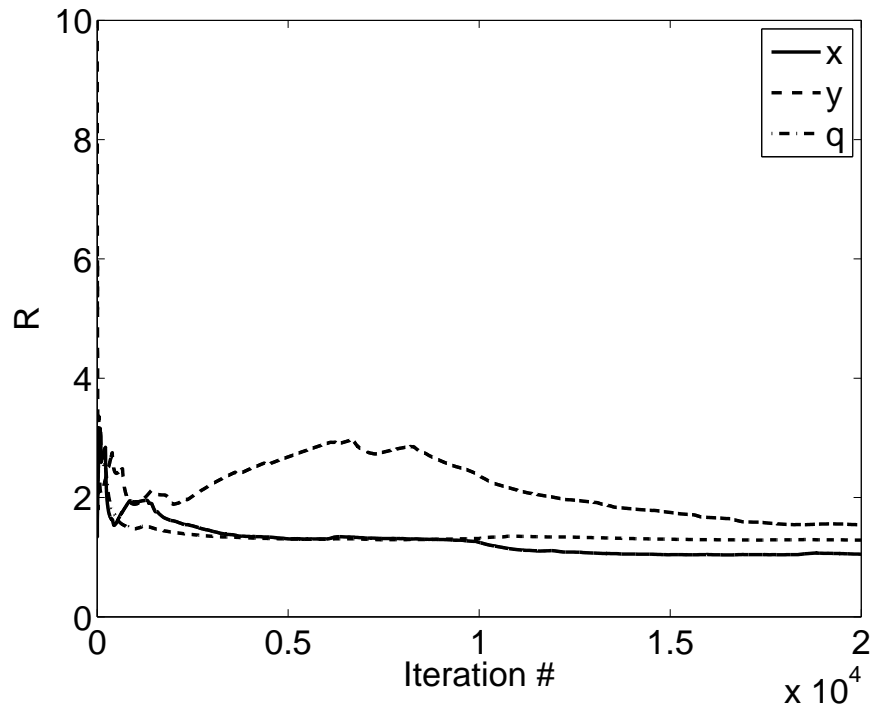
Fig. 20. Convergence rates for horizontal position (x, y) and source strength q for flow in OKC during IOP 9.
