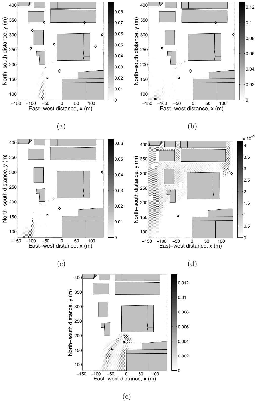
Fig. 23. Probability distribution of source location for flow in OKC during IOP 3 using 8, 4, and 2 sensors, and two different instances with 1 sensor of chosen from the original 15. Sensors chosen are shown with black diamonds. The true source is indicated by the black square.
