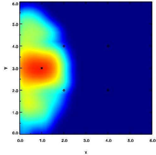
Figure 2: Posterior probability distribution of the source location for a synthetic data case using a square sensor array (four sensors, represented by diamonds). The source location is indicated by the black dot at the coordinates (1.0, 3.0). Red color contours represent high probability density and blue color contours represent low probability density.
