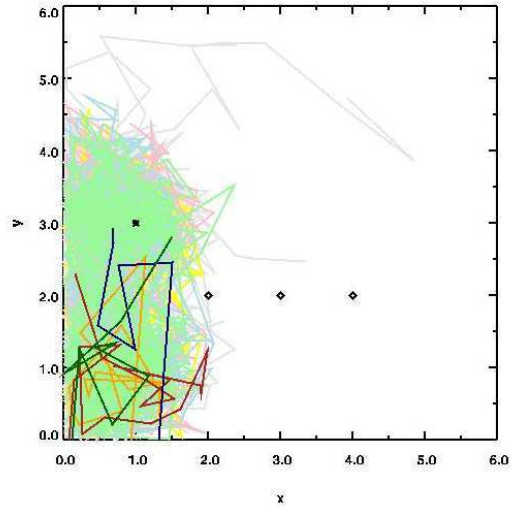
Figure 5: Markov chains explore two posterior probability distribution modes for the source location for a synthetic data case using concentrations from a linear array of three sensors. Light colors represent early stages of MCMC iteration procedure and dark colors represent late stages.
