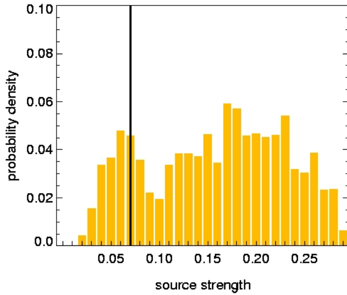
Figure 8: Probability distribution of source release rate for Prairie Grass release 5. The actual release rate was q = 0.05 g/s.
