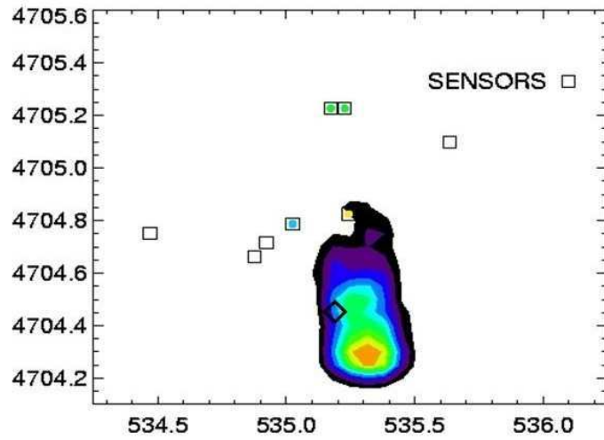
Figure 7: Probability distribution for the source location for Prairie Grass release 5. The x and y axes denote west-east and south-north location in km. Squares indicate the locations of the sensors, while the color filling the squares denotes the observed concentration (white indicates a zero observation, and blue, green, and yellow indicate low, medium, and high concentrations). The colored contours indicate the posterior probability distribution for the source location, with orange indicating the highest probability area. The actual source location, marked by a triangle, lies within the 50th percentile confidence contour.
