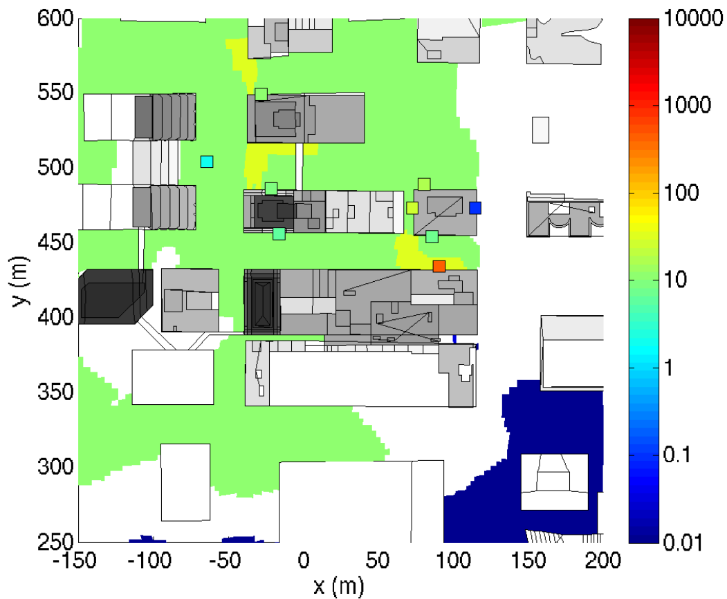
Fig. 22. Composite plume showing 90% confidence intervals for concentration levels for flow in OKC during IOP 9. Observed concentrations are also shown as small colored squares. The threshold is set at 10 ppb.
