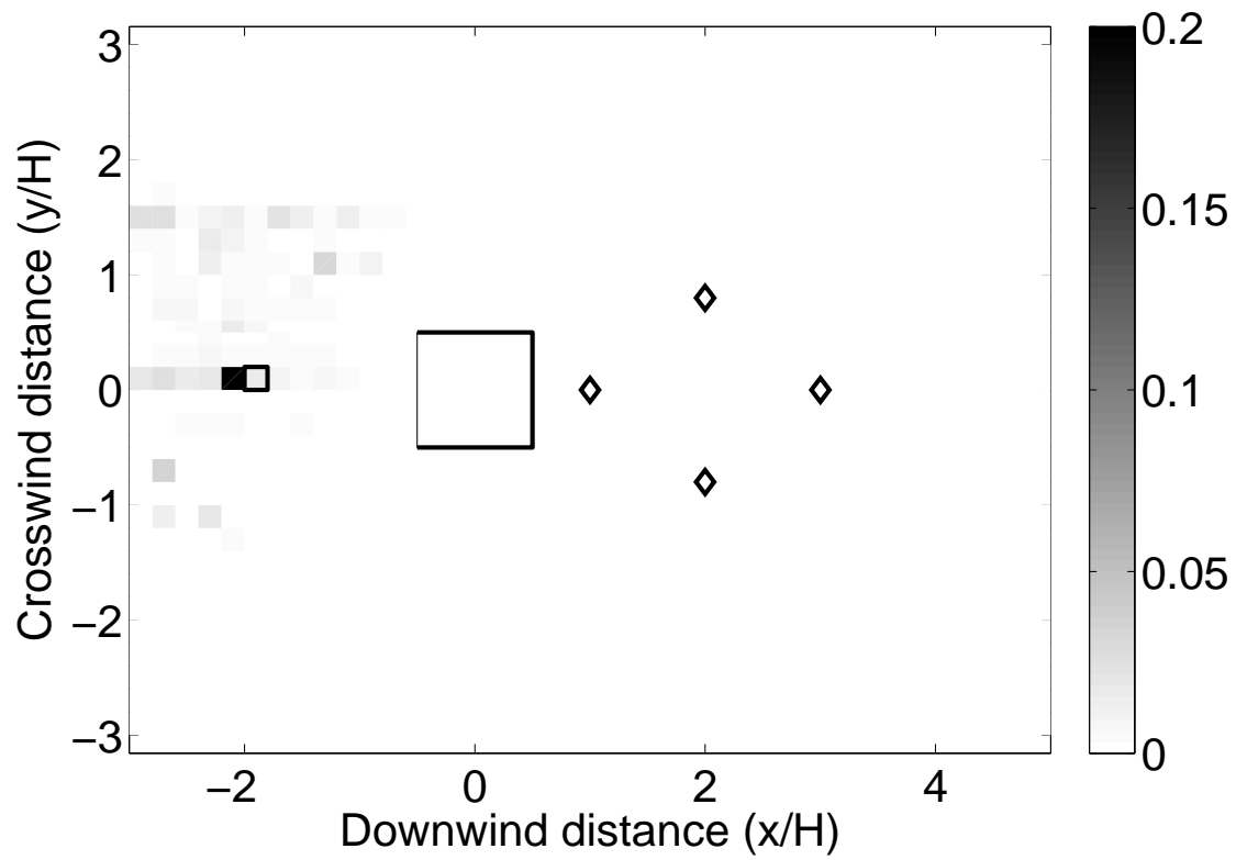
Fig. 3. Probability distribution of source location for flow around an isolated building. Black diamonds indicate the four sensor locations. Small black square shows true source location adjacent to peak of probability distribution.
