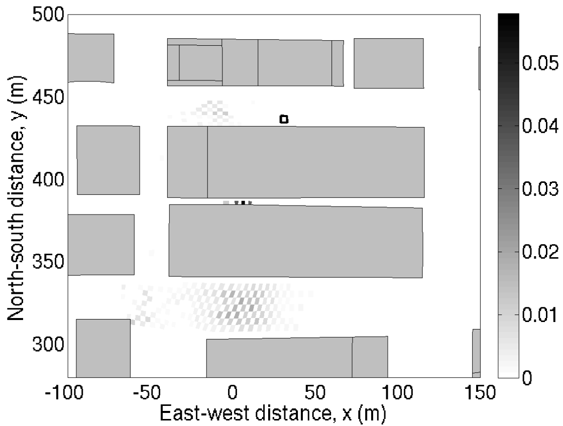
Fig. 17. Probability distribution of source location for flow in OKC during IOP 9. Only sub-domain indicated by dashed line in Fig. 16 is shown. Actual source location is shown by black square. Buildings are shaded in gray.
