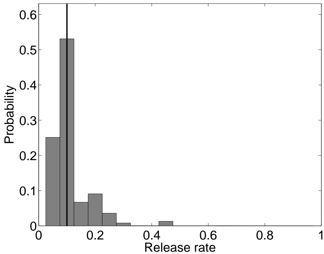
Fig. 4. Histogram of source strengths for flow around an isolated building. Solid vertical line shows actual release rate magnitude.
