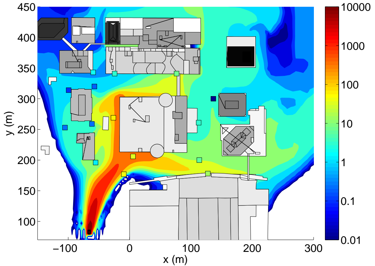
Fig. 13. As in Fig. 12 except source location and strength are from peak of reconstructed probability distribution.
