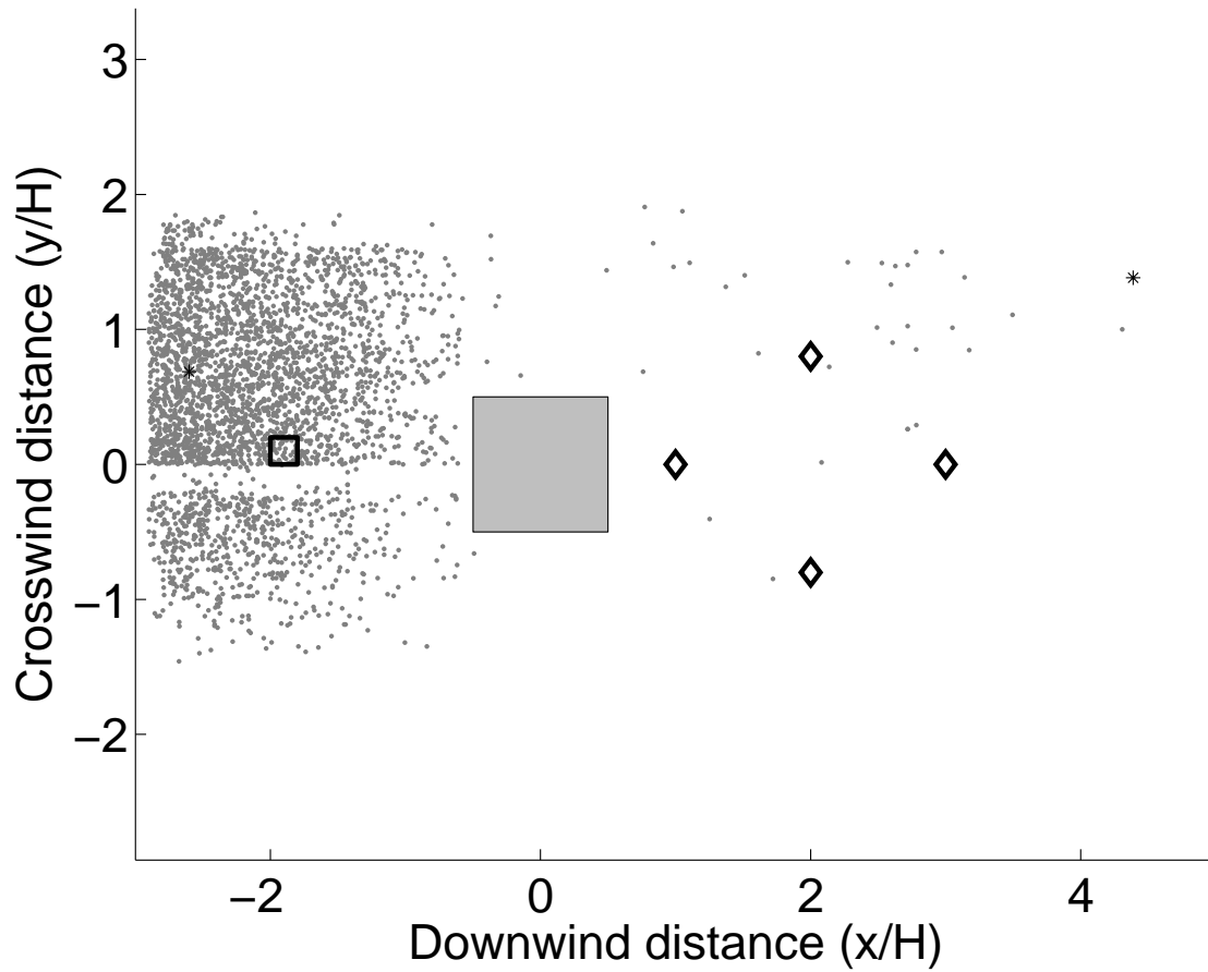
Fig. 2. Gray dots show locations sampled by the four Markov chain used for source inversion for flow around an isolated building (gray square at origin). Black diamonds indicate the four sensor locations. Black stars show the random starting points of the Markov chains (two are co-located at the origin). Small black square shows true source location.
