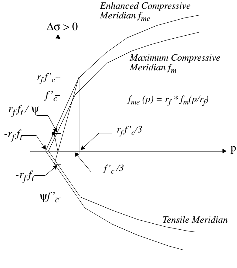
FIGURE 9. Description of strength enhancement calculation.
