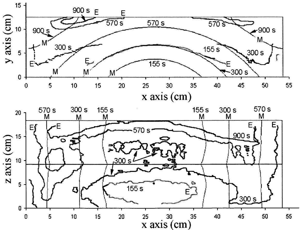
Figure 65. Predicted versus experimental results for case TA01.
