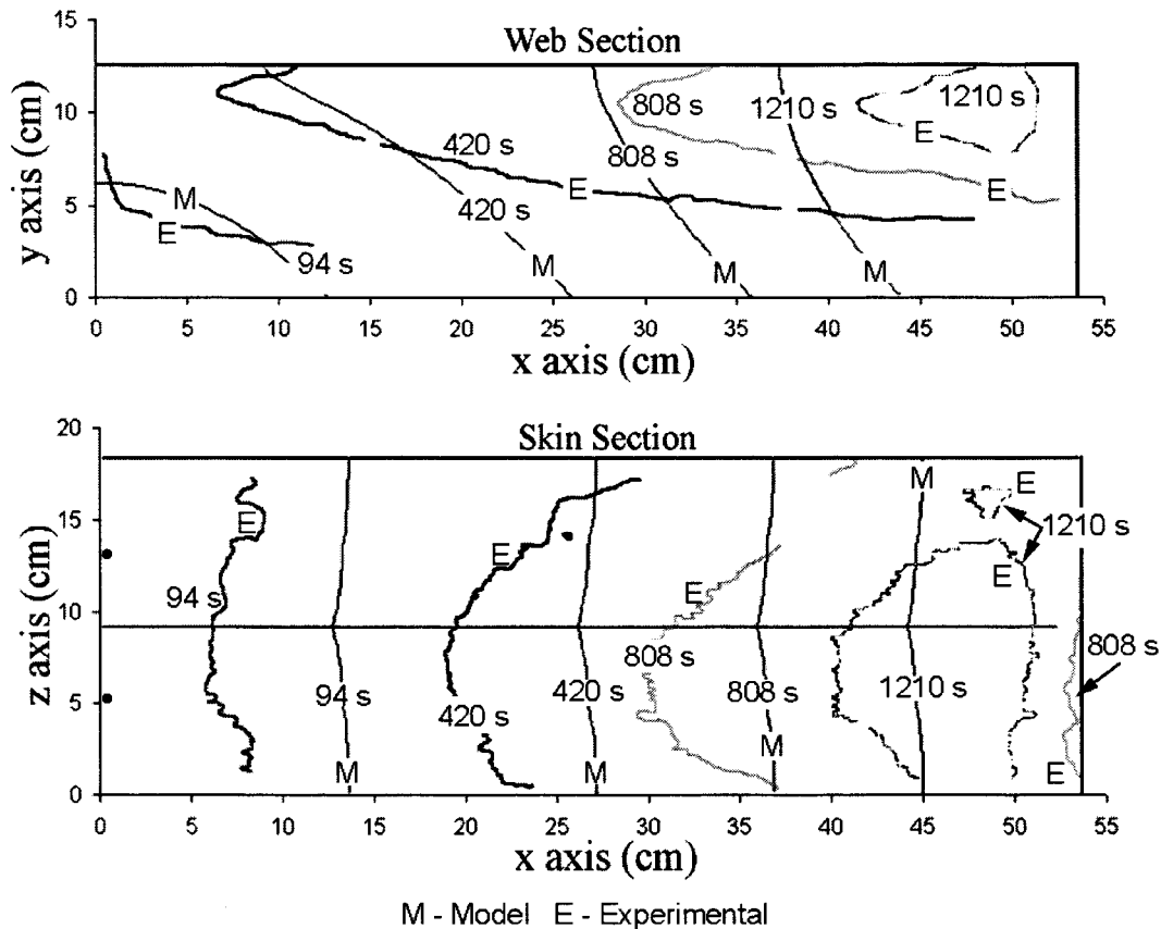
Figure 67. Experimental versus predicted results for TA02.
