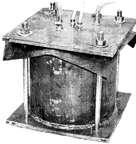
Figure 19. Pressure pot.
