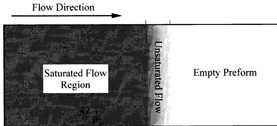
Figure 14. Three regions of flow in an RTM mold.
