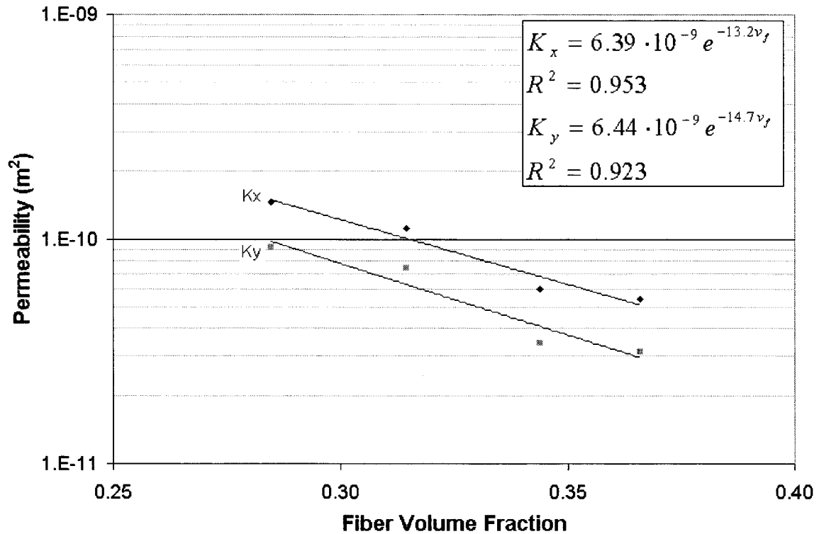
Figure 42. Permeability versus fiber volume fraction for DB120 fabric.
