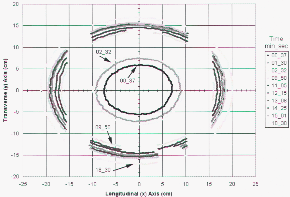
Figure 41. Contour plot for experiment SB08-1. Times are listed in minute_second format on the legend. The lay-up consisted of 8 layers of DB120 fabric with a fiber volume fraction of 0.31.
