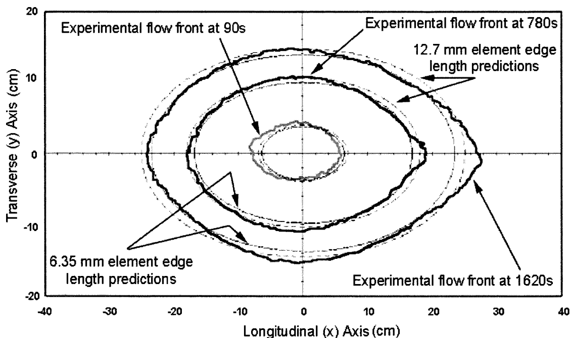
Figure 60. Experimental versus predicted flow front positions for SA08-1, single fabric A130. K_x=9.90 \times 10^{-11} K_y=3.47 \times 10^{-11} , \nu_f=0.400 , \mu=0.195 kg/m·s and P=89.7 kPa.
