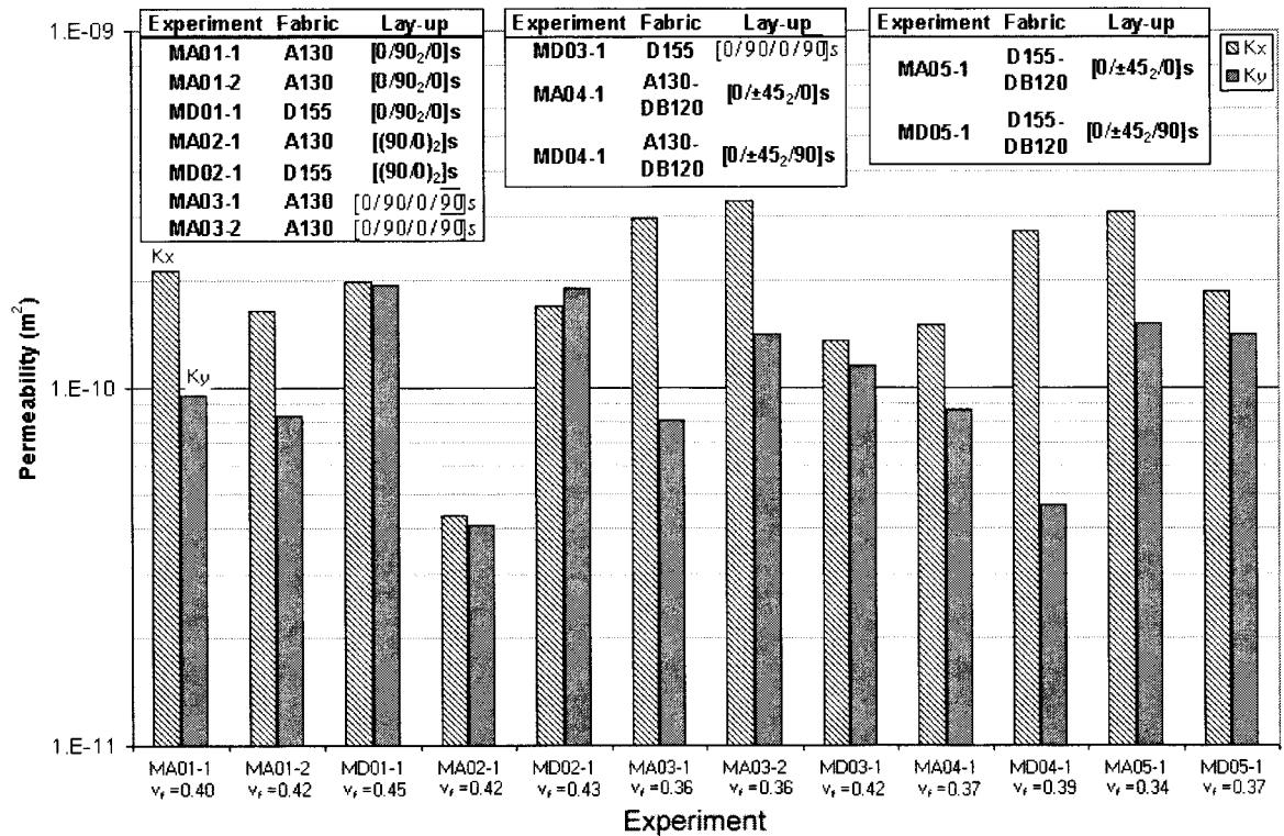
Figure 48. Transverse and longitudinal permeabilities for mixed fabric experiments.
