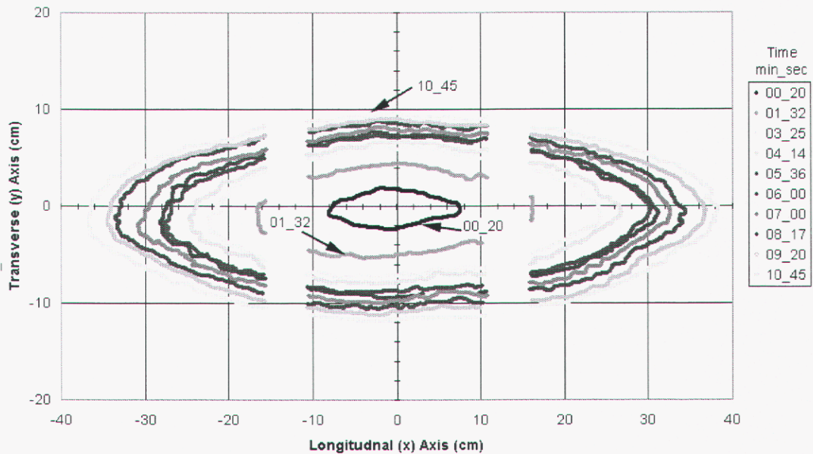
Figure 43. Contour plot for experiment SD06-1. Times are listed in minute_second format on the legend. The lay-up consisted of 6 layers of D155 fabric with a fiber volume fraction of 0.40. Fibers aligned with x-axis.
