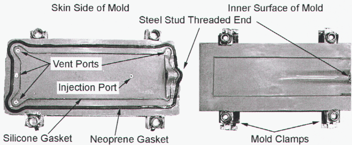
Figure 23. Skin and inner-surface halves of the steel insert mold.
