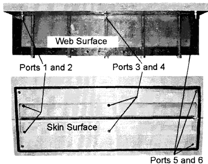
Figure 22. T-section mold.
