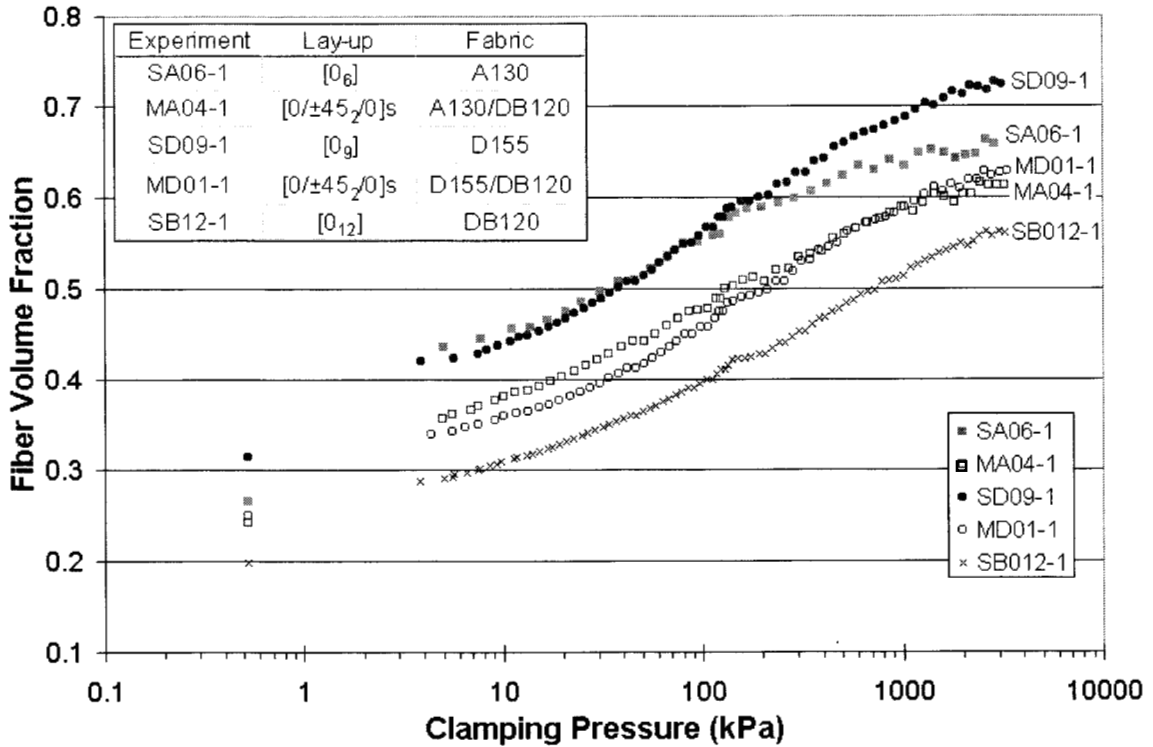
Figure 38. Effect of mixed fabrics on fiber volume fraction.
