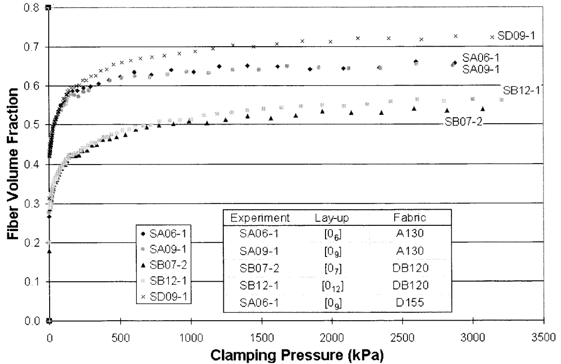
Figure 35. Compressibility of unidirectional A130, DB120 and D155 fabrics.
