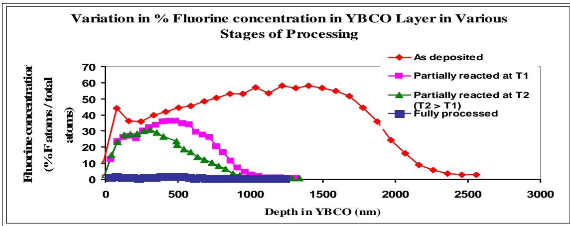
Figure 3: Variation in % Fluorine concentration in YBCO layer in various stages of processing
