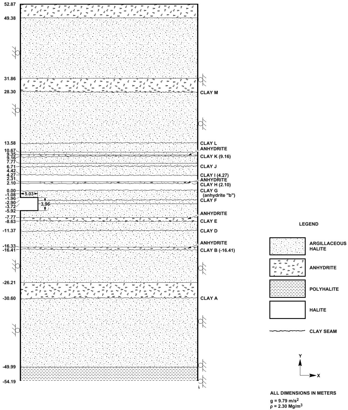
Figure 4: Idealized stratigraphy near the disposal room horizon defined by Munson et al. (1989)
