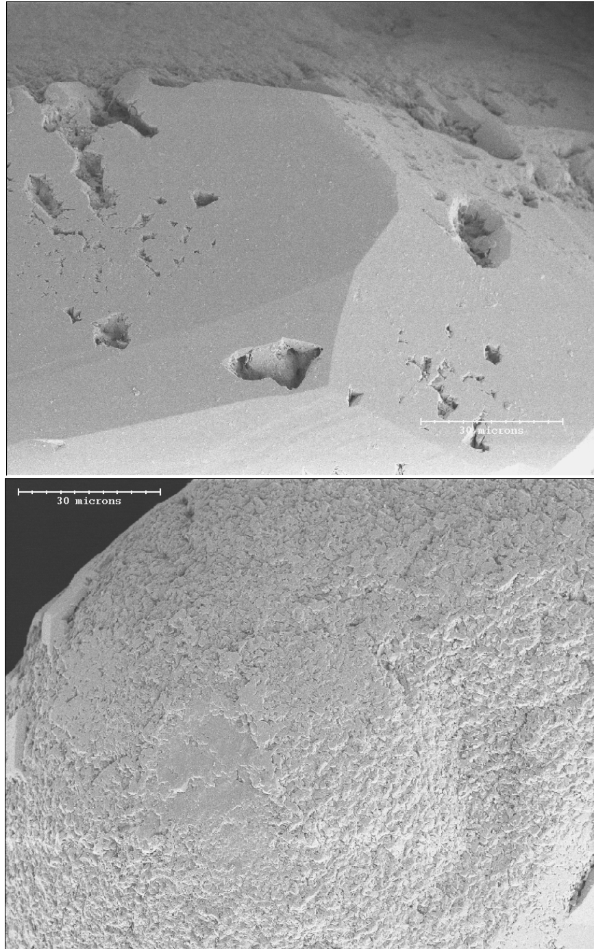
Figure 3.3 Backscattered electron micrographs showing the bimodal morphology of Arizona magic sand. Grains are smooth and faceted (top), or alternatively rough and irregular (bottom).
