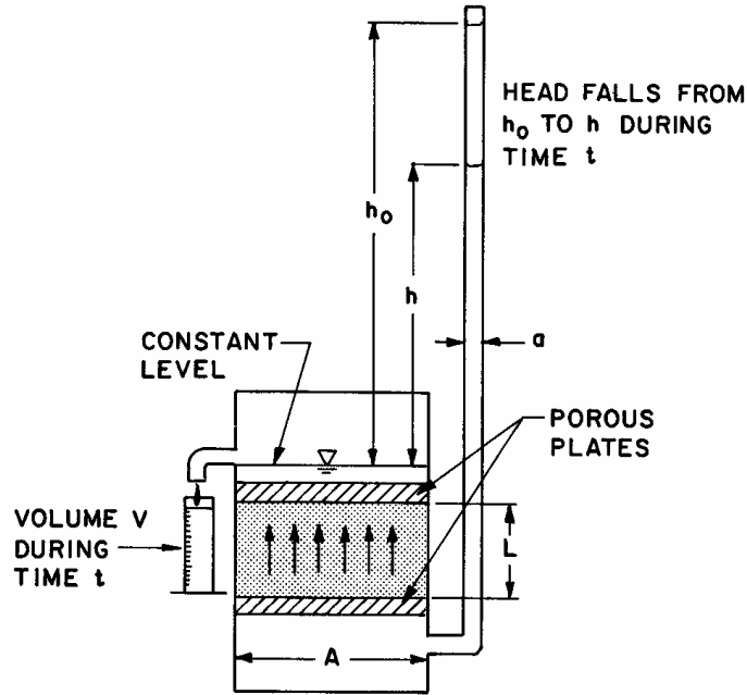
Figure 3.2 Falling head permeameter testing configuration (after Dullien, 1992).
