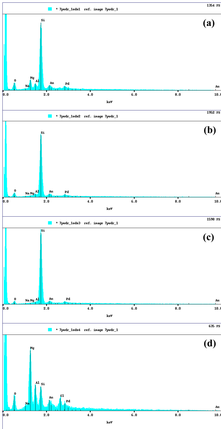
Figure 3.8 Spectra collected from powdered region from LDH precipitation experiment AZ-7. A light gold-palladium film coats all samples as required in scanning electron microscopy. (Top) The signal for Mg and Al is moderate as are the Au-Pd peaks. (Middle) The Mg/Al signal from these two regions is minimal, indicating possible lack of coverage or incomplete formation of LDH. (Bottom) The signal here is strong and in the proper ratio (2:1) of the precursor solutions. The presence of the chlorine peak suggests that this area contains remnants of the unreacted precursor solution.
