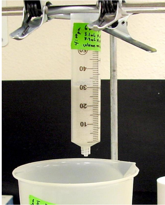
Figure 3.1 Experimental setup for column mixing experiments and permeability testing. A plastic beaker below the column collects solutions that exit the column.
