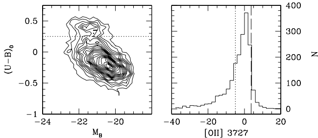
FIG. 1.— Left panel: Restframe color-magnitude diagram of 17,745 DEEP2 galaxies. Our sample of RSGs is defined by U-B > 0.25 (objects above the dotted line). Right panel: A histogram of [OII] \lambda 3727 EWs for RSGs. Because the [OII] line is overimposed to strong absorption lines, EW=0 is not achieved for zero emission. Instead, no [OII] emission happens when EW[OII]=3.7 \text{ \AA} (dashed line, Konidaris et al. in preparation), with emission line galaxies having lower EWs. All galaxies with EW[OII] \leq -5 \text{ \AA} (dotted line) are excluded from the sample.
