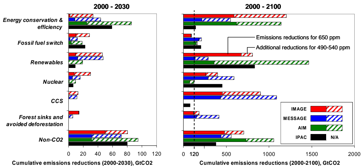
20 Figure SPM 9: Cumulative emissions reductions for alternative mitigation measures for 2000 to 2030 (left-hand panel) and for 2000-2100 (right-hand panel). The figure shows illustrative scenarios from four models (AIM, IMAGE, IPAC and MESSAGE) aiming at the stabilization at 490-540 ppm CO 2 -eq and levels of 650 ppm CO 2 -eq, respectively. Dark bars denote reductions for a target of 650 ppm CO 2 -eq and light bars the additional reductions to achieve 490-540 ppm CO 2 -eq. Note that some models do not consider mitigation through forest sink enhancement (AIM and IPAC) or CCS (AIM) and that the share of low-carbon energy options in total energy supply is also determined by inclusion of these options in the baseline. CCS includes carbon capture and storage from biomass. Forest sinks include reducing emissions from deforestation. [Figure 3.23] 25
