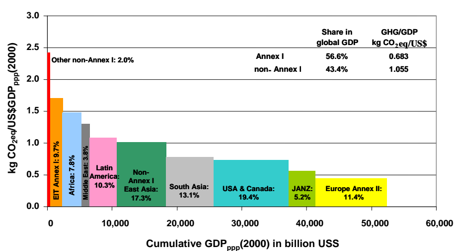
Figure SPM 3b: Year 2004 distribution of regional GHG emissions (all Kyoto gases, including those from land-use) per US$ of GDP over the GDP of different country groupings. The percentages in the bars indicate a regions share in global GHG emissions [Figure 1.4b].
