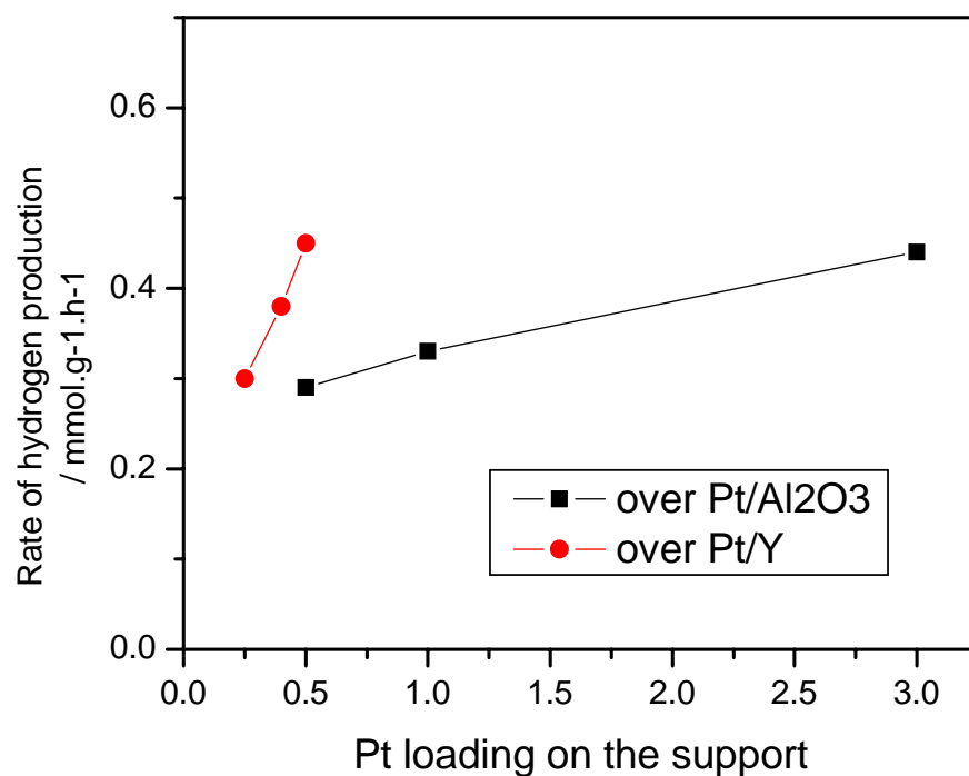
Figure 16. Hydrogen production rate as a function of Pt loading. Solid circles are for Pt/ \gamma -Al 2 O 3 catalysts with Pt loads of 1/2%, 1%, 3 wt%; Solid squares are for Pt/NaY catalysts with Pt loads of 0.25%, 0.4% and 0.5%; reaction conditions: 493 K, 2.6 Mpa, WHSV=0.008 h -1 , with 1 wt% methanol solution feed.)
