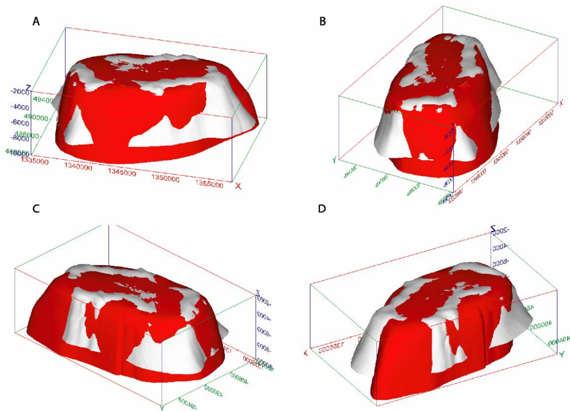
Figure 19. Comparison of the original (gray) and updated (red) West Hackberry salt dome models in perspective view. View from azimuths of (a) 165°, (b) 240°, (c) 315°, (d) 30°. Elevation is 30° above the horizontal. No vertical exaggeration.
