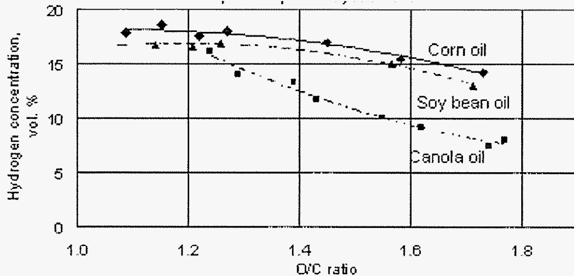
Figure 8.28. Hydrogen concentration for catalytic reformation of corn oil, soybean oil and canola oil.
