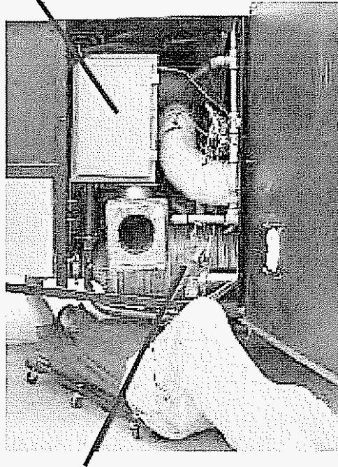
Figure 4.15 Picture of part of plasmatron diesel reformer system in the back of the bus
