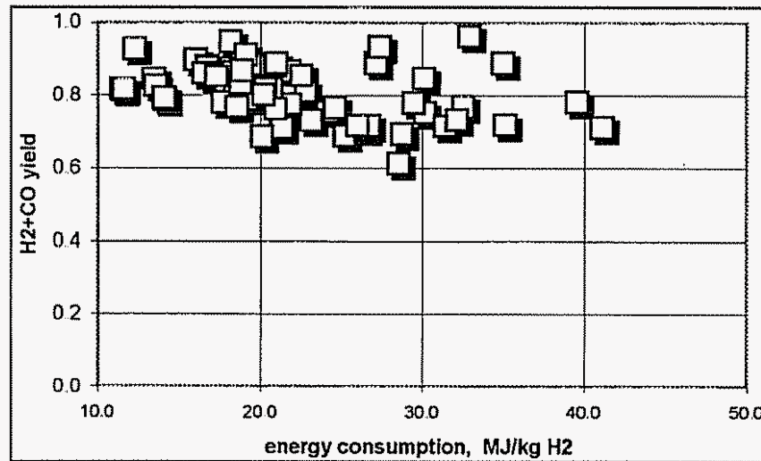
Figure 8. Hydrogen and CO yield (for complete PO stoichiometric conversion) as a function of specific energy consumption for plasma catalytic reforming of methane.
