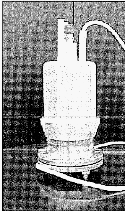
Figure 2.7. Gen H plasmatron developed at ARM.
