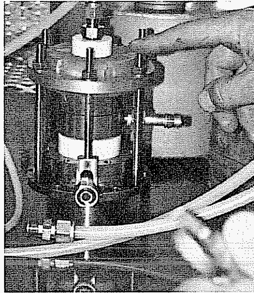
Figure 4.2. Compact low power plasmatron fuel converter used for these tests
