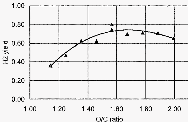
Figure 4. Hydrogen yield for the plasma-catalytic reformation of ethanol vs. O/C ratio
