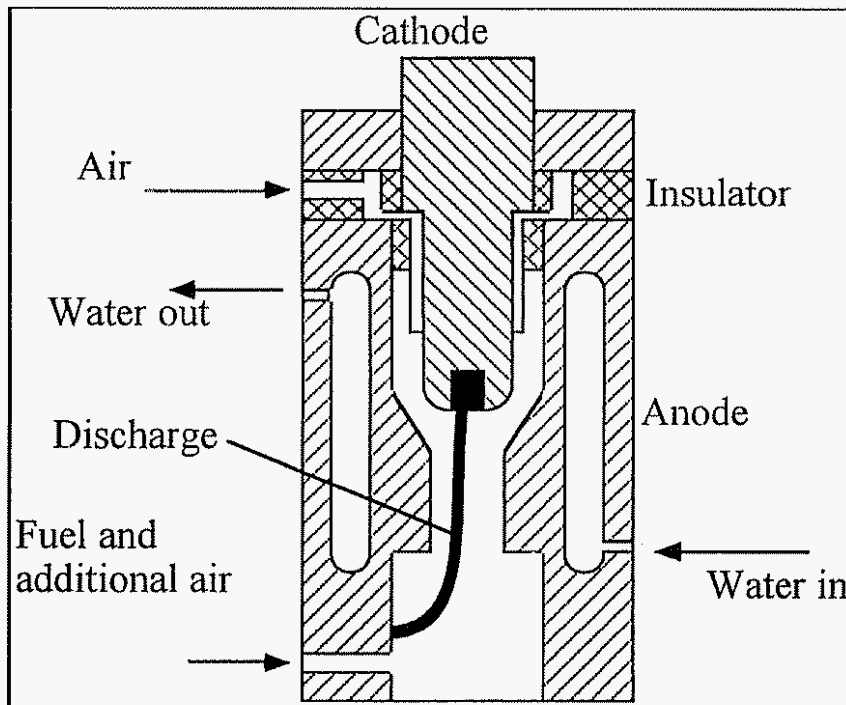
Figure 1. Thermal arc plasmatron
