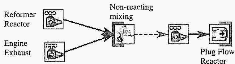
Figure 5.10. System without equilibrium reactor for reformer.
