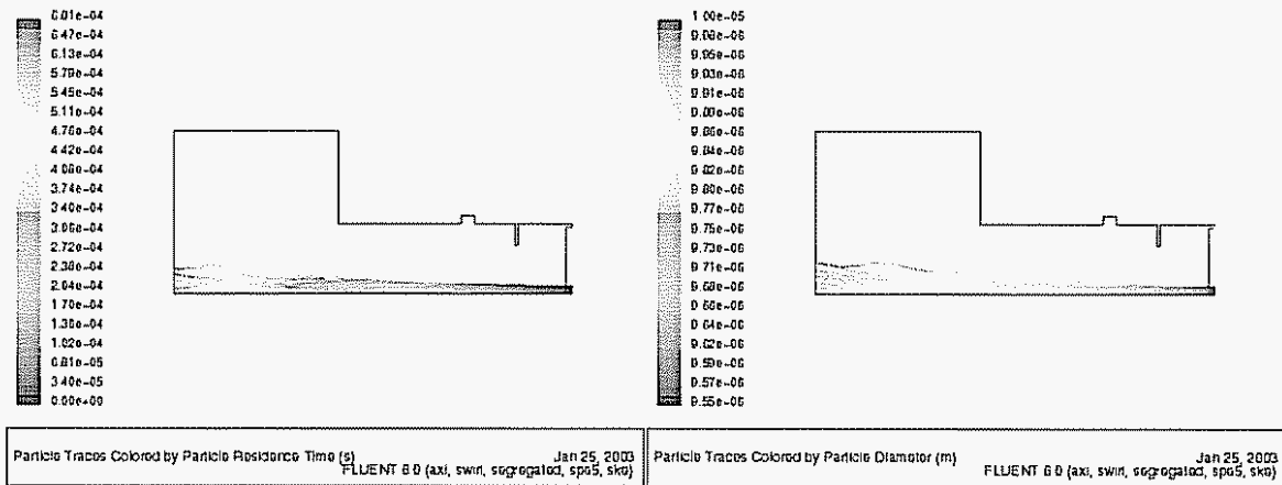
Figure 7.14. Stochastic particle path vs (a) residence time (b) particle diameter
