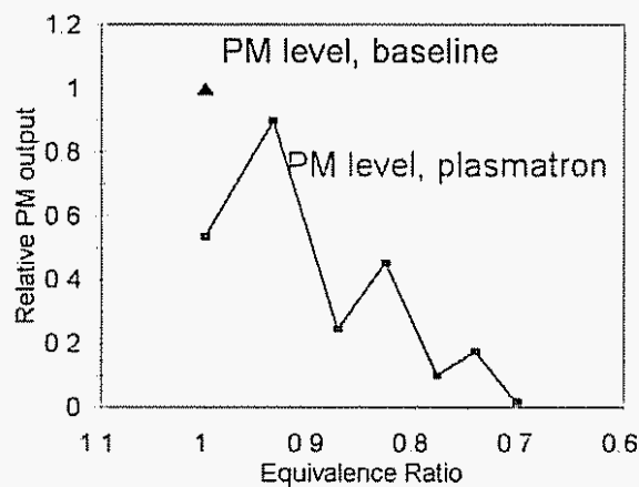
Figure 3.7. Relative PM emissions as a function of equivalence ratio (1500 rpm, 2.6 bar BMEP).
