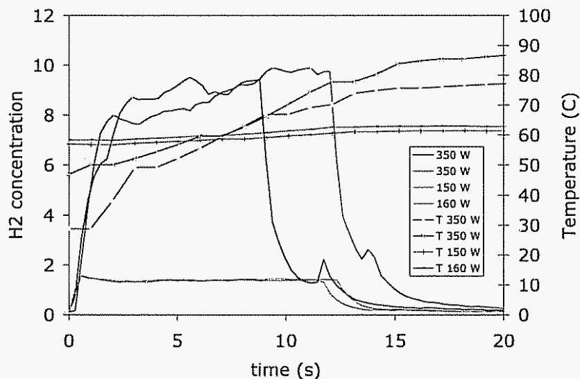
Figure 8.21. Transients for the case of propane/air premixed, resulting in a homogeneous air/fuel mixture.
