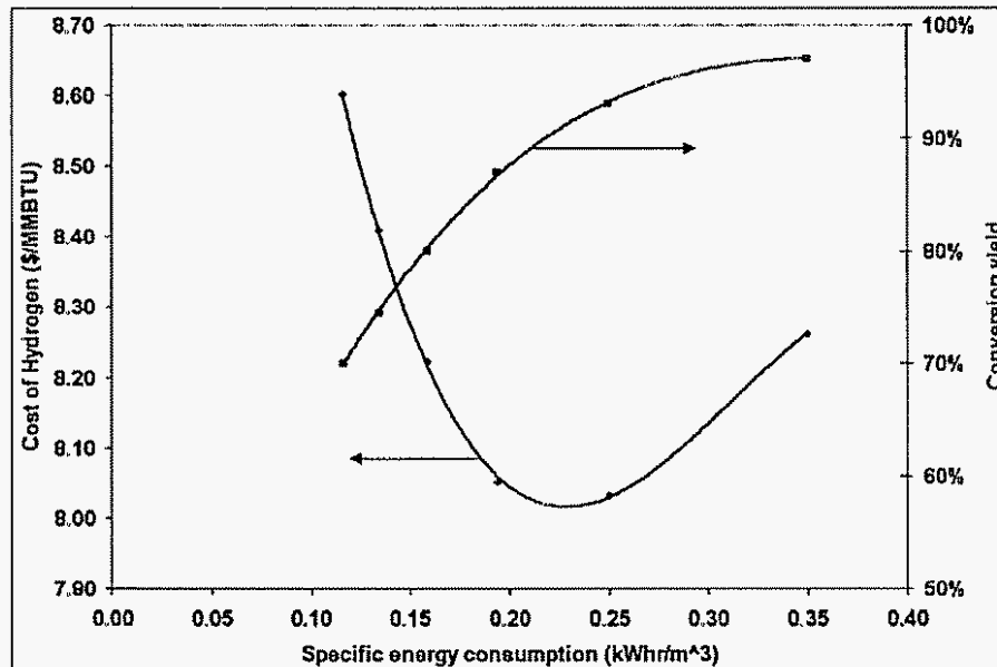
Figure 9 Methane yield and cost of hydrogen as a function of the specific energy, for 571 m 3 =h plant capacity
