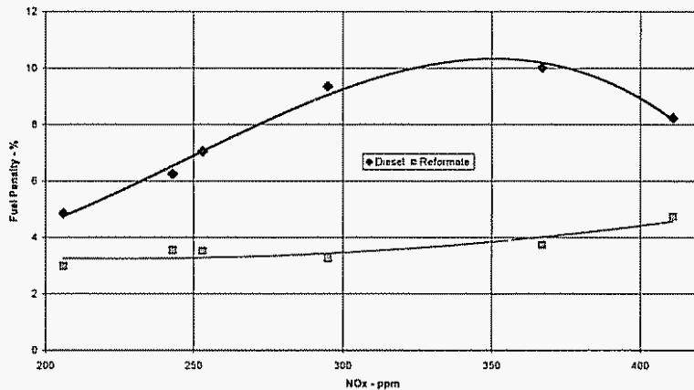
Figure 4.11. Fuel penalty for ECS Modes, at same NO x adsorption
