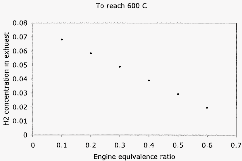
Figure 5.5. Hydrogen concentration in exhaust if reformat reaches equilibrium in the reformer, as a function of the engine equivalence ratio.
