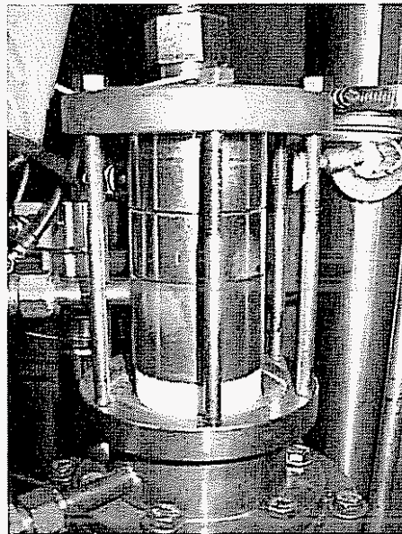
Figure 2.6. Photograph of plasmatron fuel reformer used for experiments with propane, natural gas, gasoline and bio fuels during the last year of the program (gen 3a)
