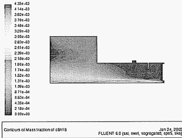
Figure 7.13. Mass fraction of Gaseous C8H18 (relative to nitrogen)
