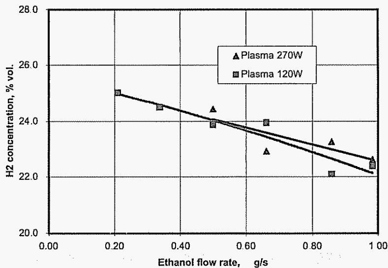
Figure 4.4. Hydrogen concentration in dry gas for ethanol reforming, as a function of flow rates, for O/C ~ 1.2
