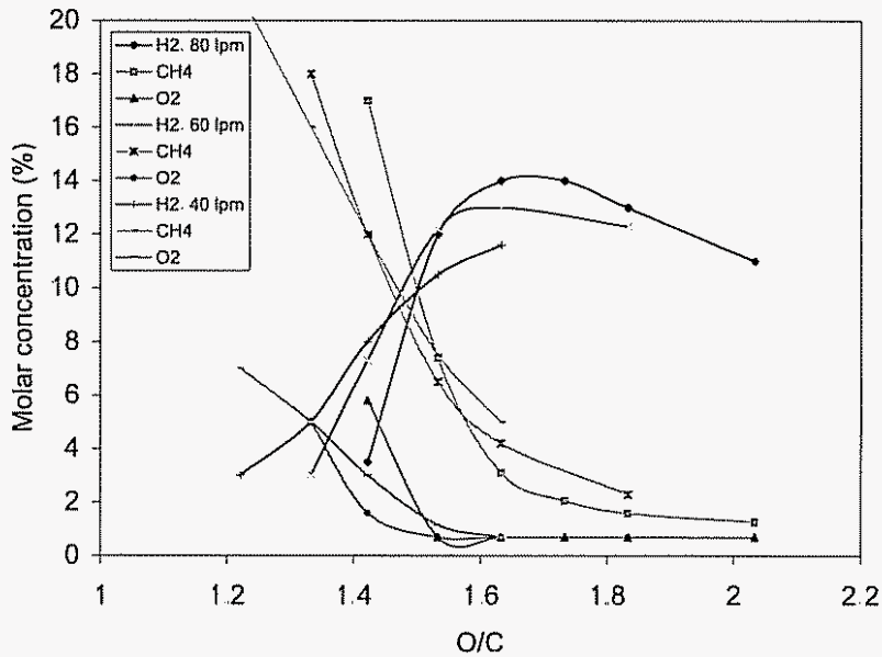
Figure 7.27. Experimental results (from reference [PSR9]),
