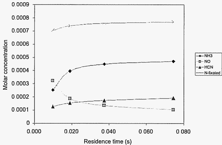
Figure 7.25. Molar concentration of fixated nitrogen.
