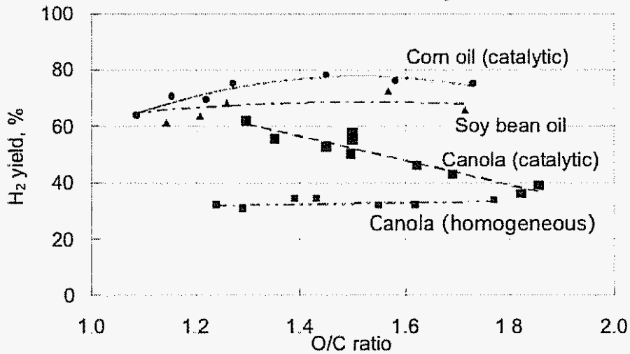
Figure 8.26. Hydrogen concentration for catalytic reformation of corn, canola and soy bean oils
