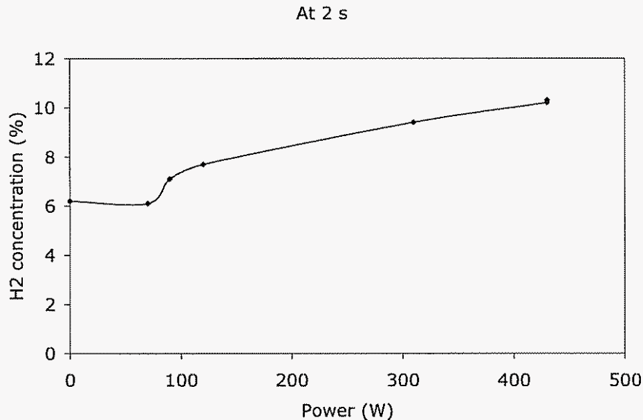
Figure 9.5. H 2 concentration at 2 s as a function of plasma power at fixed O/C.
