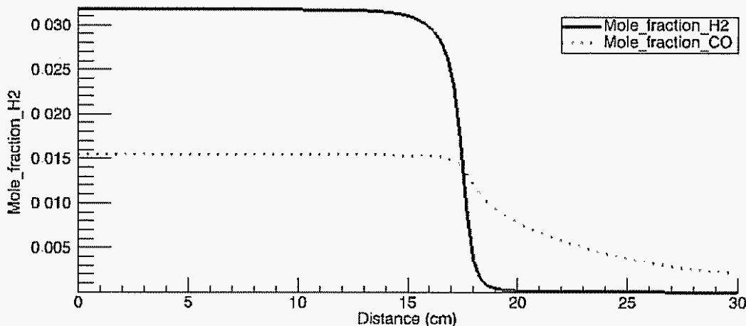
Figure 9. Hydrogen and CO concentration of the gas in the PFR as a function of distance, for the case of engine exhaust temperature of 973 K.
