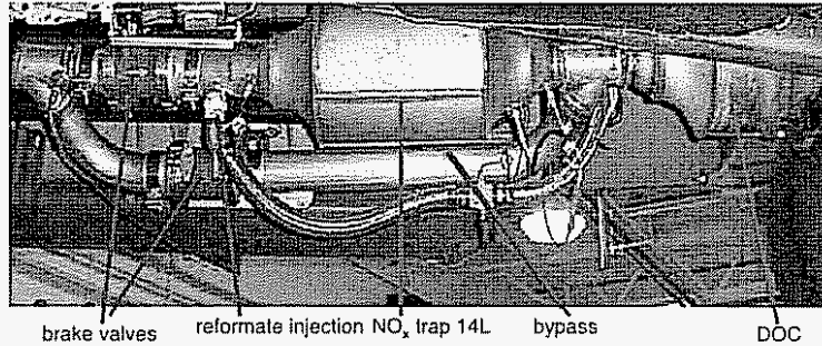
Figure 4.13. F250 hydrogen assisted NO x trap installation
