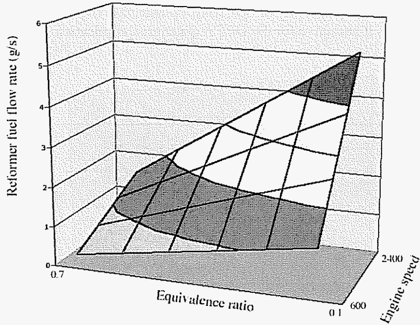
Figure 5.4. Rate of fuel flow rate through the reformer (in g/s) required to achieve regeneration conditions as a function of the equivalence ratio and the engine speed, for 3-bar inlet manifold pressure.
