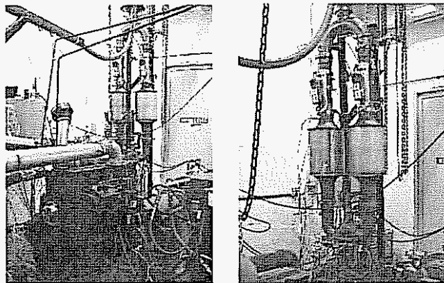
Figure 4.5. Test set-up for hydrogen assisted NO x traps
