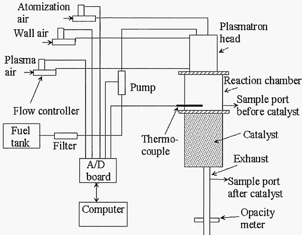
Figure 3.3 Schematic layout of the reformer setup
