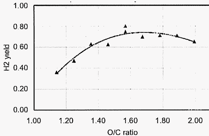
Figure 8.29. Hydrogen yield for catalytic reformation of ethanol as a function of O/C ratio.
