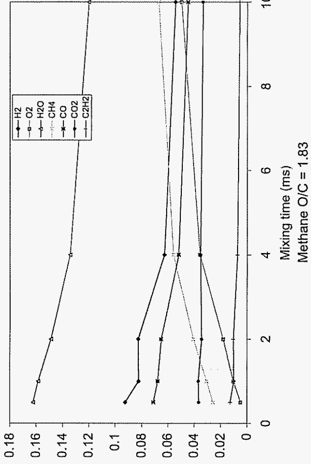
Methane O/C = 1.83
