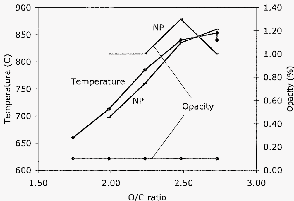
Figure 8.26 Temperature and opacity for the same cases as Figure 8.25. NP stands for No-Plasma.
