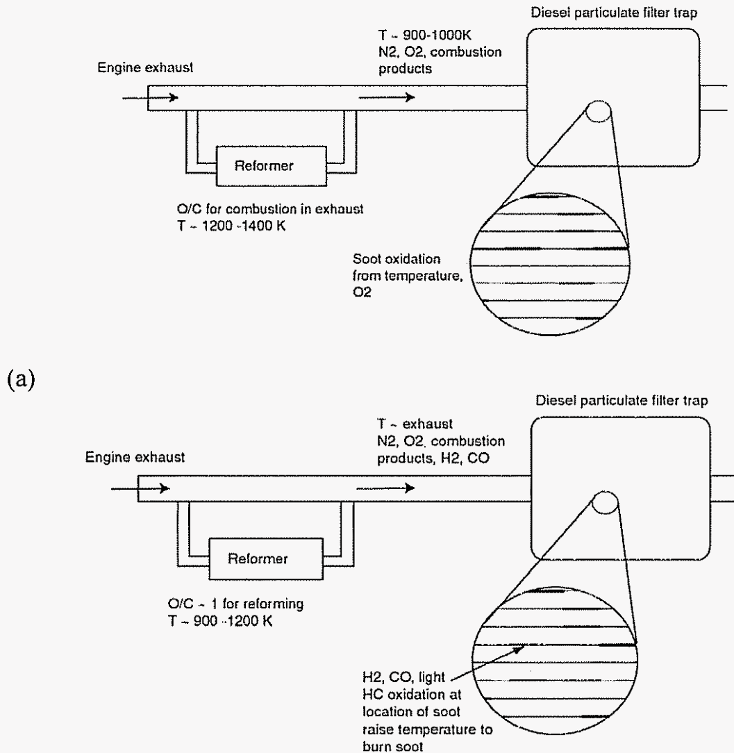
(b) Figure 5.1. Reformer operating as a (a) combustion for DPF regeneration (b) Generation of hydrogen rich gas
