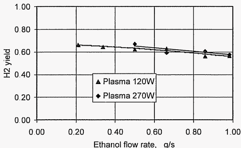
Figure 5. Hydrogen yield vs. ethanol flow rate for plasma-catalytic reforming
