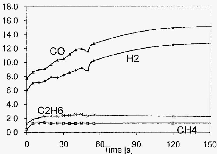
Figure 6. Concentration of H 2 , CO and C 2 H 6 in the reformat as a function of time for homogeneous reforming, with variable O/C ratio during the first 12 seconds.
