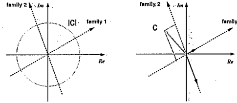
Figure 1: Left: complex plane with the measured |C| and the directions of the two corrector families. Right: case with measurement of C , its decomposition along the two lines and corresponding correction setting.
