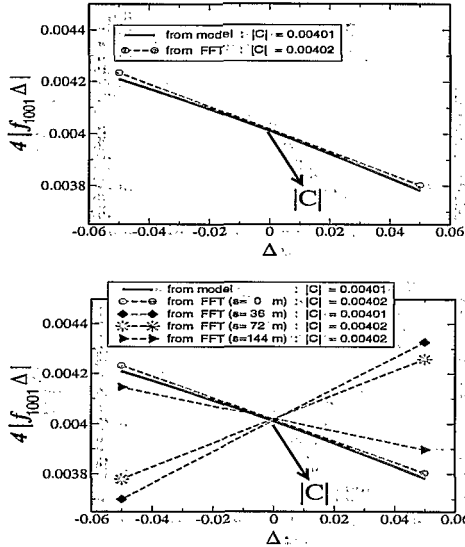
Figure 2: Examples of |C| inferred from two simulated measurements of |f_{1001}| according to Eq. (5) at one location (top) and at several locations (bottom).
