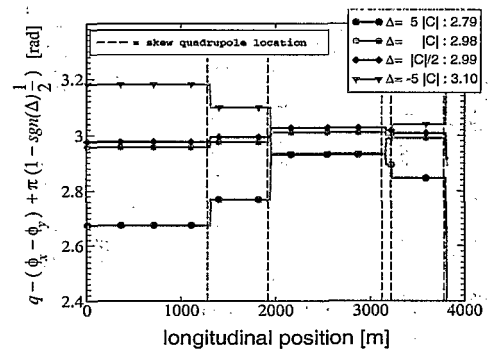
Figure 3: MADX tracking simulation of the RHIC Yellow ring at injection energy with betatron coupling |C| = 0.01 : the quantity q^w - (\phi_x^w - \phi_y^w) + \pi (1 - \text{sgn}(\Delta) \frac{1}{2}) at the BPM locations is plotted for different working points.
