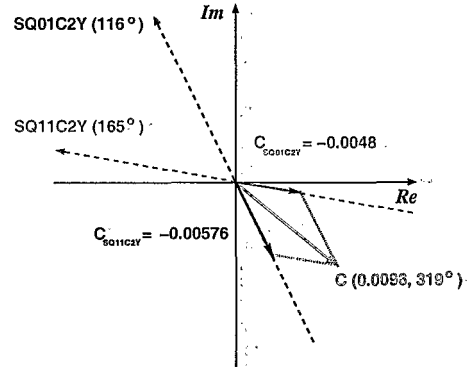
Figure 5: Sketch of the measured C decomposed on the axes defined by the two skew quadrupoles used for correction.
