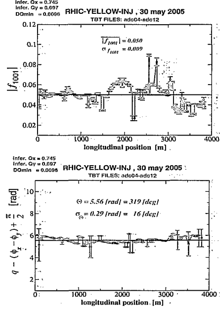
Figure 4: Variation along the Yellow ring at injection of |f_{1001}| (top) and q_x - (\phi_x^w - \phi_y^w) - \text{sgn}(\Delta) \frac{\pi}{2} (bottom). The corrector skew. Data points (i.e. BPMs) with fluctuation larger than 30% were rejected.
