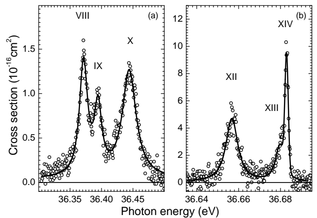
FIG. 7: Voigt line profile fits (full lines) to high resolution measurements (open symbols) in the photon energy ranges 36.3–36.5 eV (a) and 36.635–36.695 eV (b). From the fit (a) the experimental energy spread \Delta E = 1.87 \pm 0.08 meV is obtained. The same value has been used and kept fixed in fit (b). Further fit results are summarized in Table II where the resonances are labeled by Roman numerals.
