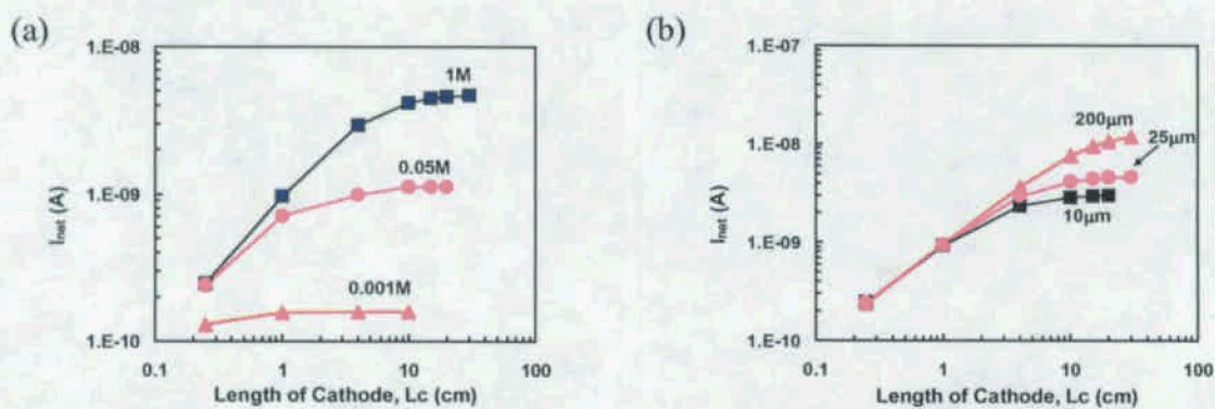
Figure 11. Total net cathodic current I_{net} got saturated as length of cathode increased to a critical value. The speed of saturation depends highly on [Cl] and slightly on WL: a) all cases had a constant WL of 25µm; b) all cases had a constant [Cl] of 1M, values kinetic parameters are the same as those used in the base cases.
