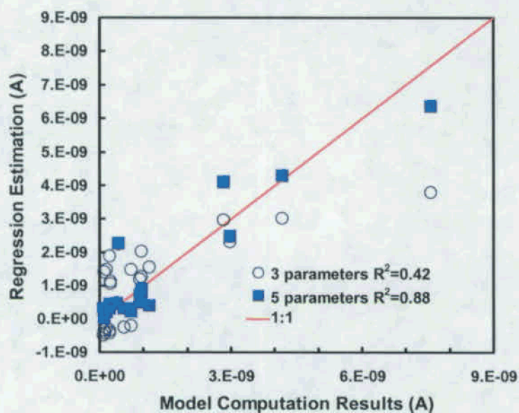
Figure 10. Regression fitting of the computation data using three main factors (WL, Lc, and [Cl]) and 5 factors (WL, Lc, [Cl], WL x Lc, Lc x [Cl]): 5 factors fitting gave better correlation with respect to model data.
