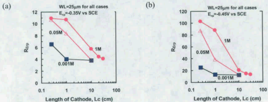
Figure 8. Effect of E_{rp} , as described by R_{E_{rp}} = I_{net}(E_{rp} = -0.35 \text{ or } -0.45\text{V}) / I_{net}(E_{rp} = -0.25\text{V}) : a) E_{rp} = -0.35\text{ V} ; b) E_{rp} = -0.45\text{ V} . Regardless of [\text{Cl}] , R_{E_{rp}} tends to asymptote to \sim 4 ( E_{rp} = -0.35\text{V} ) and \sim 12 ( E_{rp} = -0.45\text{V} ) respectively at large L_c .
