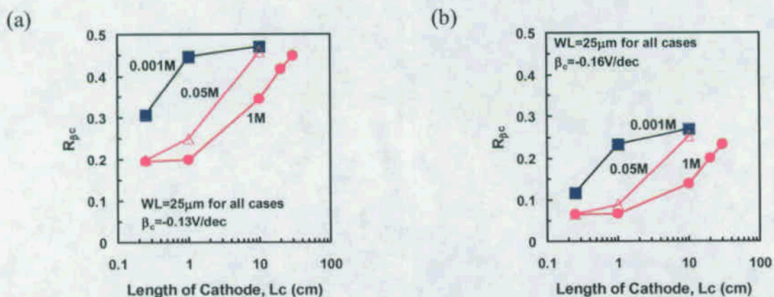
Figure 9. Effect of \beta_c , as described by R_{\beta_c} = I_{net}(\beta_c = 0.13 \text{ or } 0.16\text{V}) / I_{net}(\beta_c = 0.1\text{V}) : a) \beta_c = 0.13\text{ V/dec} ; b) \beta_c = 0.16\text{ V/dec} . Regardless of [\text{Cl}] , R_c tends to asymptote to \sim 0.45 ( \beta_c = 0.13\text{ V/dec} ) and \sim 0.25 ( \beta_c = 0.16\text{ V/dec} ) respectively at large L_c .
