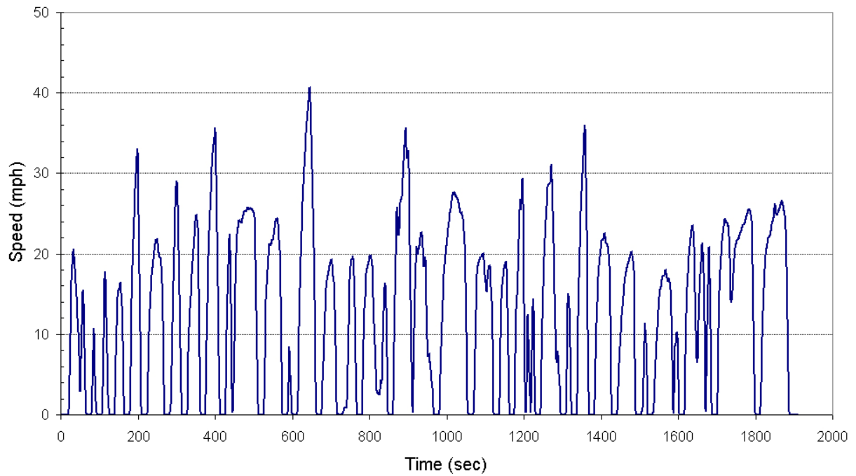
Figure 16. Orange County Test Cycle
