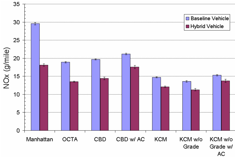
Figure 10. NO x emissions
