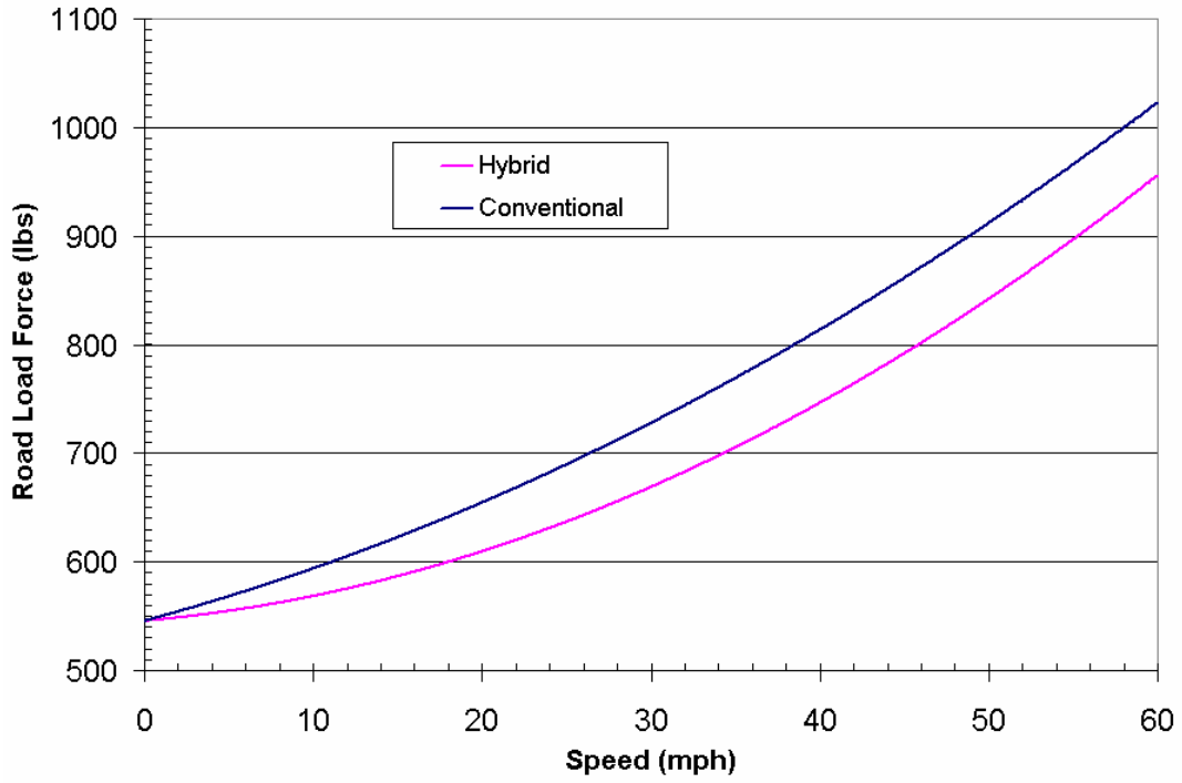
Figure 13. Road Load Curves
