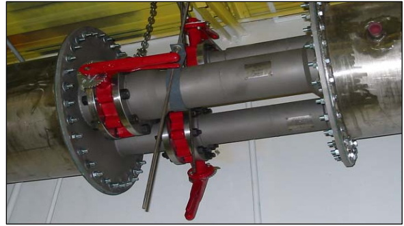
Figure 3. Venturi Nozzles
