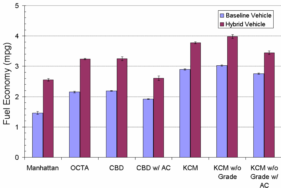
Figure 8. Average Fuel Economy
