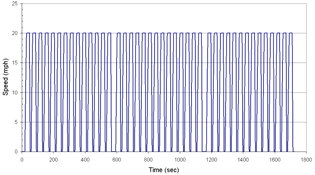
Figure 17. CBD x 3 Test Cycle
