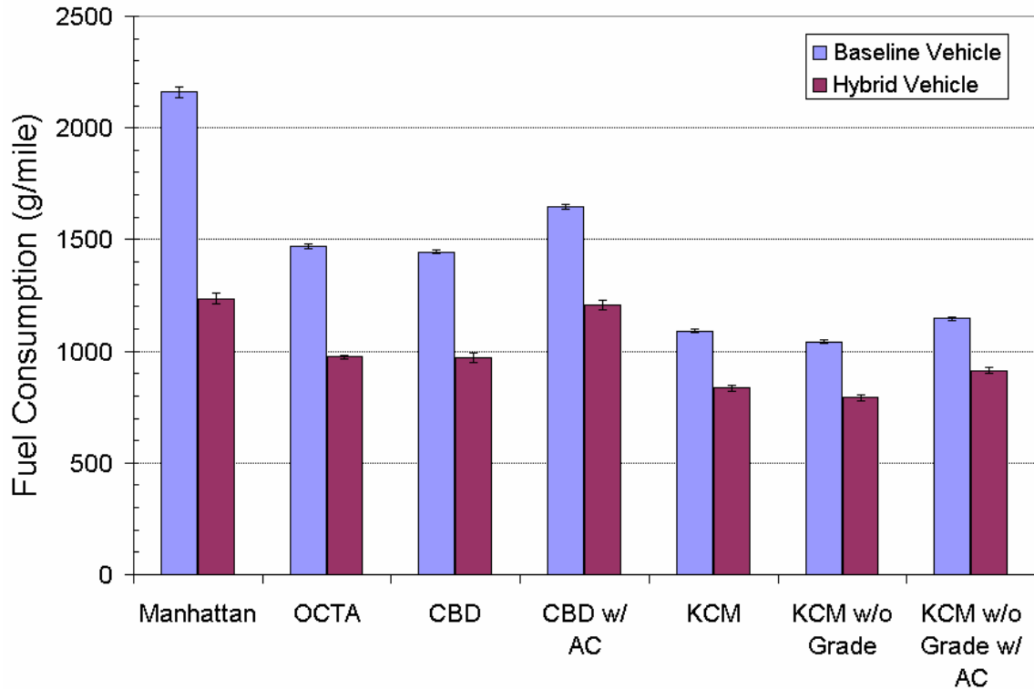
Figure 9. Average Fuel Consumption
