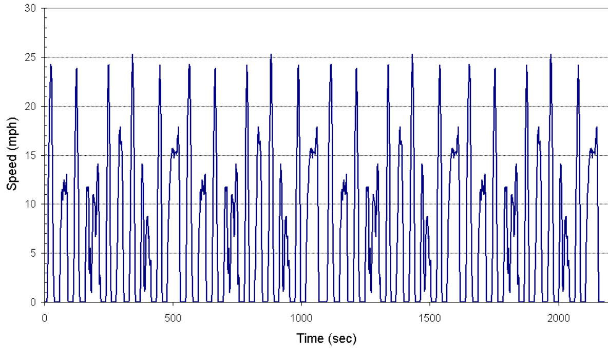
Figure 15. Manhattan x2 Test Cycle
