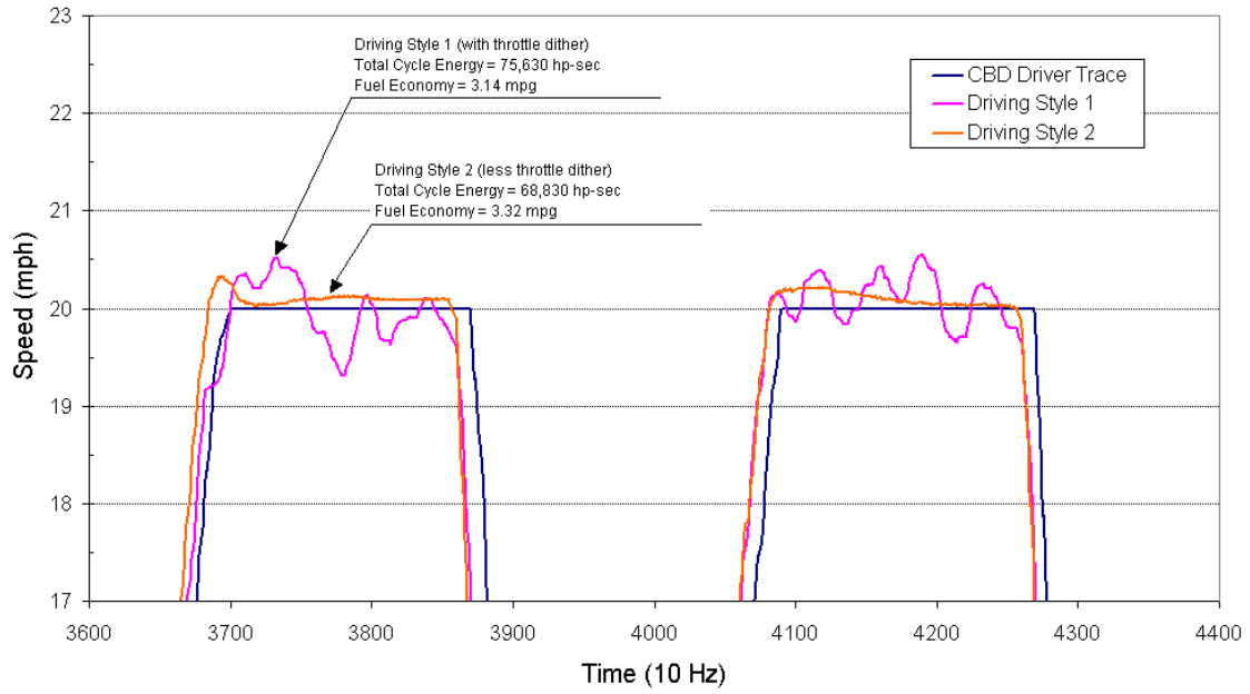
Figure 19. CBD Driving Styles
