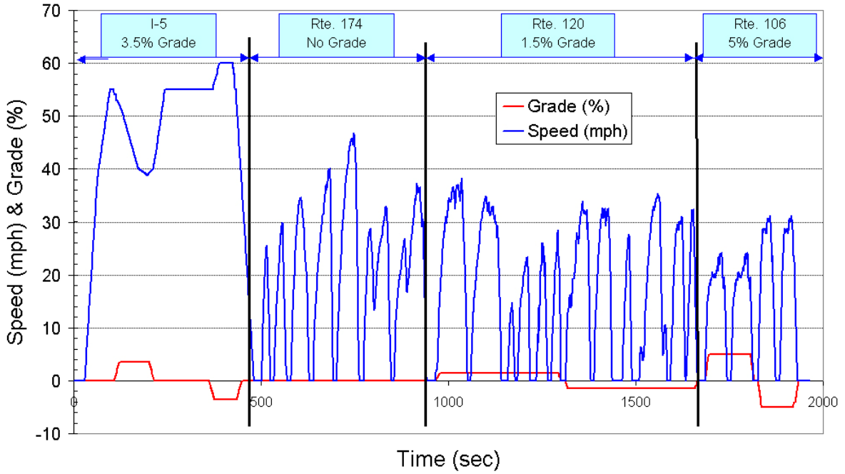
Figure 18. King County Metro Test Cycle
