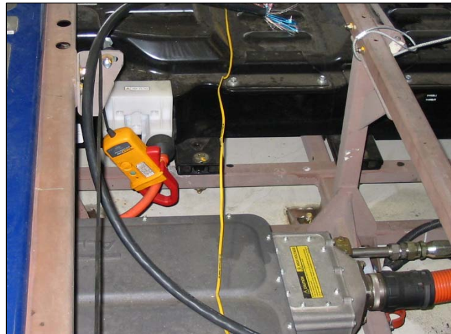
Figure 7. Current Clamp
