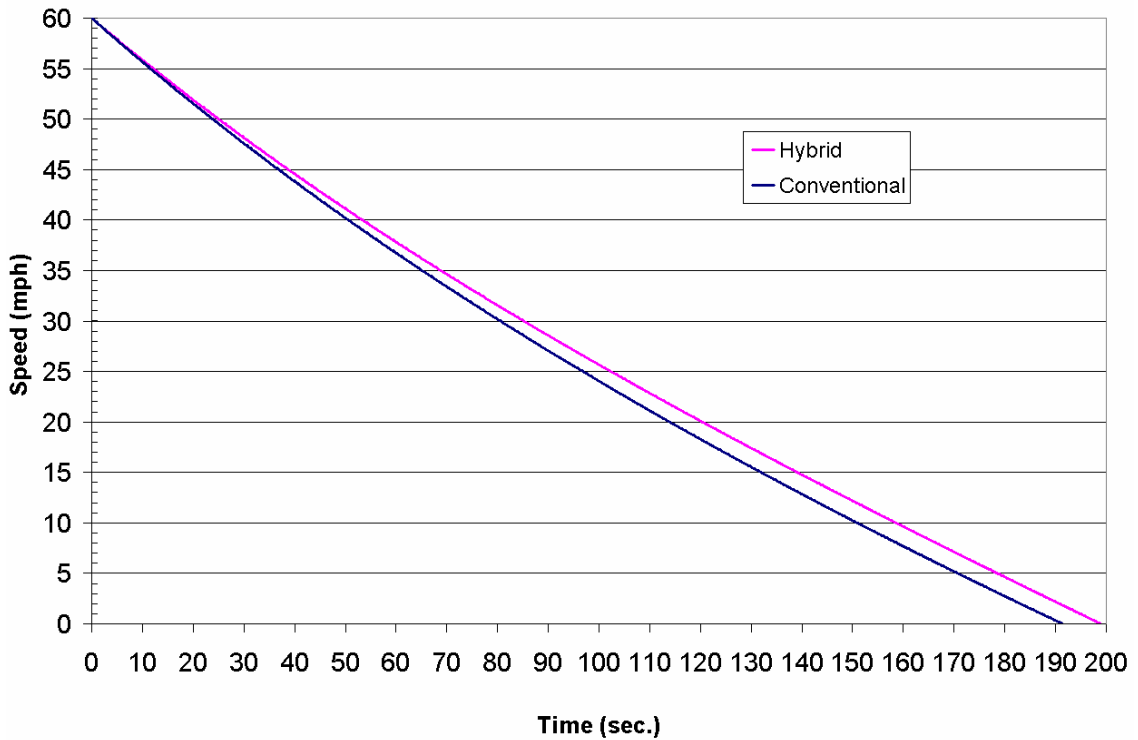
Figure 14. Coast Down Curves
