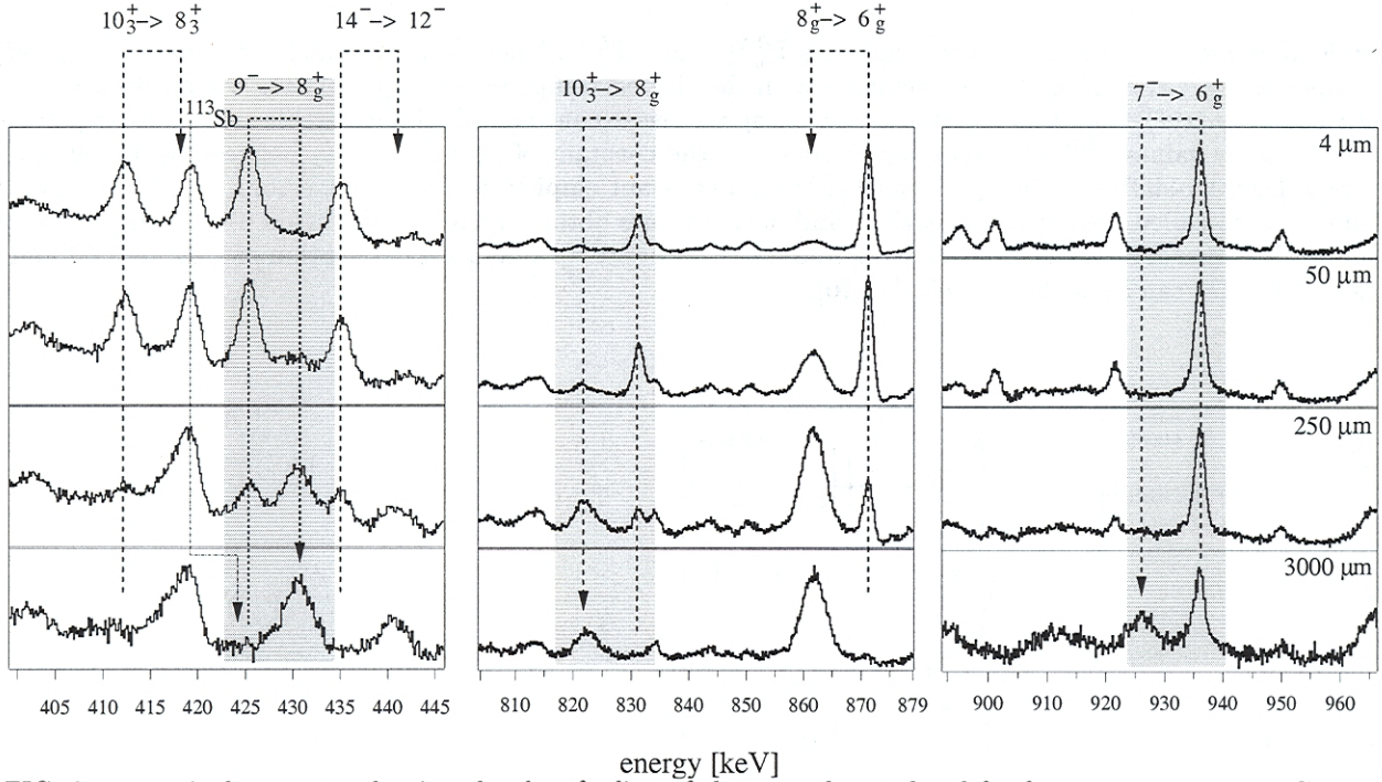
FIG. 6. \gamma -ray singles spectra showing the slow feeding of the ground-state band for four target-to-stopper distances. The spectra were obtained at 33^\circ (left panel) or 142^\circ (middle and right panels), respectively. The three main feeders of the gsb are shown against shadowed background, also indicated is a decay of a known isomer in ^{113}\text{Sb} ( \tau \approx 5 ns) at 419 keV and three other transitions in ^{114}\text{Te} . In order to draw attention to the relative shifts in intensity, no scale is given on the y-axis.
