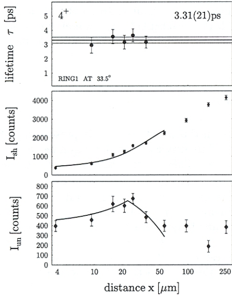
FIG. 8. Determination of the lifetime of the 4^+ state measured with detectors at 33.5^\circ .
