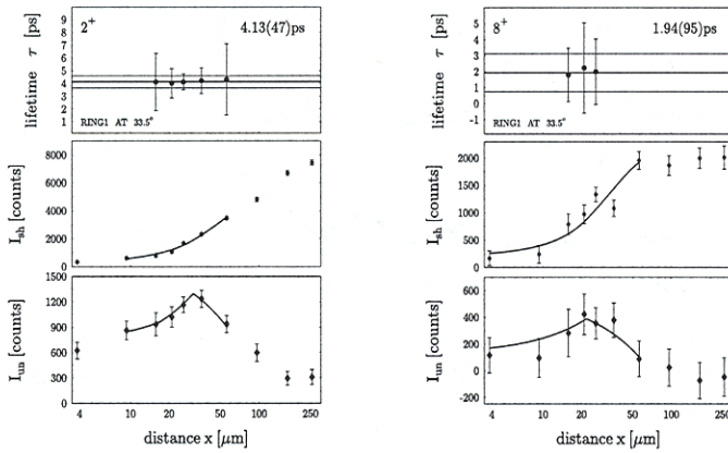
FIG. 4. Determination of the lifetime of the 2^+ (left panels) and 8^+ (right panels) states measured with the detectors at 33.5^\circ . The bottom frame displays the denominator in Eq. 1, while the numerator is displayed in the middle frame. The continuous curve in the bottom frame represents the fitted derivative of Doppler-shifted intensity (multiplied by the lifetime \tau ) as a function of the target-to-stopper distance.
