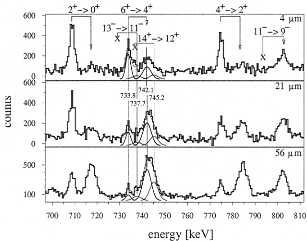
FIG. 1. Coincidence spectra resulting from gating on the 4^+ \rightarrow 2^+ shifted component observed in detector-ring 1. Indicated is the 2^+ \rightarrow 0^+ transition used to determine the 2^+ lifetime. In these spectra the shifted component lies higher in energy ( \theta_1 = 34^\circ ) than the unshifted component. The position labelled with the 'X' indicates where the unshifted component of a transition above the gating transition would be; it cannot be observed due to gating on the shifted component of a lower-lying transition.
