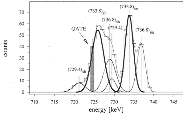
FIG. 7. Simulated spectrum of widths-calibrated Gaussians in the 740 keV region showing the 6_{gsb}^+ \rightarrow 4_{gsb}^+ transition, its contaminating peaks as well as their Doppler-shifted components, for a detector at the backward angle of 143^\circ . Since the gate on the shifted component is asymmetric relative to its centroid, recoils with higher velocities than the mean v/c are selected. This procedure makes it necessary to correct the lifetime resulting from spectra received from this gate.
