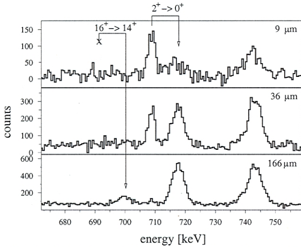
FIG. 1. Coincidence spectra resulting from gating on the 4^+ \rightarrow 2^+ shifted component observed in detector-ring 1. Indicated is the 2^+ \rightarrow 0^+ transition used to determine the 2^+ lifetime. In these spectra the shifted component lies higher in energy ( \theta_1 = 34^\circ ) than the unshifted component. The position labelled with the 'X' indicates where the unshifted component of a transition above the gating transition would be; it cannot be observed due to gating on the shifted component of a lower-lying transition.
