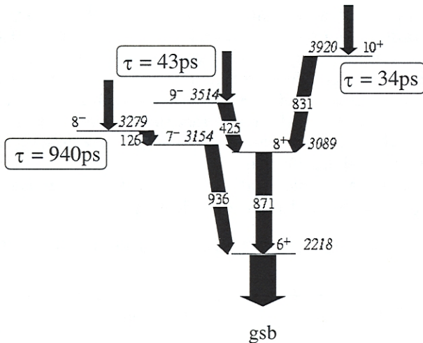
FIG. 5. Partial level scheme showing the main feeding transitions into the ground-state band (gsb) arise from isomeric levels.
